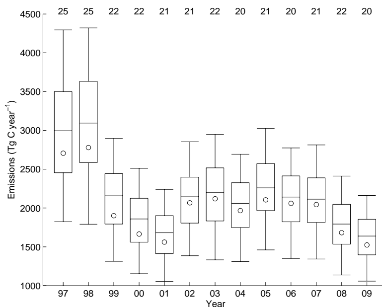
Fig. 14. Annual uncertainties expressed as the 5th, 25th, 50th, 75th, and 95th percentiles of 2000 runs in a Monte Carlo set-up. Circles denote the estimates reported throughout the paper, which do not necessarily align with the 50th percentiles due to truncation of several parameters in the Monte Carlo simulations. Numbers on the top of the plot indicate 1 \sigma uncertainties in annual fire emissions in percent of the median estimate from Monte Carlo simulations, assuming a Gaussian distribution. Note that uncertainties are larger on regional and monthly scales (Fig. S6).
