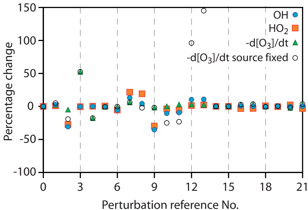
Fig. 7. Percentage change in modelled maximum OH (blue circles) and HO 2 (red squares) levels, and ozone loss rate (green triangles) for perturbations 1–21 (Table 3) of the model scheme, and change in ozone loss rate under the assumption of a fixed halogen source strength (open circles); see text for details.
