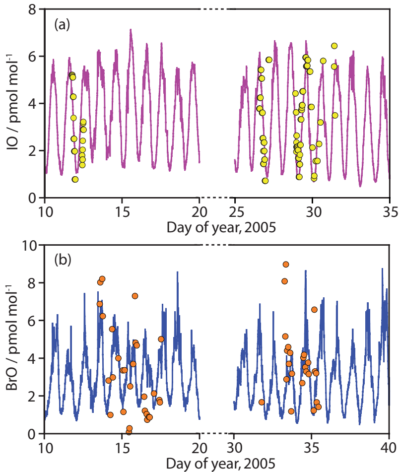
Fig. 1. (a) Observed and modelled IO and (b) Observed and modeled BrO mixing ratios as a function of day of year, 2005.
