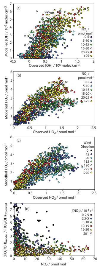
Fig. 3. (a) Modelled vs. observed OH, coloured as f(\text{NO}_x) ; (b) Modelled vs. observed \text{HO}_2 , coloured as f(\text{NO}_x) ; (c) Modelled vs. observed \text{HO}_2 coloured by wind direction (legend denotes centre of 45^\circ sector, expressed in degrees from North) and (d) ratio of modelled to observed \text{HO}_2 :OH ratio as a function of \text{NO}_2 , coloured according to j(\text{NO}_2) .
