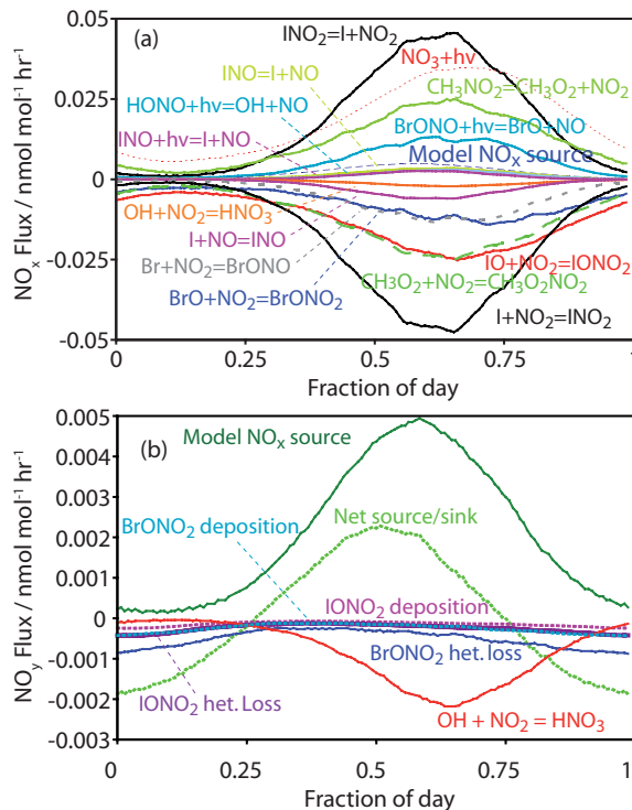
Fig. 5. Diurnal variation in modelled production and loss for (a) \text{NO}_x and (b) \text{NO}_y . Panel (a), major source and sink processes for \text{NO}_x (here defined strictly as \text{NO}_x = \text{NO} + \text{NO}_2 only) for model case B2. The \text{NO}_3 contribution (red dashed line) arises here from photolysis of \text{INO}_3 and \text{BrNO}_3 , offsetting their sink role, rather than \text{NO}_2 + \text{O}_3 reactions. Panel (b), major source and sink contributions to \text{NO}_y calculated for model scenario B2, plus net \text{NO}_y production/removal (dashed line). \text{NO}_y defined as \text{NO}_y = \text{NO} + \text{NO}_2 + \text{NO}_3 + 2\text{N}_2\text{O}_5 + \text{HONO} + \text{PNA} + \text{CH}_3\text{NO}_3 + \text{CH}_3\text{O}_2\text{NO}_2 + \text{XNO} + \text{XNO}_2 + \text{XNO}_3 .
