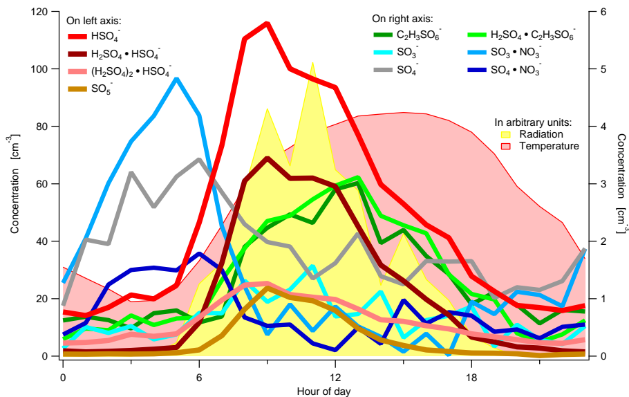
Fig. 7. Diurnal trends for selected sulfuric acid related negative ions.
