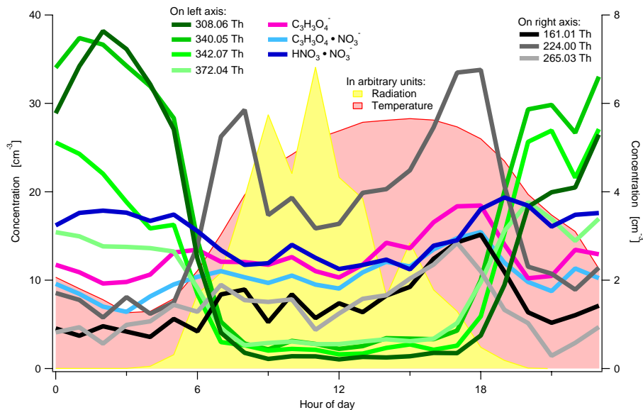
Fig. 8. Diurnal trends for selected organic and nitric acid negative ions.
