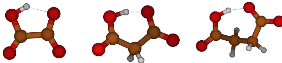
Fig. A1. Minimum-energy structures (at the CBS-QB3 level) of hydrogenoxalate (left), hydrogenmalonate (center) and hydrogensuccinate (right) ions. Color coding: red = oxygen, brown = carbon, white = hydrogen.
