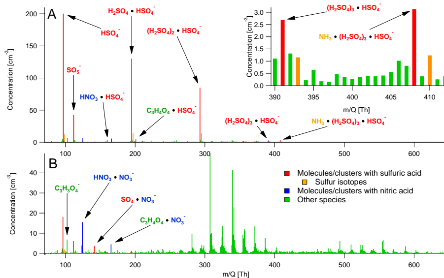
Fig. 1. Negative ion mass spectra during the measurements in Hyytiälä, averaged over 3 h. (A) shows a typical daytime spectrum and (B) a typical nighttime spectrum. The ions are colored based on the identified composition.
