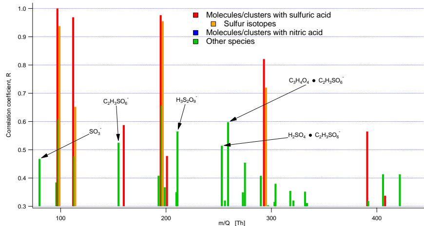
Fig. 3. Correlogram showing time-series correlation of ions with \text{HSO}_4^- . The dimer, trimer and tetramer all stand out, together with some other peaks tagged in Fig. 1. Ions with typically lower concentration but high correlation are marked in the figure. The \text{C}_2\text{H}_3\text{SO}_6^- ion may be the first observation of an organosulfate in the gas phase. For reference, the coloring is kept the same as in Fig. 1 although additional peaks were found to contain sulfuric acid.
