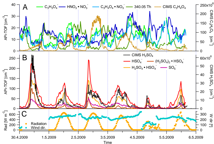
Fig. 6. Time trends of selected negative ions in Hyttiälä measured by the API-TOF, with sulfate – related ions in the middle panel and nitric acid and organics in the top panel. Also included in these are CIMS measurements of sulfuric and malonic acid (dotted lines). In the bottom panel radiation and wind direction are included (data for 30 April is missing).
