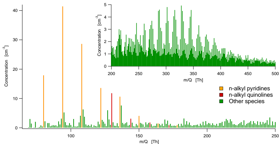
Fig. 2. Typical daytime positive ion mass spectrum during the measurements in Hyytiälä, averaged over 3 h.
