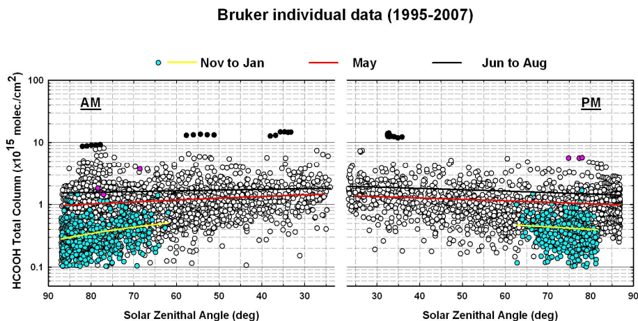
Fig. 4. Illustration of the diurnal variation of HCOOH above the Jungfrauoch, based on the individual Bruker FTIR observations between 1995 and 2007, with overall AM increases and PM decreases evaluated separately. First order fittings to all N-D-J data (filled cyan points) are highlighted by the two yellow lines. The black and red lines correspond to similar fittings, respectively to all J-J-A and May observations. Related AM increases and PM decreases are given in Table 3. The extreme high HCOOH columns observed on 15 August 1995 and on 14 January 2007 (respectively 25 black- and 7 pink filled circles) were excluded from the fittings.
