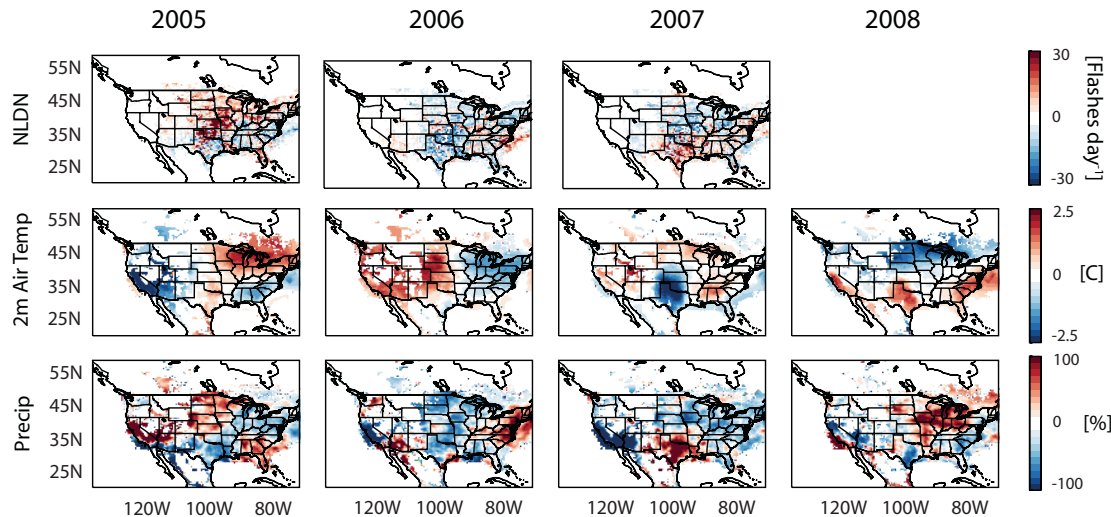
Fig. 3b. Same as Fig. 3a except for flash counts from the National Lightning Detection Network (NLDN) (mean daily flashes), Temperature (C), Precipitation (%). NLDN flashes are X3 higher in 2008 than 2005–2007 for reasons that are unclear as such we take the anomaly from 2005–2007 mean.
