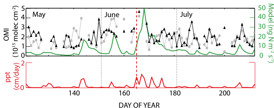
Fig. 5. May–July 2006 timeseries of soil NO pulsing events over rural South Dakota (43–45° N, 98.75–96.25° W). OMI NO 2 column densities (top) for the Standard Product (black triangles) and DOMINO Product (grey circles) are compared with predicted soil NO emissions (top, green) and precipitation (bottom, red).
