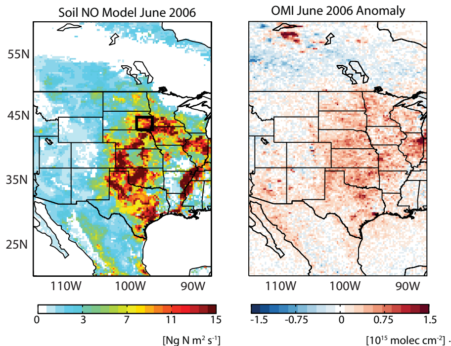
Fig. 4. June 2006 modeled Soil NO x emissions are compared to OMI tropospheric column NO 2 anomalies over the Central United States. Anomaly calculated as in Fig. 3a. Boxed region (43–45° N, 98.75–96.25° W) shown is used in case-study in Sect. 5 of text.
