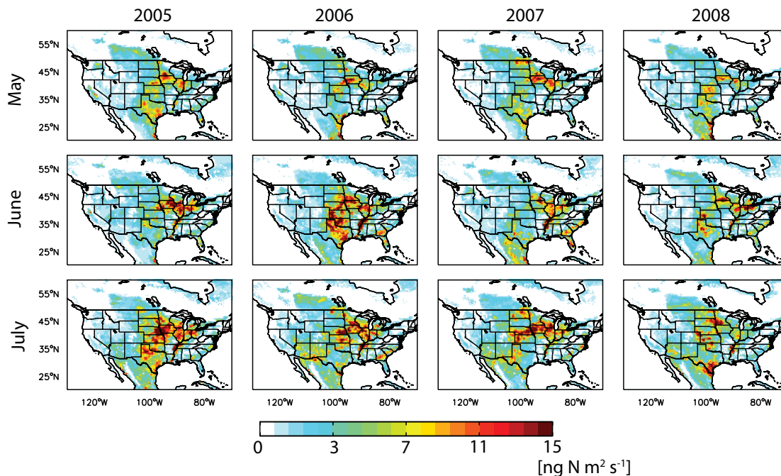
Fig. 1. Simulated monthly mean soil NO x emissions for 2005–2008 at 0.25^\circ \times 0.25^\circ resolution. Emissions were derived using Yienger and Levy (1995) algorithm, with modifications as described in the text. The model is driven by daily precipitation and soil temperature from the North American Regional Reanalysis, NASA TERRA/MODIS HDF-EOS MOD12Q1 V004 land cover data, and fertilizer totals from Potter et al. (2009) with seasonality from Goebes et al. (2003) regridded to model resolution.
