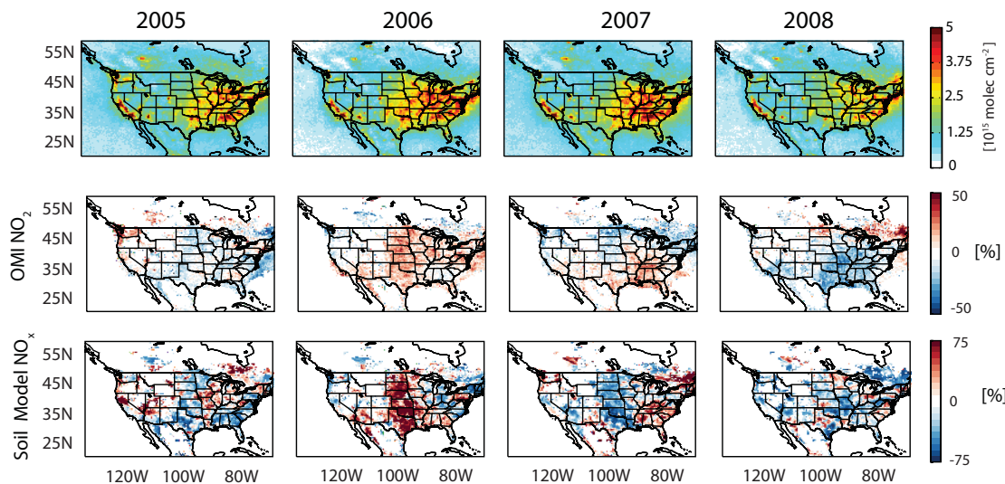
Fig. 3a. June mean OMI NO 2 column densities (top) are compared to mean anomalies for OMI NO 2 (middle) and Soil Model NO x emission (bottom), calculated as difference with June 2005–2008 mean. Only regions with mean June OMI NO 2 column > 1.25 \times 10^{15} molec cm -2 are shown in anomaly plots. Color bar saturated at high and low end.
