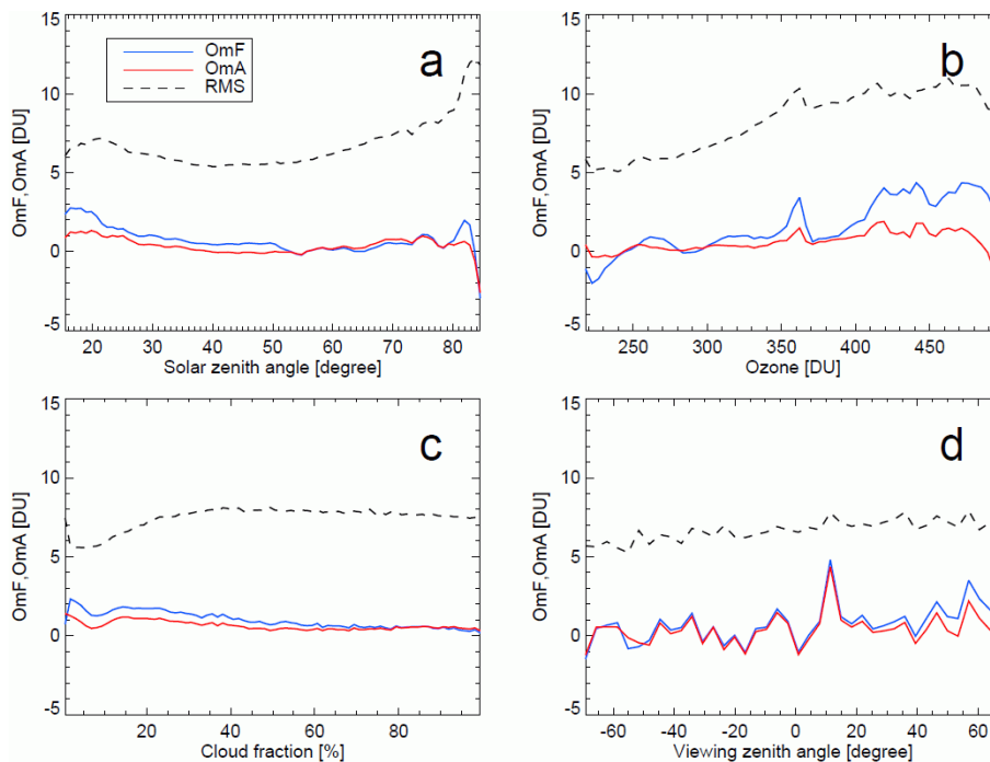
Fig. 8. The observation-minus-forecast in DU (blue line) and the observation-minus-analysis (red line) as a function of solar zenith angle ( a ), observed ozone ( b ), cloud fraction ( c ), and viewing zenith angle ( d ). The dashed line represents the RMS value of the observation-minus-forecast distribution. All data are averaged over January 2008.
