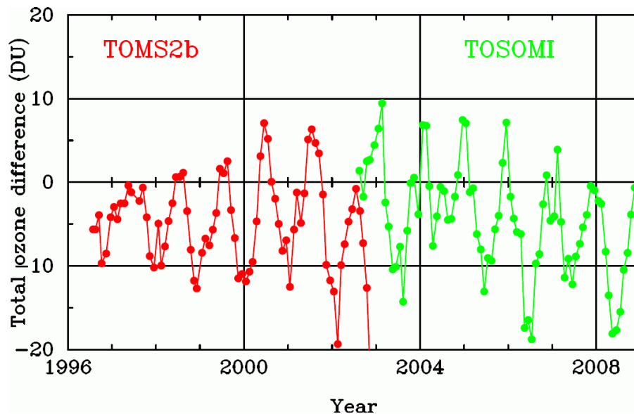
Fig. 1. Monthly averaged anomalies for the overpass data at the ground station De Bilt (5.18° E, 52.1° N) in the Netherlands. The anomalies for TOMS2b (red) correlate with stratospheric temperature, while the anomalies for TOSOMI (green) correlate with Solar zenith angle.
