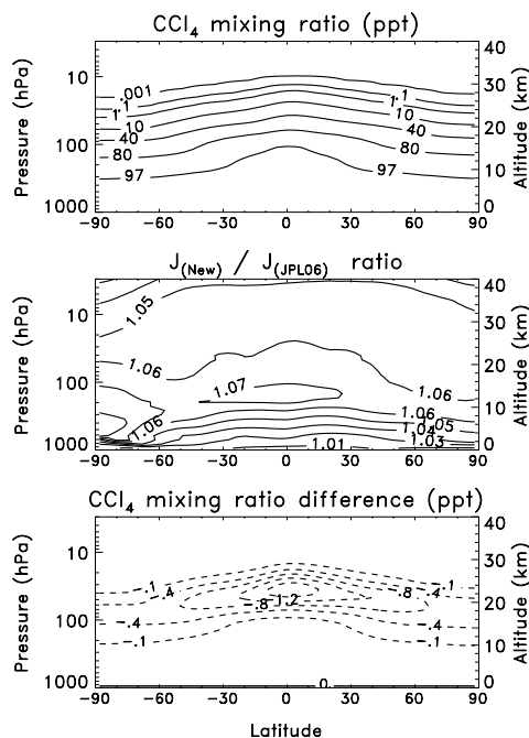
Fig. 5. (Top) Modeled distribution of CCl 4 mixing ratio (ppt); (middle) ratio of the photolysis loss of CCl 4 using UV absorption cross sections obtained in this work to that using absorption cross sections from JPL06-2 (Sander et al., 2006); (bottom) modeled CCl 4 mixing ratio difference (ppt) using absorption cross sections obtained in this work and that using absorption cross sections from JPL06-2. All values are annual averages for year 2000. The contours plotted in the bottom panel are -1 , -4 , -8 , -1.2 , and -1.6 ppt.
