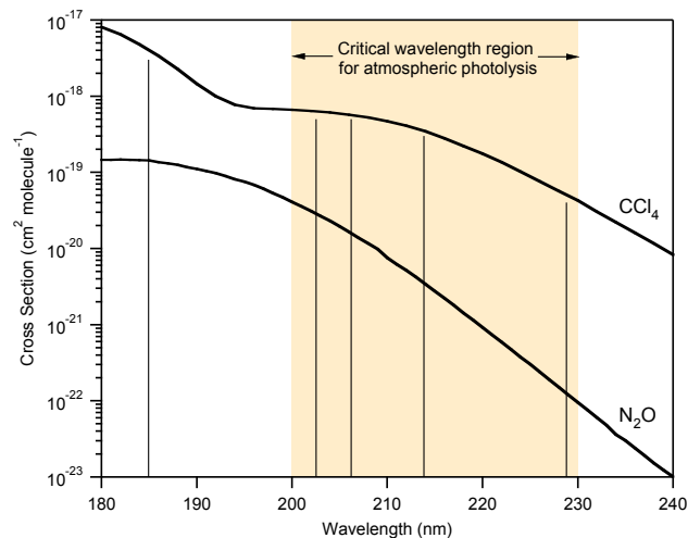
Fig. 1. The JPL06-2 (Sander et al., 2006) recommended UV absorption cross section spectra of N 2 O and CCl 4 at 298 K. The shaded area highlights the wavelength region most important for atmospheric photolysis. The vertical lines correspond to the wavelengths of the atomic lines used in this work.
