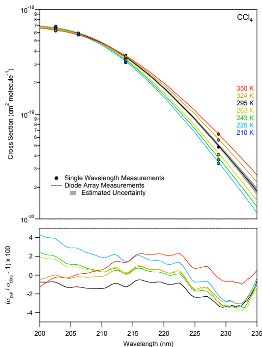
Fig. 4. Absorption spectra of CCl 4 obtained using a diode array spectrometer (solid lines) at temperatures given in the legend. The shaded region represents the estimated absolute 2\sigma (95% confidence level) uncertainty at 295 K including estimated systematic errors. Also included for comparison are the absorption cross sections obtained from the single wavelength measurements in this work (•). The deviation of the measured spectra from the cross section parameterization given in Table 3 is given in the lower frame.
