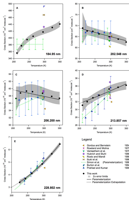
Fig. 3. Temperature dependent CCl 4 absorption cross sections obtained in this work (●). The shaded region represents the estimated absolute 2σ (95% confidence level) uncertainty from our work including estimated systematic errors. Included for comparison are results from previous studies as indicated in the legend. The data from Simon et al. (1988), the data set currently recommended by JPL06-2 (Sander et al., 2006) for use in atmospheric modeling, are plotted using the cross section and temperature dependence parameterization reported in their work. Data from Causley and Russell (1977), Seccombe et al. (1999), Ho (1998), and Roxlo and Mandl (1980) are not included due to the large deviation from the other studies.
