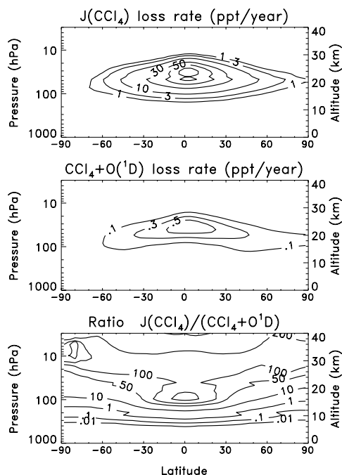
Fig. 6. (Top) Modeled photochemical loss rate of CCl 4 due to photolysis (in parts per trillion per year) using the UV absorption cross sections obtained in this work. Also shown are the CCl 4 loss rate due to reaction with O( 1 D) (middle), and the ratio of the photolysis loss to the O( 1 D) loss (bottom). All values are annual averages for year 2000. The contours plotted in the top panel are 1, 3, 10, 30, 50, and 70 ppt/year.
