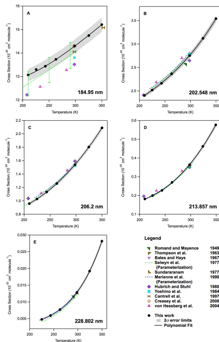
Fig. 2. Temperature dependent N 2 O absorption cross sections obtained in this work (●). The shaded region represents the estimated absolute 2σ (95% confidence level) uncertainty from our work including estimated systematic errors. Included for comparison are results from previous studies as indicated in the legend. The data from Merienne et al. (1990) and Selwyn et al. (1977) are plotted using the cross section and temperature dependence parameterizations reported in their work. Data from Zelikoff et al. (1953) are not included due to their large deviation from the other studies. The results from Selwyn et al. (1977) supercedes the results from Johnston and Selwyn (1975), which are not shown.
