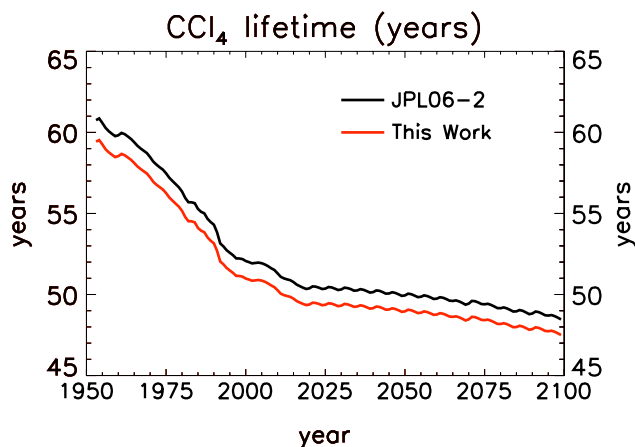
Fig. 7. Time series for 1950–2100 of the modeled photochemical lifetime of CCl 4 (years) using the UV absorption cross sections obtained in this work (red), and absorption cross sections from JPL06-2 (Sander et al., 2006) (black). Note that the calculation of lifetime does not include any surface land or ocean loss of CCl 4 .
