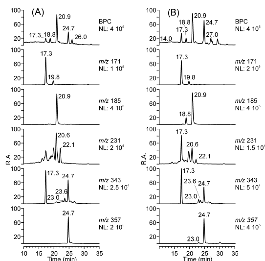
Fig. 1. LC/MS chromatographic data [base peak chromatograms (BPCs) and extracted ion chromatograms (EICs)] for (A) \alpha -pinene and (B) \beta -pinene ozonolysis SOA. Abbreviation: NL, normalization level.
