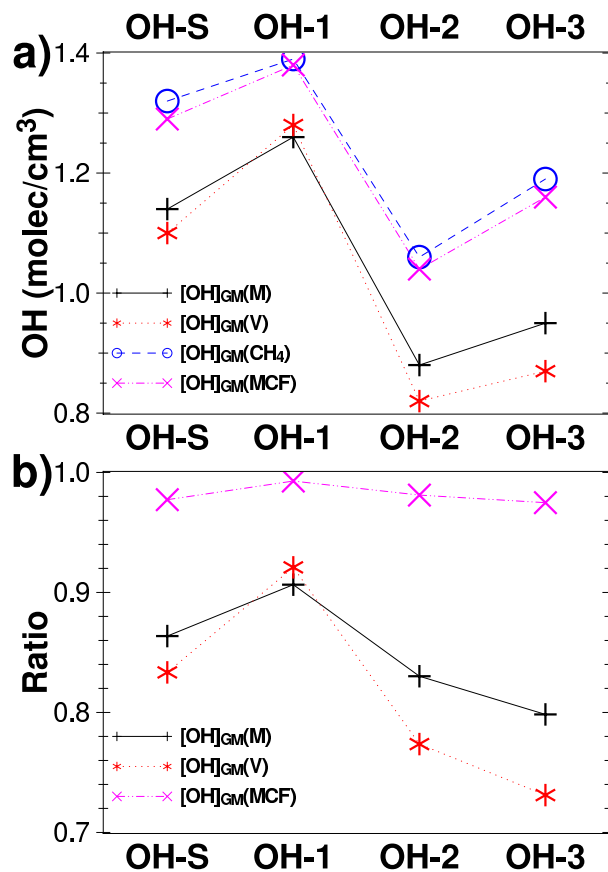
Fig. 2. Depictions of the relationships between different ways of computing the tropospheric [\text{OH}]_{GM} : (a) [\text{OH}]_{GM} values for the four distributions and four weightings discussed in the text; (b) ratio of [\text{OH}]_{GM} values for three weightings versus [\text{OH}]_{GM}(\text{CH}_4) .
