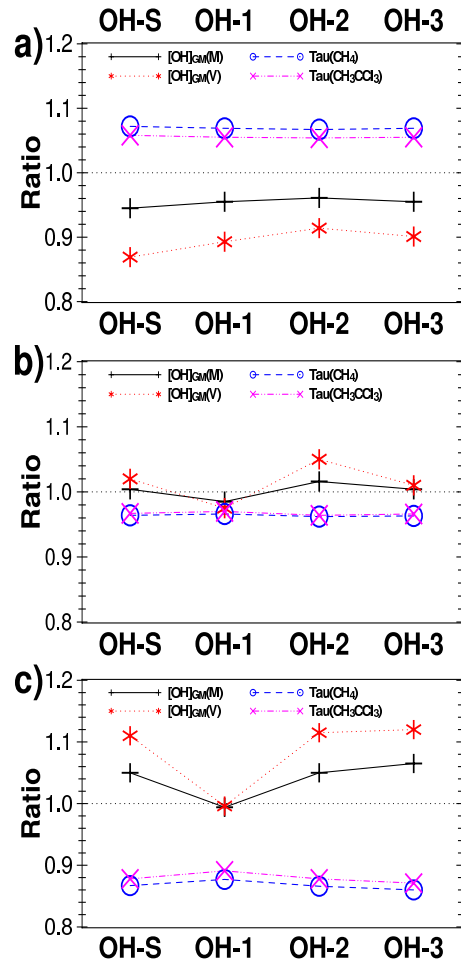
Fig. 3. The ratios of [OH]_{GM}(M) , [OH]_{GM}(V) , \tau(CH_4) , and \tau(CH_3CCl_3) for (a) the domain below 100 hPa, (b) the domain below 200 hPa, and (c) the domain below 300 hPa, versus the values for the climatological troposphere (Eq. 6).
