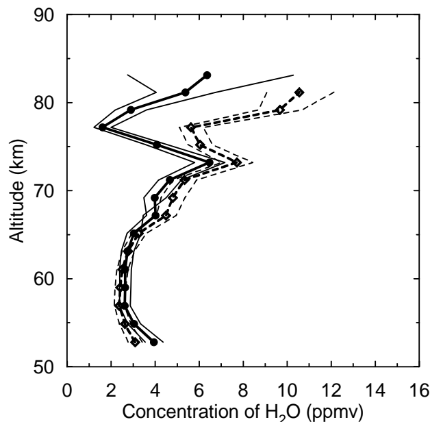
Fig. 5. Profiles of \text{H}_2\text{O} concentration retrieved from CRISTA-MAHRSI data measured on 15 August 1997 at 69\text{--}71^\circ\text{N} , 60\text{--}65^\circ\text{W} (heavy solid curve and dark circles) and 66\text{--}68^\circ\text{N} , 141\text{--}148^\circ\text{W} (heavy dashed curve and open rhombs). The thin curves show retrieval error corresponding to uncertainties of initial experimental data.
