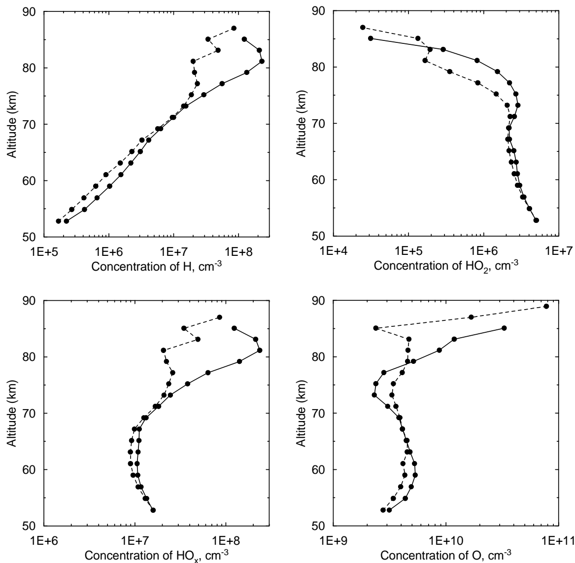
Fig. 3. Vertical distributions of H, HO 2 , HO x and O concentration at the instants of local time about 08:00 a.m. (dashed curve) and 03:00 p.m. (solid curve) retrieved from CRISTA-MAHRSI data measured on 13 August 1997 at 60–63° N, 355–360° W.
