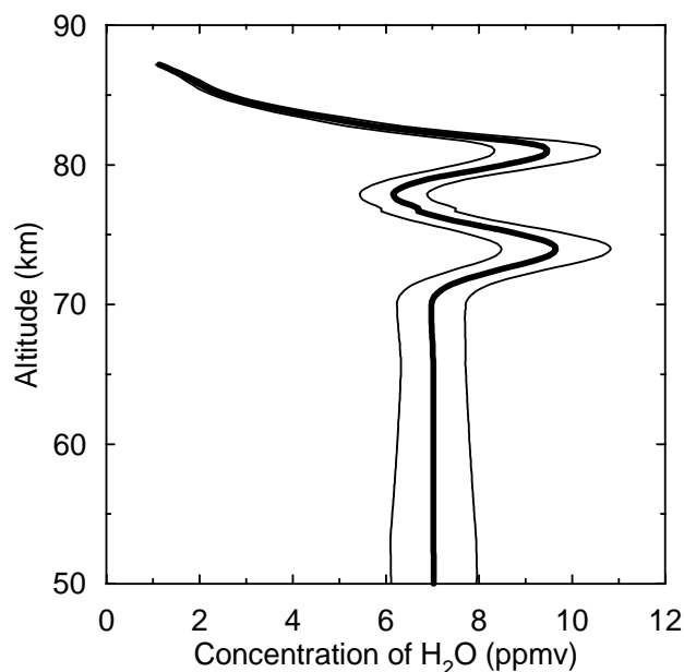
Fig. 2. The same as in Fig. 1 (violet curves), but with allowance for 5% uncertainty of initial data. The thin lines show uncertainty boundaries of retrieved values of \text{H}_2\text{O} concentration.
