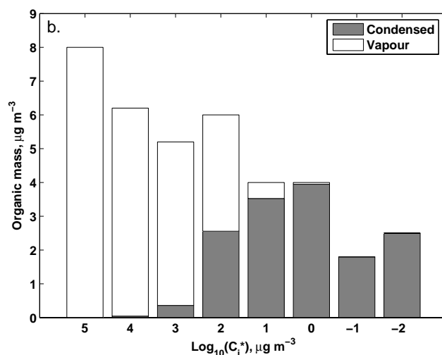
Fig. 3b. Same as panel (a) but for moist air (RH=80%), total condensed mass= 74.22 \mu\text{g m}^{-3} , of which organic condensed mass= 14.74 \mu\text{g m}^{-3} .
