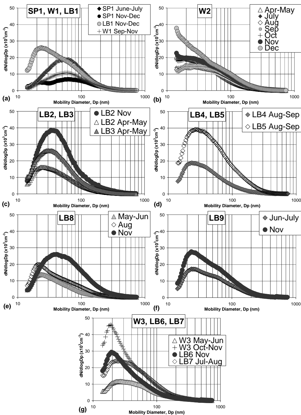
Fig. 2. Average number-based particle size distributions measured during each sampling period at each site.
