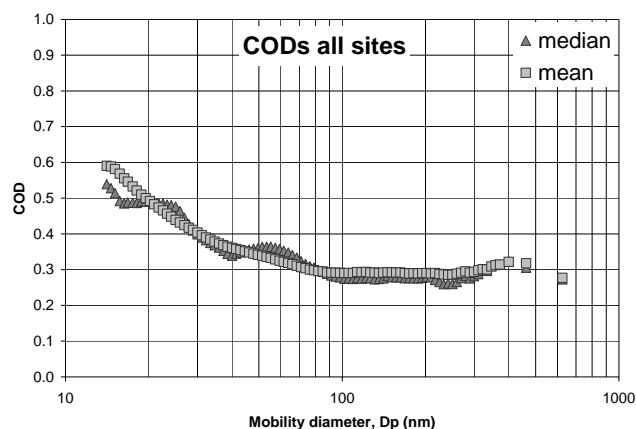
Fig. 5. Median and mean CODs across all sites and sampling periods.
