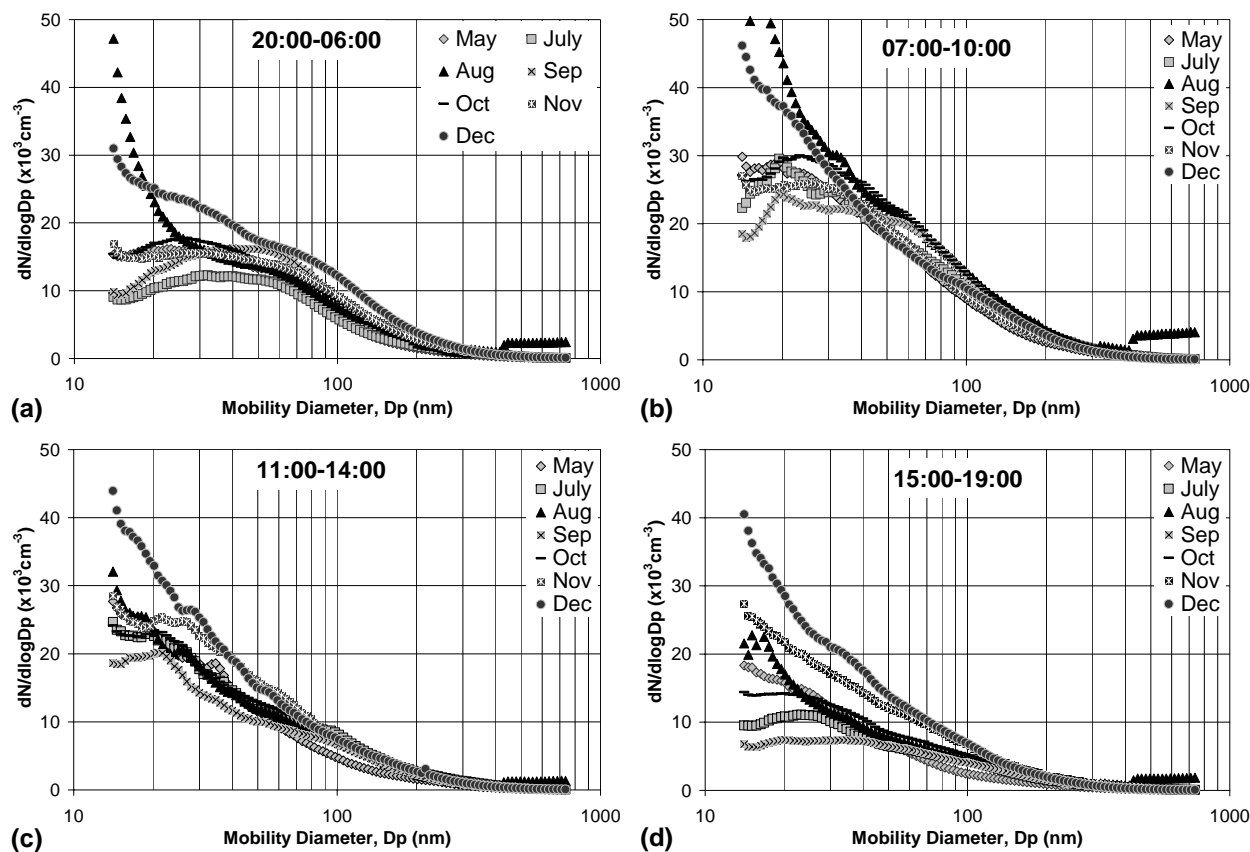
Fig. 3. Diurnal and seasonal patterns in number size distributions at site W2 during: (a) nighttime (20:00–06:00), (b) morning commute (07:00–10:00), (c) midday (11:00–14:00), and (d) evening commute (15:00–19:00). All times are Pacific Standard Time (PST).
