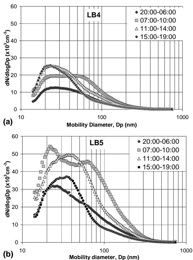
Fig. 4. Diurnal patterns in number size distributions at sites: (a) LB4 and (b) LB5.
