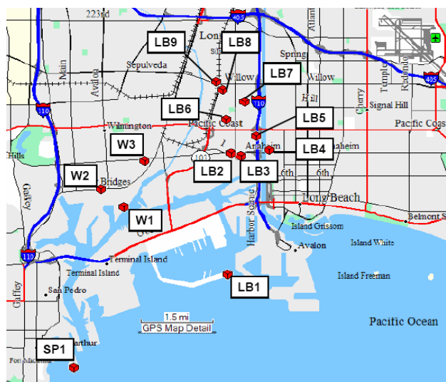
Fig. 1. SMPS sampling sites (latitude and longitude coordinates provided in Moore et al., 2009).
