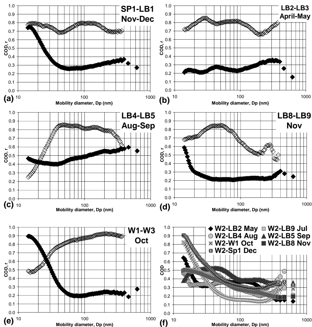
Fig. 6. CODs and correlations coefficients for selected site pairs. (a) SP1–LB1 in November–December, (b) LB2–LB3 in April–May, (c) LB4–LB5 in August–September, (d) LB8–LB9 in November, (e) W1–W3 in October, and (f) LB2 with selected sites (assorted months). Closed and open symbols indicated COD and r values, respectively.
