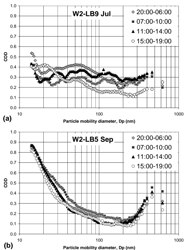
Fig. 7. Diurnal patterns in CODs for selected site pairs (a) LB2 and LB9 in July, and (b) LB2 and LB5 in September.
