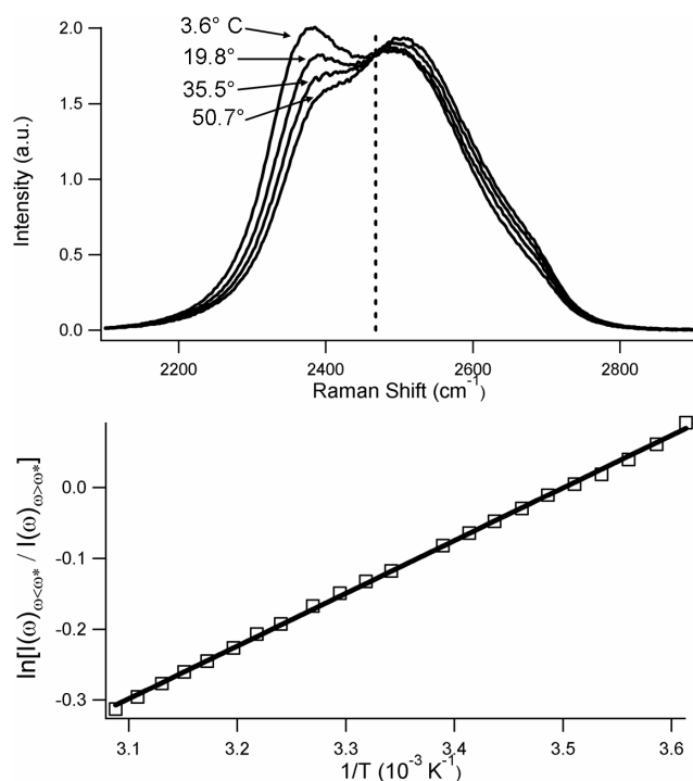
Fig. 2. (a) Representative spectra used to generate one of the temperature calibration curves. The dashed line shows the frequency \omega^* = 2468 \text{ cm}^{-1} where the spectra were split. The full curve is constructed from spectra of liquid D 2 O at 22 different temperatures between 3.6°C and 50.7°C. (b) Representative temperature calibration curve. R^2 = 0.9992 .
