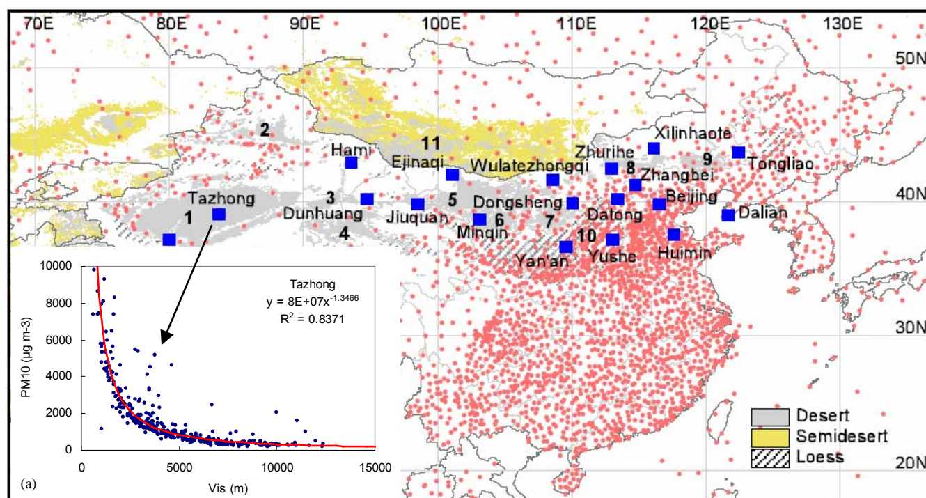
Fig. 4. SDS observation stations by the CMA. The red dots are meteorological stations with visual visibility measurements and the blue squares are SDS observation stations with PM 10 and instrumental visibility measurements. Insert: Relationship between hourly-averaged PM 10 concentration and visibility during SDS events in the springtime at Tazhong station.
