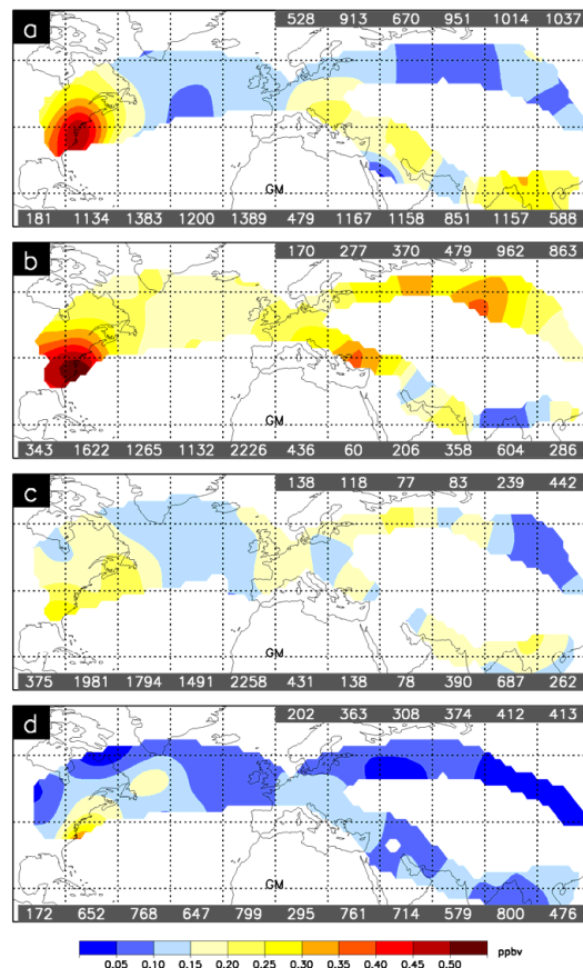
Fig. 5. Distribution of NO x (in ppbv or nmol/mol) in the 330–220 hPa altitude range in the four seasons ((a): MAM, (b): JJA, (c): SON, (d): DJF). Numbers denote the sample sizes along the routes (Brunner, 1998).
