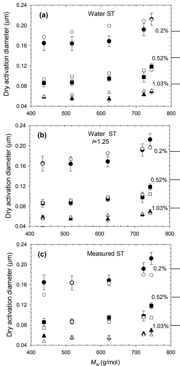
Fig. 6. The measured (solid symbols) and calculated (hollow symbols) dry diameters needed for particle activation for the size-fractionated SRFA samples. Circles, squares and triangles indicate the activation diameters at supersaturations 0.2, 0.52 and 1.03%, respectively. The correlation of Schafer et al. (2002) is used in estimating M_n . The particle surface tension is assumed to be either that of water ( a and b ) or taken from the measurements ( c ). The Van't Hoff factor is set equal to unity (a and c) or to 1.25 (b).
