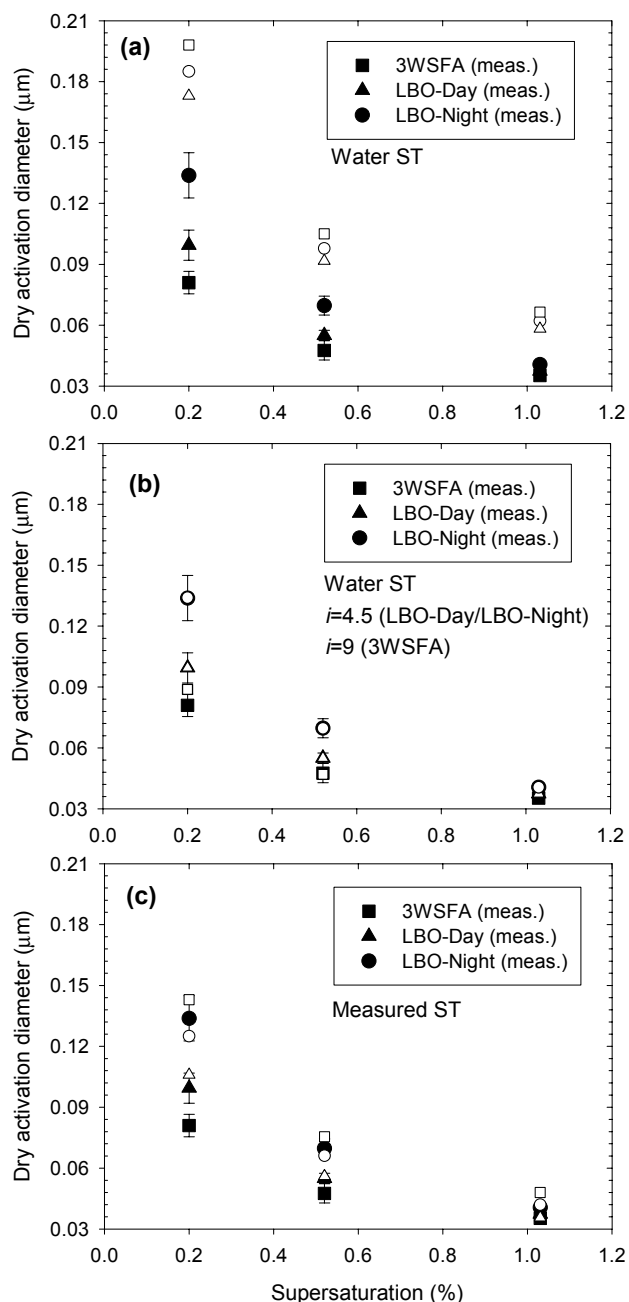
Fig. 7. The measured (solid symbols) and calculated (hollow symbols) dry diameters needed for particle activation for the extracted FA HULIS samples. The correlation of Schafer et al. (2002) is used in estimating M_n . The particle surface tension is assumed to be either that of water (a and b) or taken from the measurements (c). The Van't Hoff factor is set equal to unity (a and c) or varied (b). It is found that i=4.5 can account for the LBO samples, and i=9 can account for the behavior of the 3WSFA sample.
