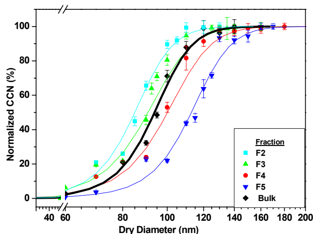
Fig. 3. An example for activation curves for all SRFA fractions at SS=0.52\% . The bulk sample (black line) lies between the 1–3 kDa to the 3–10 kDa. This behavior is repeatable in all SS measured for these samples. A clear correlation between the mass and activation diameter exists. The error bars represent the standard deviation for each point of 6–14 experiments, conducted on different days.
