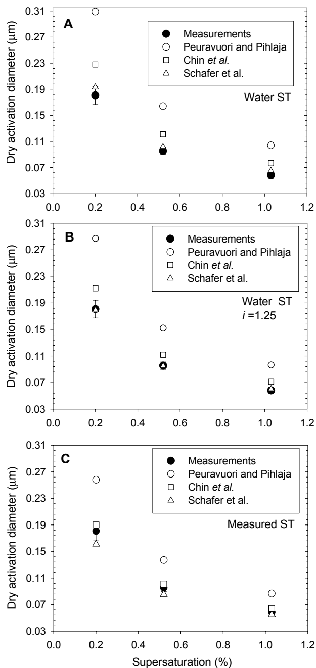
Fig. 5. The measured (solid symbols) and calculated (hollow symbols) dry diameters needed for particle activation for the bulk SRFA sample. The correlation used in estimating M_n is displayed in the legend. The particle surface tension is assumed to be either that of water ( a and b ) or taken from the measurements ( c ). The Van't Hoff factor is set equal to unity (a and c) or to 1.25 (b).
