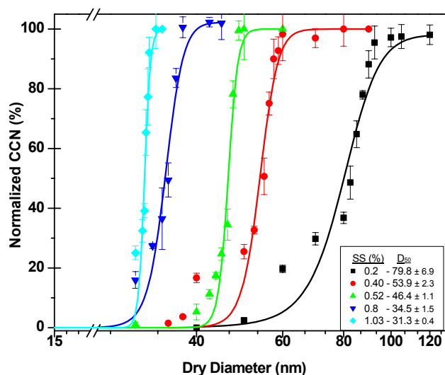
Fig. 2. Activation curves of ammonium sulfate particles. The activation diameter ( D_{50} ) is indicated in the legend for all SS measured. The error bars represent the standard deviation for each point of 6–14 experiments, conducted on different days.
