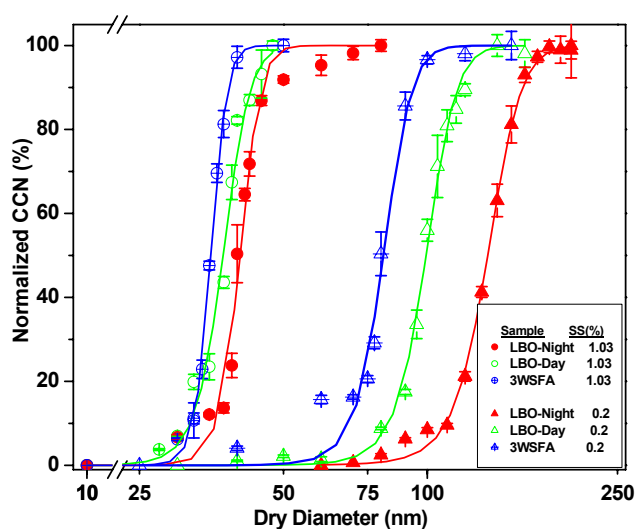
Fig. 4. Activation experiments with extracted FA HULIS under SS conditions of 0.2 and 1.03%. Experiments were carried out by atomizing solution of FA extracted from collected smoke particles. Refer to the text for explanation of the samples. Activation experiments under SS of 0.52% exhibit same behavior (see Table 5).
