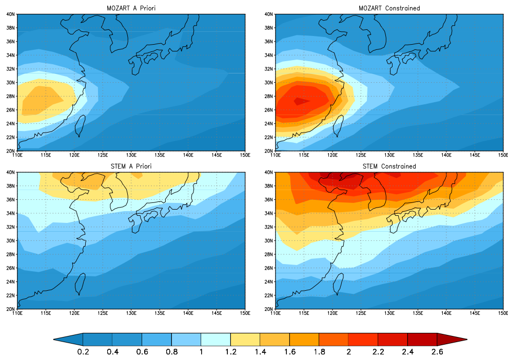
Fig. 20. NWP AOD at 0.55\ \mu\text{m} with MOZART aerosols (top panel) and STEM aerosols (bottom panel). First column is with the “a priori” aerosol optical properties; second column is with the constrained optical properties.
