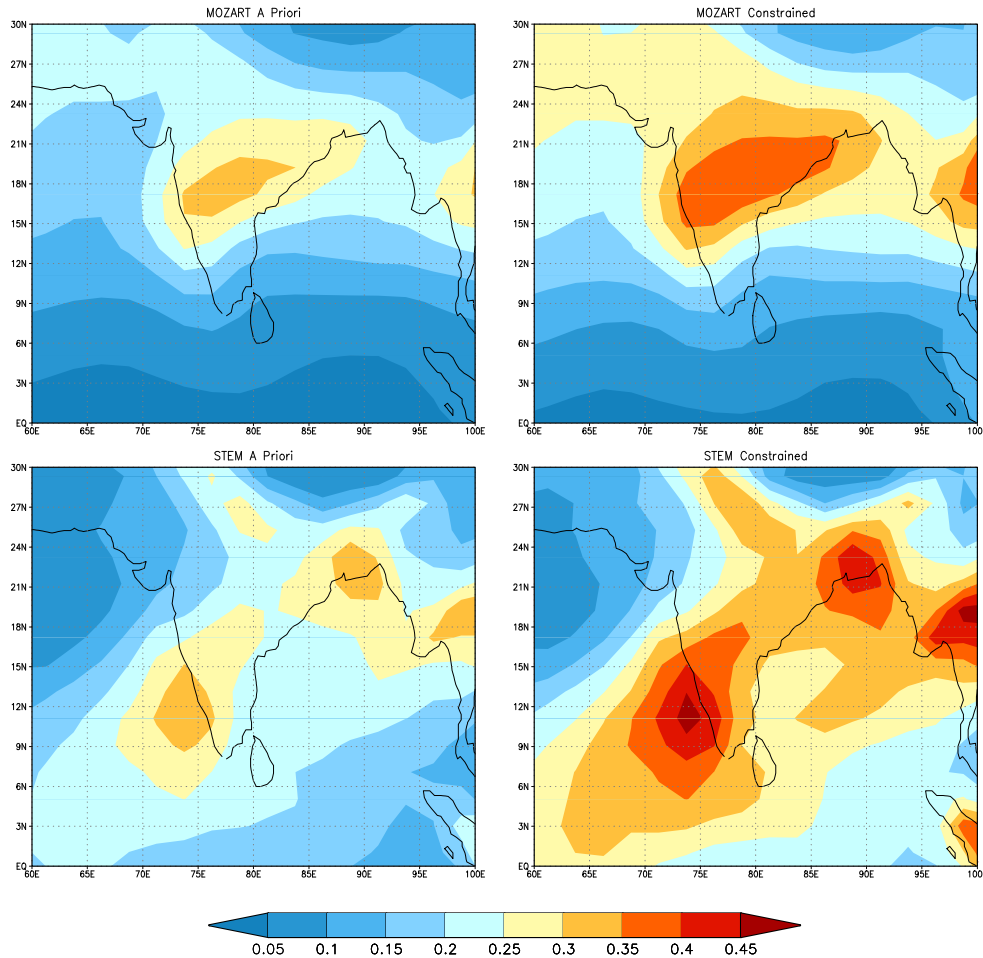
Fig. 18. NIO AOD at 0.55 \mu\text{m} with MOZART aerosols (top panel) and STEM aerosols (bottom panel). First column is with the “a priori” aerosol optical properties; second column is with the constrained optical properties.
