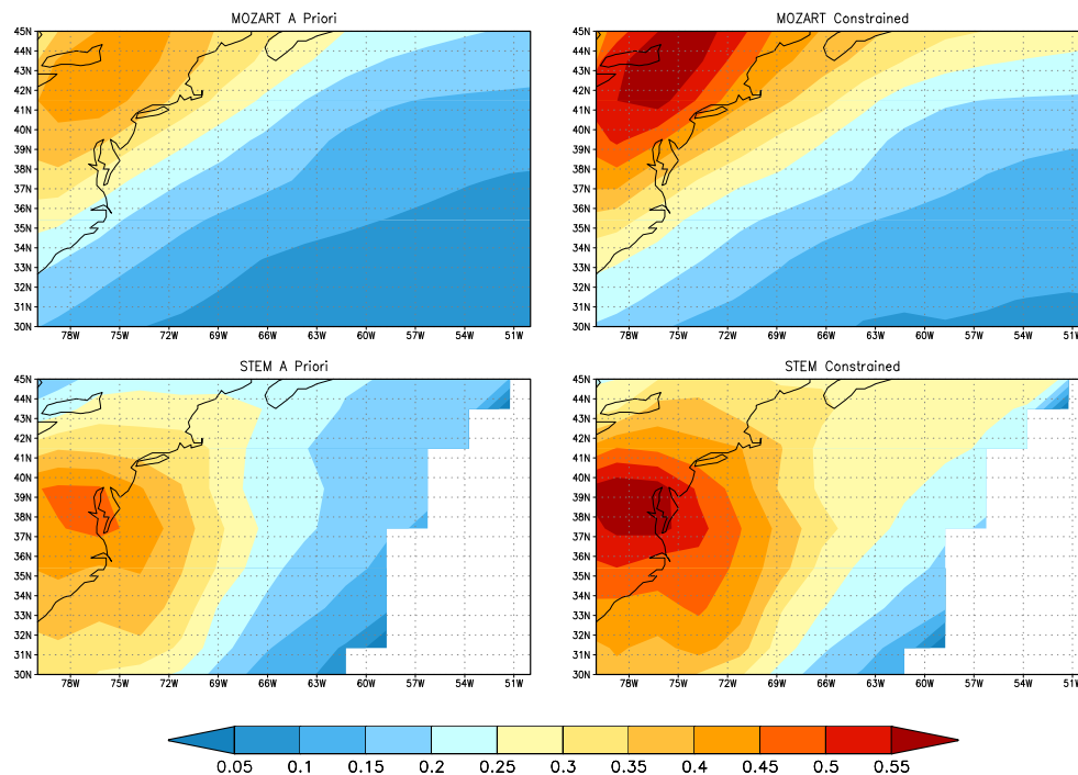
Fig. 21. NWA AOD at 0.55 \mu\text{m} with MOZART aerosols (top panel) and STEM aerosols (bottom panel). First column is with the “a priori” aerosol optical properties; second column is with the constrained optical properties. Note that the STEM simulation in NWA does not cover the whole domain.
