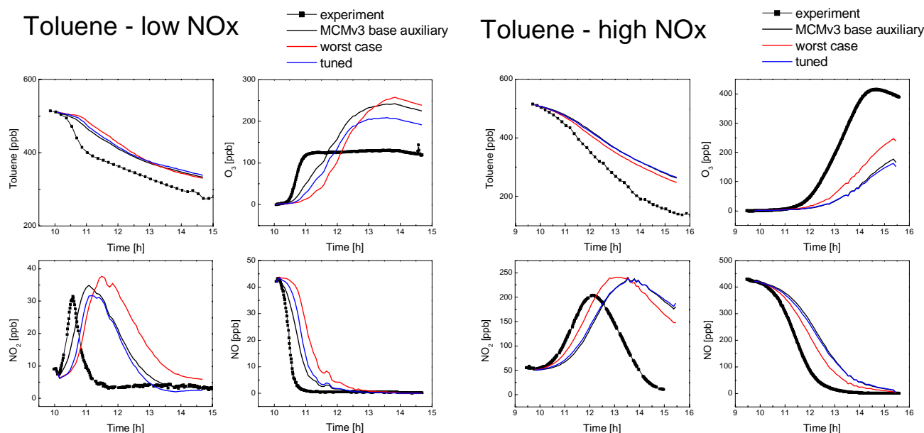
Fig. 3. Simulations of toluene photostmog experiments with base case, worst case and tuned auxiliary mechanism as determined from analysis of the ethene experiments.
