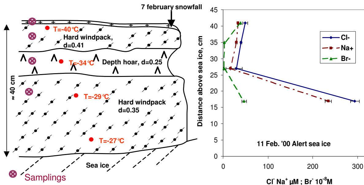
Fig. 2. Stratigraphy and concentrations of \text{Cl}^- , \text{Na}^+ and \text{Br}^- in a snow bank on sea ice near Alert, on 11 February 2000. Density ( d ) and temperature ( T ) values of the snow are indicated. Symbols for snow crystals are those recommended by Colbeck et al. (1990).
