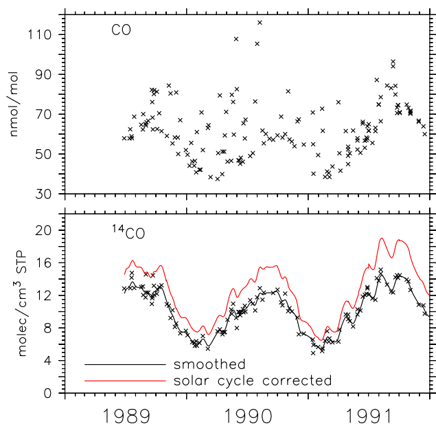
Fig. 4. CO (upper) and ^{14}\text{CO} (lower) measurements at Baring Head ( 41.4^\circ\text{S} , 174.9^\circ\text{E} ), New Zealand for the years 1989 to 1991. The black solid line shows the data smoothing, the red line indicates the smoothed data corrected with respect to solar variation of the GCR ^{14}\text{CO} background production rate using neutron count rates of the Mt. Wellington ( 42.92^\circ\text{S} , 147.25^\circ\text{E} ) neutron monitor. The scatter in CO is the result of CO from local sources during non background conditions. This CO is free of ^{14}\text{CO} . Non clean air conditions were included to not bias the ^{14}\text{C} record towards specific meteorological conditions.
