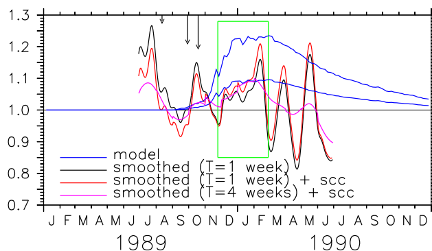
Fig. 5. Observed (black), and solar cycle corrected (scc) observed (red, cf. Fig. 4), enhancement of ^{14}\text{CO} for June 1989 to June 1990 with June 1990 to June 1991 as reference year at Baring Head. The 3 SPEs in 1989 are indicated by the arrows at the top. The relative arrow-lengths correspond to the estimated total ^{14}\text{CO} production of the respective SPE. The blue lines show the results of the model prediction for normal cut-off rigidity (lower line) and an 80% reduced cut-off rigidity (upper line). The purple line shows the observations smoothed with a time window of T=4 weeks, and corrected for the solar cycle (scc).
