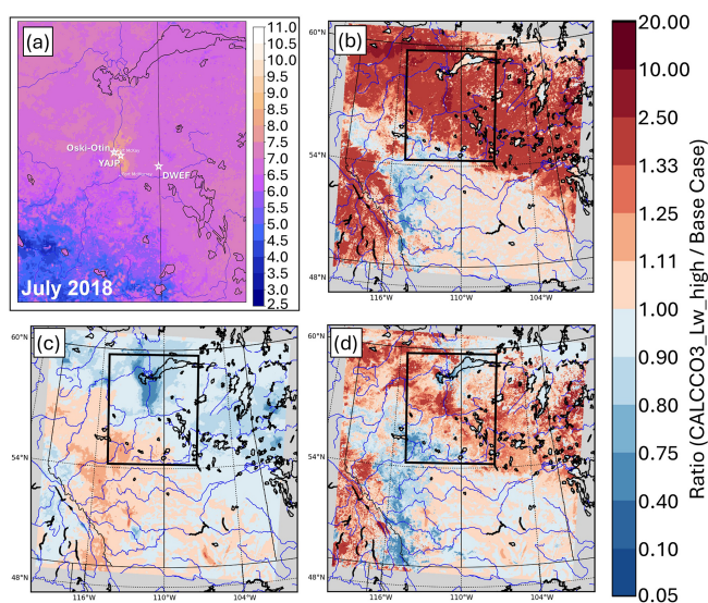
Figure 8. Average impact of surface foliage pH. July, 2018. Panels as in Fig. 6. Figure S5 shows the Base Case and CALCCO3_Lw_high values corresponding to (b), (c), (d). The locations of Oski-otin, YAJP and DWEF (stars) are provided for reference to Fig. 9.
