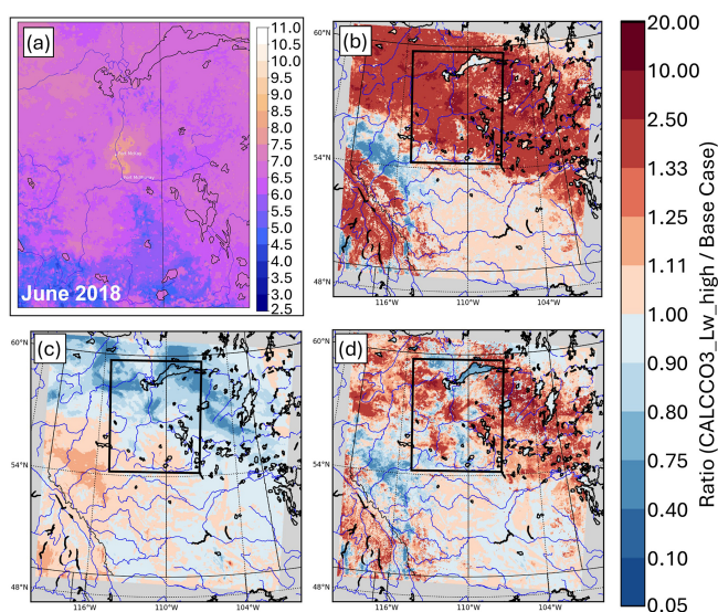
Figure 7. Average impact of surface foliage pH. June, 2018. Panels as in Fig. 6. Figure S4 shows the Base Case and CALCCO3_Lw_high values corresponding to (b), (c), (d).
