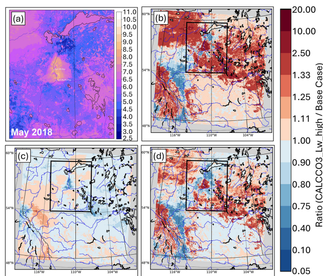
Figure 6. Average impact of surface foliage pH. May, 2018. (a) AOSR average surface foliage pH calculated using CALCCO3_Lw_high. (b, c, d) Ratios (CALCCO3_Lw_high : Base Case) of (b). V_{\text{dSO}_2} , (c) \text{SO}_2 concentration at the surface, (d) Monthly \text{SO}_2 deposition flux at the surface. Inset box in (b), (c), (d) shows the AOSR, displayed as a “zoom” in (a). Figure S3 shows the Base Case and CALCCO3_Lw_high values corresponding to (b), (c), (d).
