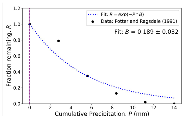
Figure 4. Linear least squares best fit of R = \exp(-P \times B) , where R is the fraction of mass remaining on the leaf after P mm of cumulative rainfall. The fitting parameter B is estimated to be 0.189 \pm 0.032 . Data were obtained by interpolating data presented graphically in Potter and Ragsdale (1991).
