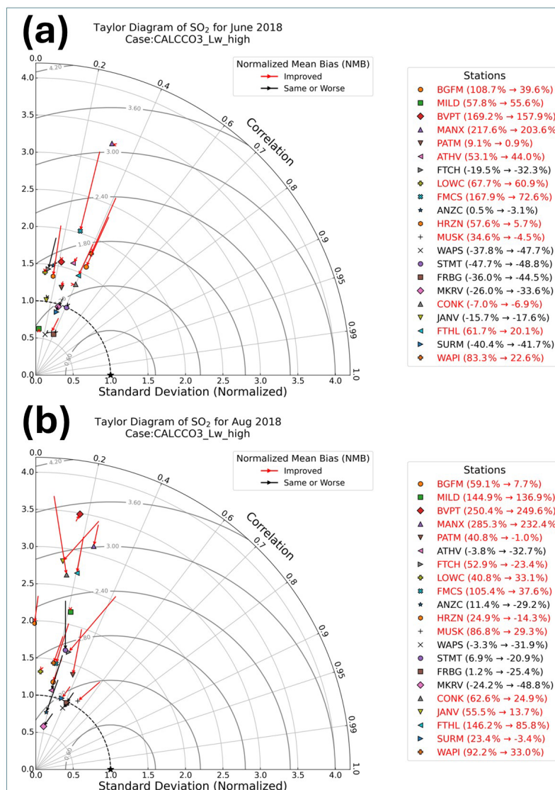
Figure 11. Taylor Diagram of SO 2 for (a) June 2018, (b) August 2018 (see Fig. S10 for May and July). The equations used to compute these metrics are provided in Table S3. In each panel, the “star” symbol on x -axis marks the reference point for a perfect model, corresponding to a correlation = 1.0, a CRMS = 1.0 and a normalized standard deviation = 1.0. Arrows illustrate changes in model performance from the Base Case (arrow start) to CALCCO3_Lw_high (arrow end). A trajectory that moves closer to the reference point indicates improved agreement with observations (red arrows). The CRMS is proportional to the distance from the star; concentric circles centred on the star represent contours of constant CRMS. The standard deviation is measured radially from the origin. The different WBEA stations are denoted by different symbols, with each arrow pointing from the Base Case to CALCCO3_Lw_high locations of station performance on the diagram. Red (black) arrows denote an improvement (deterioration or no change) in the normalized mean bias error (NMB) for CALCCO3_Lw_high compared to the Base Case. The value of the NMB for each station is shown in the legend after the station name as (Base Case → CALCCO3_Lw_high), with red text likewise representing improvements in the NMB when using CALCCO3_Lw_high compared to the Base Case. The azimuthal distance represents the correlation (i.e., r ) starting from 0.0 and increasing clockwise to 1.0. The radial distance from the origin gives the normalized standard deviation of the model at the station. Each station standard deviation has been normalized by the observed standard deviation at that station. Thus, the observed standard deviation is always at (1.0, 1.0) represented by the star on each plot. May and July Taylor diagrams are given in the Supplement, Fig. S10.
