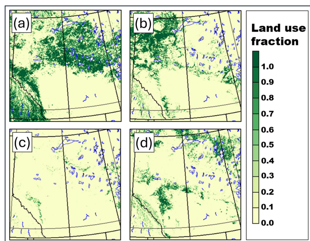
Figure 3. Land use fractions (0.0–1.0) for vegetation classes in GEM-MACH simulations: (a) evergreen needleleaf forests, (b) deciduous broadleaf trees, (c) mixed wood forests and (d) dwarf trees, shrubs with ground cover. While GEM-MACH contains classes for evergreen broadleaf and deciduous needleleaf forests, the land-use fraction for these categories is 0.0 in the entire geographic domain investigated here.
