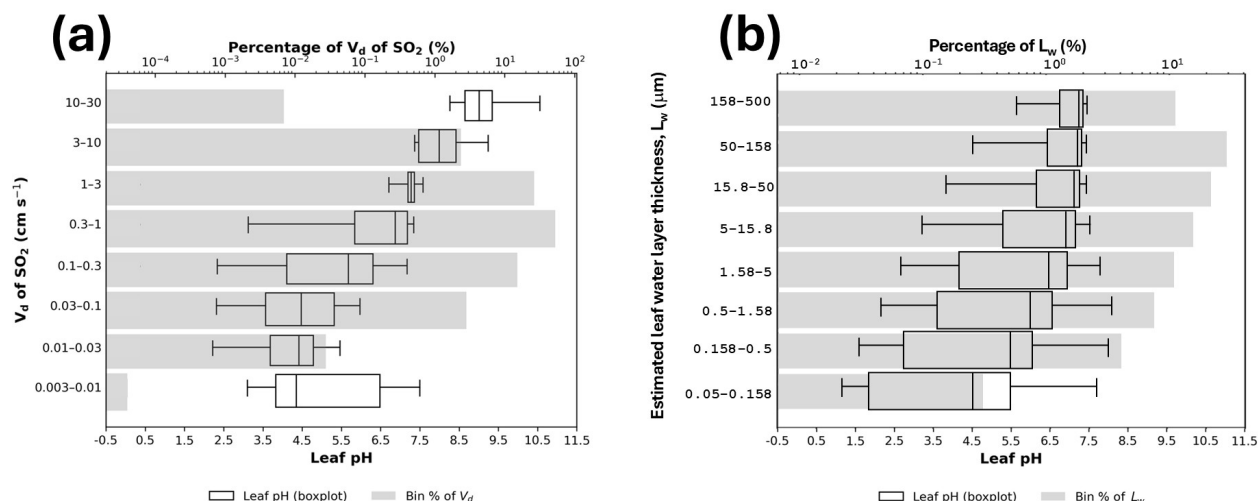
Figure 5. (a) The deposition velocity of \text{SO}_2 ( V_{\text{dSO}_2} , \text{cm s}^{-1} ) as a function of foliage (leaf) pH; data are from May 2018. V_{\text{dSO}_2} has been separated into 8 discrete bins, and the corresponding box plots give the range of leaf pH (lower x-axis) within each bin. The whiskers, box boundaries, central vertical line, etc. from left to right for each box are the 5th percentile, 25th percentile, median, 75th percentile, and 95th percentile, respectively. This format for box plots is applied henceforth. Each box is superimposed over a shaded bar that gives the percentage of V_{\text{dSO}_2} in the corresponding bin (upper x-axis). (b) The foliage (leaf) pH as a function of the estimated leaf water layer thickness ( L_w , \mu\text{m} ). L_w has been separated into 12 discrete bins, and the corresponding box plot gives the range of leaf pH in the corresponding bin. The shaded bars give the percentage of L_w in each bin (right y-axis).
