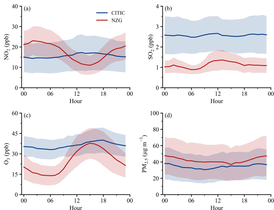
Figure 9. Diurnal variations of \text{NO}_2 , \text{SO}_2 , \text{O}_3 , and \text{PM}_{2.5} during observational period (2020–2024) at the CITIC (blue) and NZG (red) stations, respectively. The shaded areas denote 50 % standard deviation.
