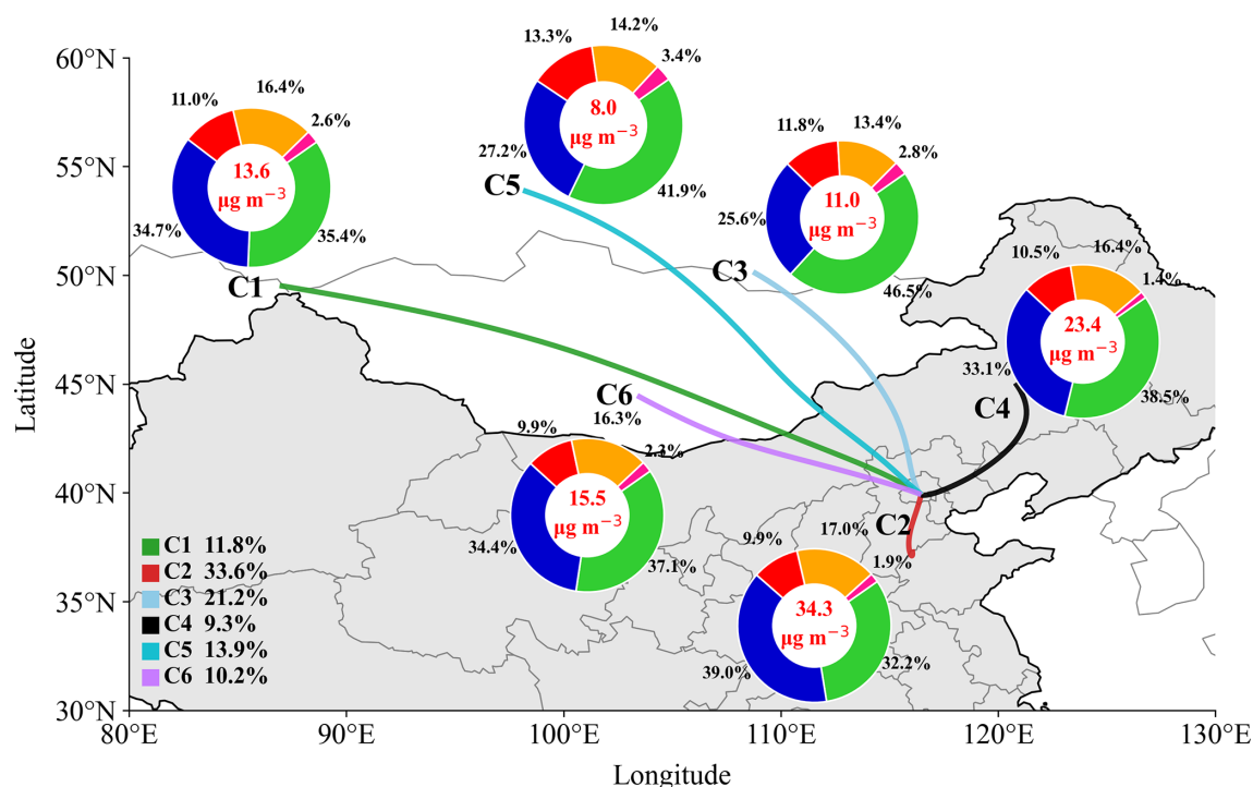
Figure 3. Forty-eight hours back trajectories of air masses over Beijing at altitude of 500 m in the six clusters (C1–C6), together with the mean NR-PM 2.5 mass concentration and composition at the CITIC station in each cluster.
