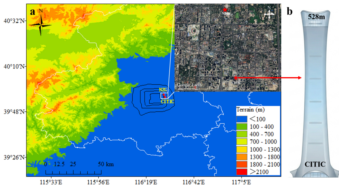
Figure 1. Locations of the monitoring sites used in this study with lack lines, red dots representing the second to fifth rings surrounding central Beijing, and CITIC and NZG stations, respectively (a); sketch map of the 528 m CITIC Tower (b).
