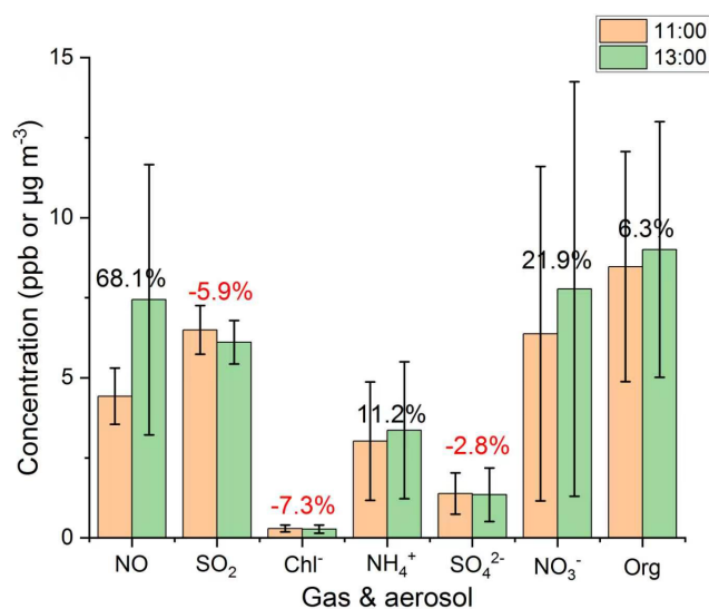
Figure 10. Mean concentrations of gases and aerosol components at the CITIC station at 11:00 and 13:00 LT from 17 October to 12 November 2020. Values indicate the percentage variations of pollutants between 11:00 and 13:00 LT. Error bars represent 50 % of the standard deviations.
