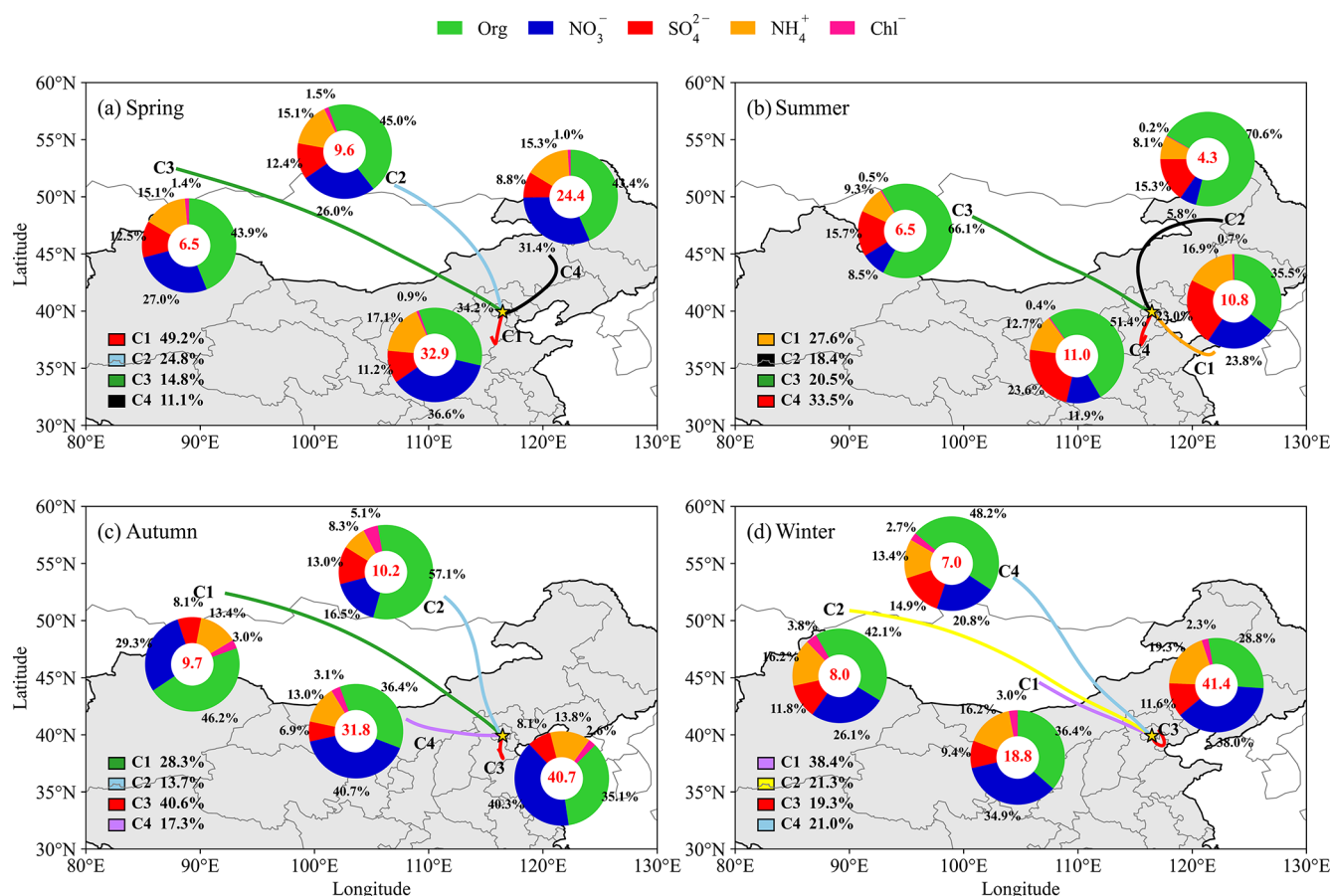
Figure 8. Forty-eight hours back trajectories of air masses over Beijing at altitude of 500 m in four seasons, together with mean mass concentration and composition of NR-PM 2.5 in each cluster.
