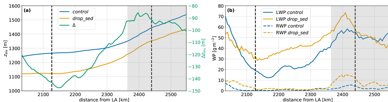
Figure 6. Time evolution of the (a) inversion height z_{\text{inv}} and (b) water paths (WP) of Leg 12A in the hours 26 to 40 of the simulation. The vertical dashed lines enclose the analysis period for this section. In panel (b), the solid lines depict the liquid water path (LWP), while the dashed ones depict the rain water path (RWP). For the water paths, a 1 h rolling mean was applied. Colours as in Fig. 3 and grey shading marks local night-time.
