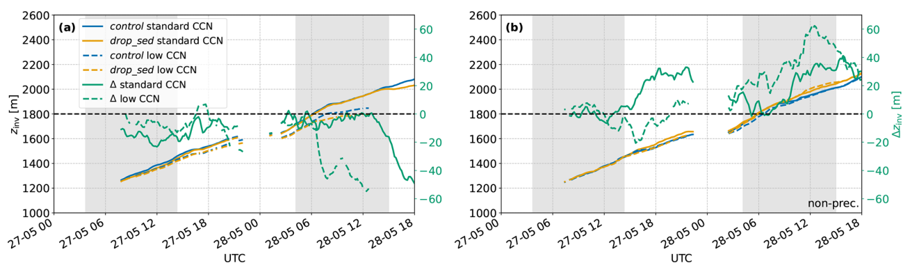
Figure 9. Inversion heights z_{\text{inv}} of the (a) precipitating and (b) non-precipitating low CCN sensitivity experiments for Leg 11A. Colours and shading as in Fig. 8. The solid lines represent the standard CCN scenario ( 250 \text{ cm}^{-3} ), while the dashed lines represent the low CCN scenario ( 100 \text{ cm}^{-3} ).
