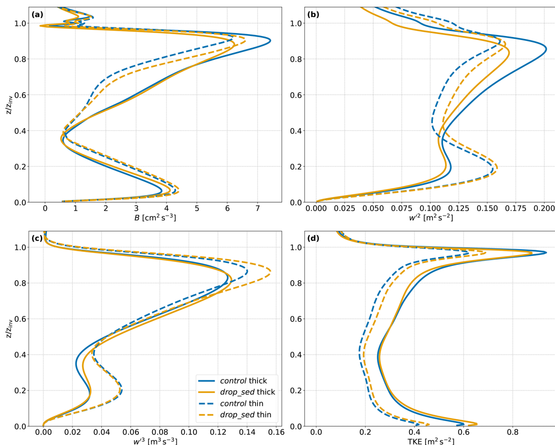
Figure 5. Total mean relative profiles of the (a) buoyancy flux B , (b) vertical wind variance w'^2 , (c) third moment of the vertical wind w'^3 and (d) turbulent kinetic energy (TKE). Lines and colours as in Fig. 4.
