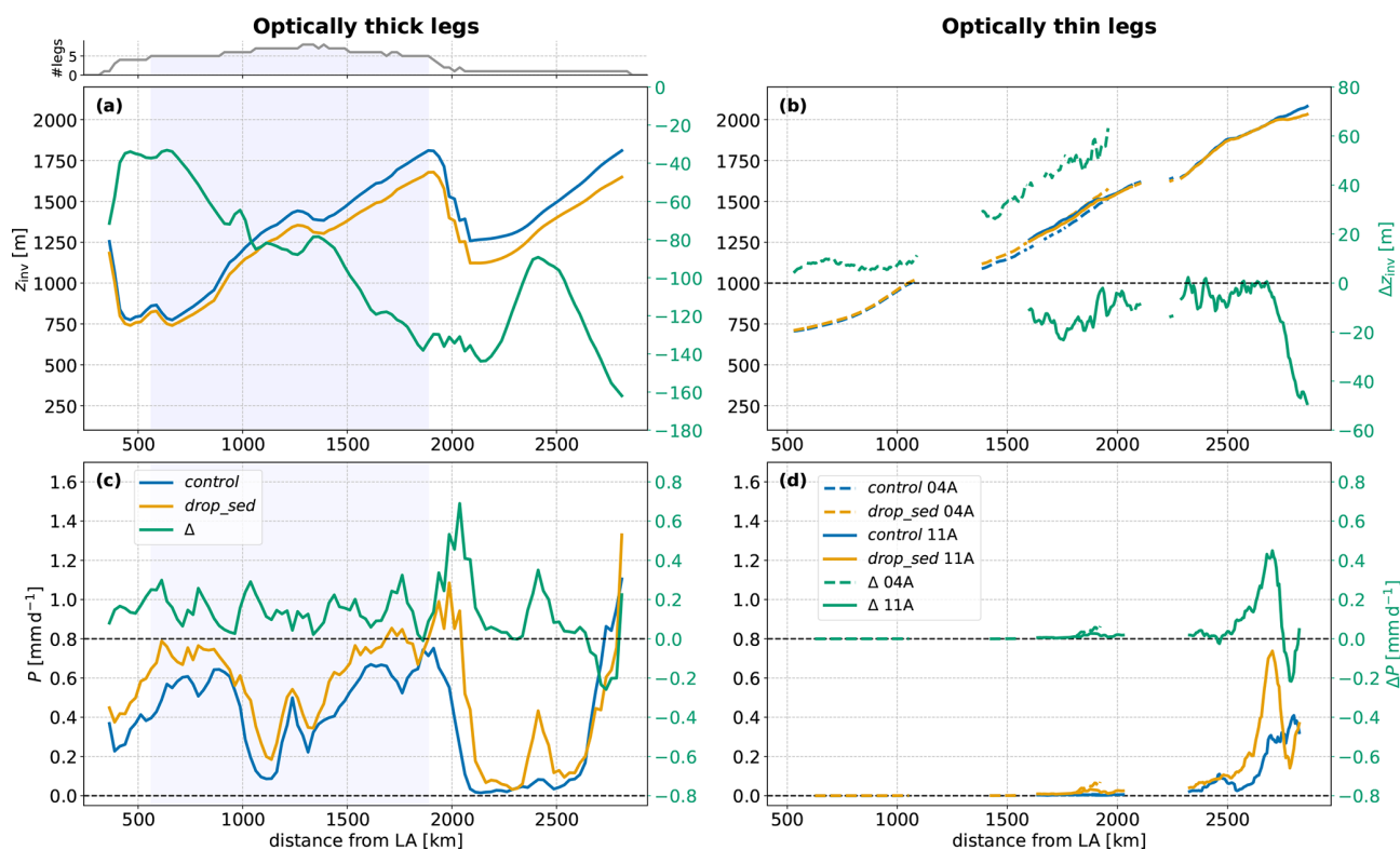
Figure 3. Binned distance plots of the inversion height z_{\text{inv}} (top panels) and the surface precipitation rate P (bottom panels), separated by category. Panels (a) and (c) represent the thick legs, whereas panels (b) and (d) represent the thin legs. The former are combined into one curve with the leg contribution depicted above the panels in grey, whereas the latter are depicted individually using dashed (solid) lines for Leg 04A (Leg 11A). The left y-axis corresponds to the absolute magnitude of both control (blue) and drop_sed (orange), while the right y-axis corresponds to the difference \Delta (green). The light blue shading indicates the core region, where at least five legs are contributing. In all panels save for (b), a rolling mean of roughly 75 km was applied.
