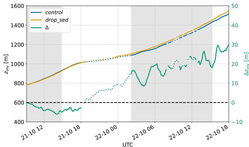
Figure A2. Leg 04A inversion height z_{\text{inv}} of the long spinup experiment, where droplet sedimentation is activated only after 15 h. Colours and shading as in Fig. 3. The dotted periods correspond to the stages where the mean cloud fraction is below 40 %.
