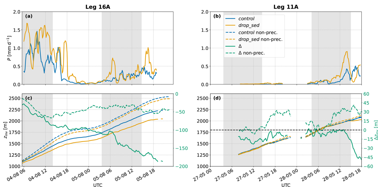
Figure 8. Comparison of the representative legs for the thick category (Leg 16A, left) and thin category (Leg 11A, right). The top panels (a) and (b) show the surface precipitation rates P , while the bottom panels (c) and (d) show the results for the inversion height z_{\text{inv}} , respectively. For the precipitation rates, a 1 h rolling mean was applied. The solid lines represent the precipitating runs, whereas the dashed lines represent the non-precipitating runs. Colours are the same as in Fig. 3 and the grey shading marks local night-time.
