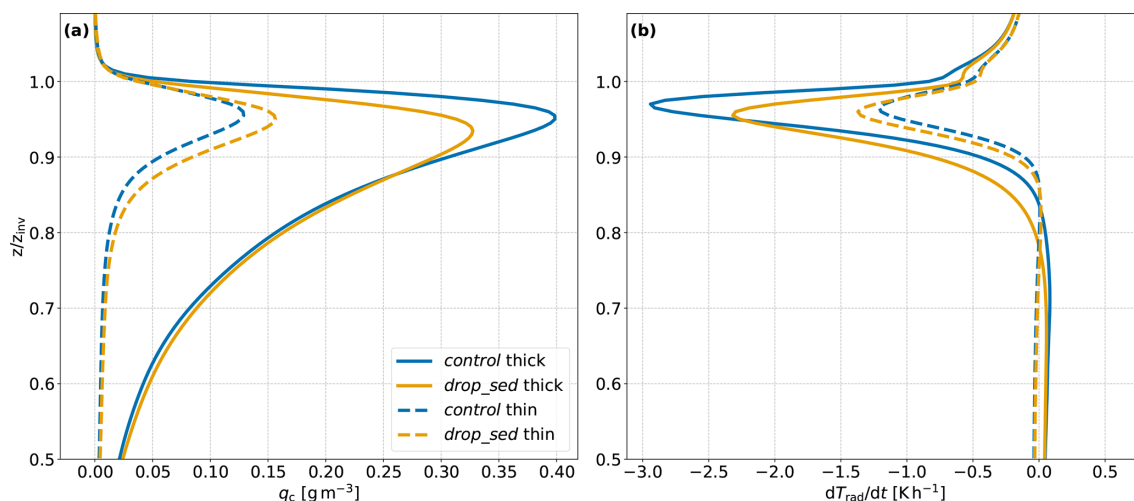
Figure 4. Total mean relative profiles of (a) liquid water content q_c and (b) radiative heating rate dT_{\text{rad}}/dt . The profiles were normalised to the inversion height z_{\text{inv}} at each time step before computing the mean. The thick (thin) legs are represented by solid (dashed) lines. Note that the y-axis is cut at 0.5. Colours as in Fig. 3.
