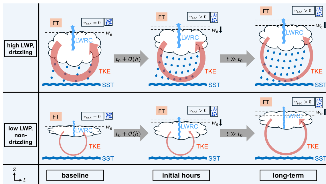
Figure 11. Schematic to illustrate the impact of droplet sedimentation on the two different idealised cloud categories (top: optically thick and precipitating, bottom: optically thin and non-precipitating). Both show a similar initial effect regarding entrainment, but evolve structurally different afterwards. The first stage is the baseline state at time t_0 before sedimentation is activated (indicated by v_{\text{sed}} ). The middle stage is the state in the initial hours and the last stage is the state after a longer period of time. The cloud thickness is a rough measure of the liquid water path (LWP), the light blue arrows indicate longwave radiative cooling (LWRC), while the red arrows indicate turbulent circulations (turbulent kinetic energy, TKE). The ocean surface is illustrated by blue waves (sea surface temperature, SST). Dashed lines represent the inversion height z_{\text{inv}} under the dry free troposphere (FT), where entrainment occurs (marked by w_e ), with the control inversion in grey for comparison, while the arrow thickness represents the strength of the respective quantity. Note that the light blue arrows are intentionally placed in the middle (bottom) of the cloud, if radiative cooling is saturated (unsaturated).
