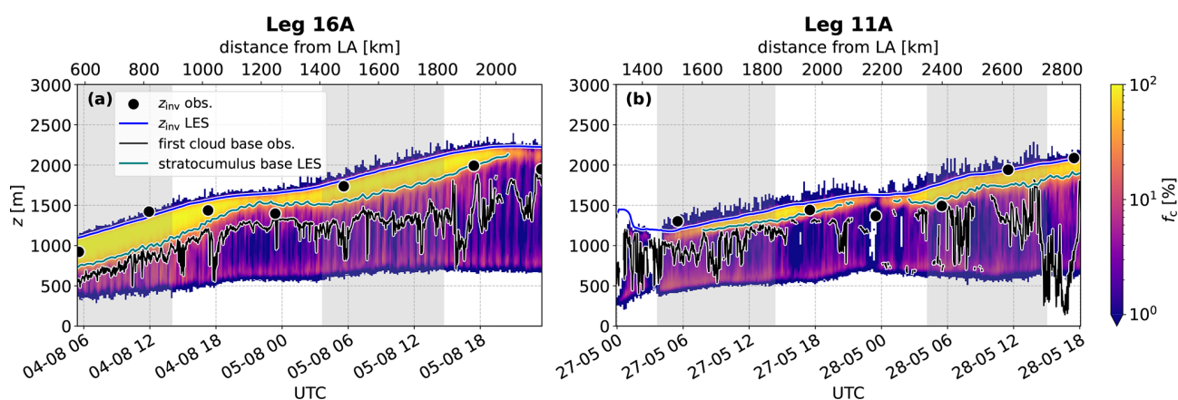
Figure 1. Domain-averaged cloud fraction f_c of the control runs of (a) Leg 16A and (b) Leg 11A as a function of height z over the course of the simulation. The bottom x -axis marks the respective time of the transect, while the top x -axis marks the distance from Los Angeles. The blue line shows the LES inversion, while the teal line shows the lowest height of f_c = 40\% , if it exists. The black dots symbolise the observed inversion height based on the ship radiosonde launches (Keeler et al., 2022), whereas the black line depicts the observed first cloud-base based on the ship ceilometer (Zhang et al., 1996). The latter was resampled to a time step of 1 min for better visibility. Grey shading marks local night-time.
