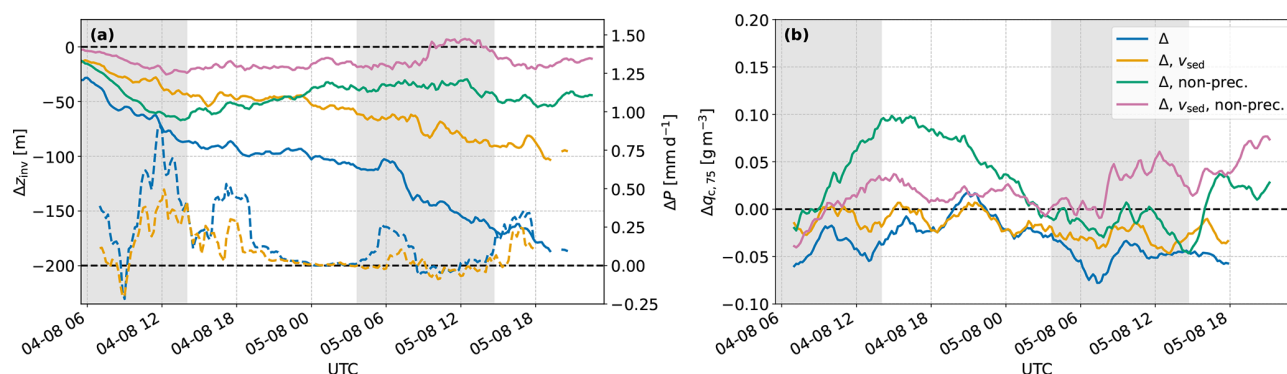
Figure 10. Leg 16A difference plots for (a) the inversion height z_{\text{inv}} (solid) as well as the surface precipitation rate P (dashed) and (b) the mean liquid water content in the top 75 m of the cloud q_{c,75} . The blue line and the green line are the respective differences in the default precipitating and the default non-precipitating setup (cf. Fig. 8c for z_{\text{inv}} ). The orange line and the magenta line are the analogous respective differences, but with a halved sedimentation velocity in the drop_sed run. All lines apart from z_{\text{inv}} were smoothed by a 3 h rolling mean. Shading as in Fig. 8.
