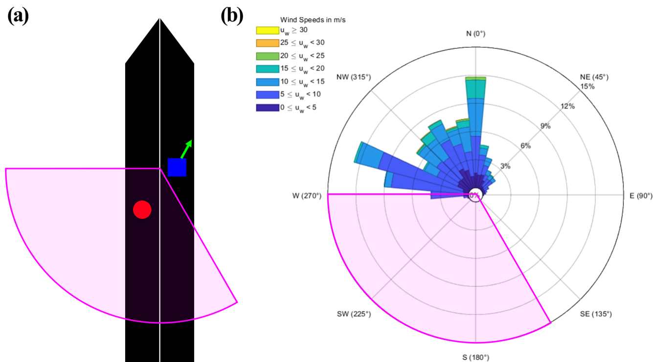
Figure 2. (a) Schematic diagram of the observation room and plume stack, and (b) relative wind rose plot during the transit voyage of the R/V ISABU. The red circle, blue square, and green arrow represent the plume stack, observation room, and the direction of inlets, respectively. The magenta circular sector indicates a range from 150 to 270°.
