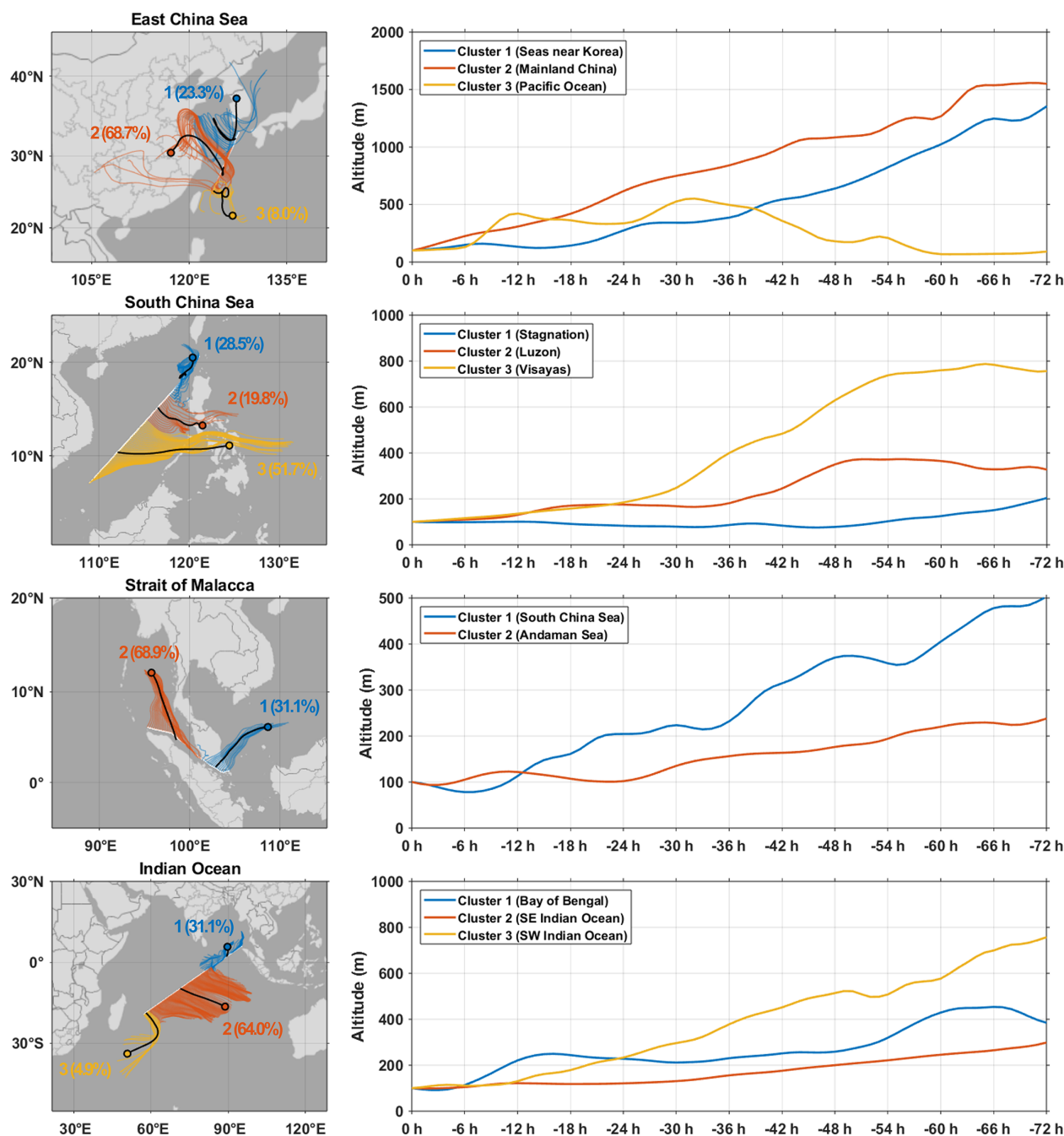
Figure 12. Cluster analysis results for each sea area and mean altitude variations of 72 h back trajectories within each cluster. The thick black solid lines with dots at their ends represent the mean trajectories of each cluster. The percentages in parentheses indicate the proportion of trajectories assigned to each cluster. Map data from Natural Earth.
