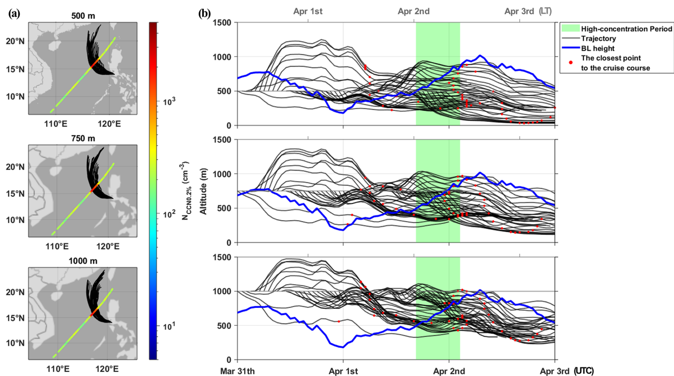
Figure 6. (a) A total of 48 trajectories originating at 500, 750, and 1000 m above the Taal volcano at every hour from 00:00 on 31 March to 23:00 on 1 April (UTC). The color scale represents CCN number concentrations at 0.2 % supersaturation. Map data from Natural Earth. (b) Altitudes of trajectories and boundary layer height at the location of the R/V ISABU . The green shading indicates the volcanic-influence period from 16:30 on 1 April to 02:30 on 2 April (UTC). The red dots denote the times at which each trajectory was closest to the cruise route.
