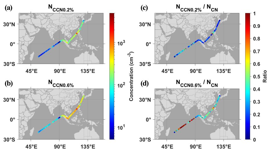
Figure 5. Spatial distributions of (a, b) CCN number concentrations at 0.2 % and 0.6 % supersaturation and (c, d) their ratios to total aerosol number concentrations during the transit voyage of the R/V ISABU (from Natural Earth).
