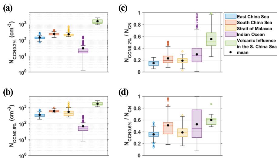
Figure 8. Box plots of (a, b) CCN number concentrations at 0.2 % and 0.6 % supersaturation and (c, d) their ratios to the total aerosol number concentrations for each sea area. For the South China Sea, the volcanic-influence period was depicted separately. The horizontal line in each box and the black dots represent the median and mean values, respectively. The range of the box is from the 25th percentile to the 75th percentile (IQR). The whiskers extend away from the box to the two extreme values, but if there are data points that exceed 1.5 \times \text{IQR} from the upper or lower end of the box, they are shown as colored dots as outliers.
