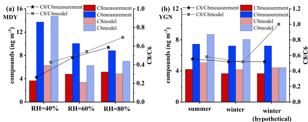
Figure 7. (a) Concentration distributions of C_8H_9NO_4 and C_6H_5NO_4 under different RH conditions in Mandalay. (b) Concentration distributions of C_8H_9NO_4 and C_6H_5NO_4 during Yangon summer, winter and winter hypothetical. Dark-colored bars represent the observed mass concentrations, while light-colored bars indicate the mass concentrations simulated by the model.
