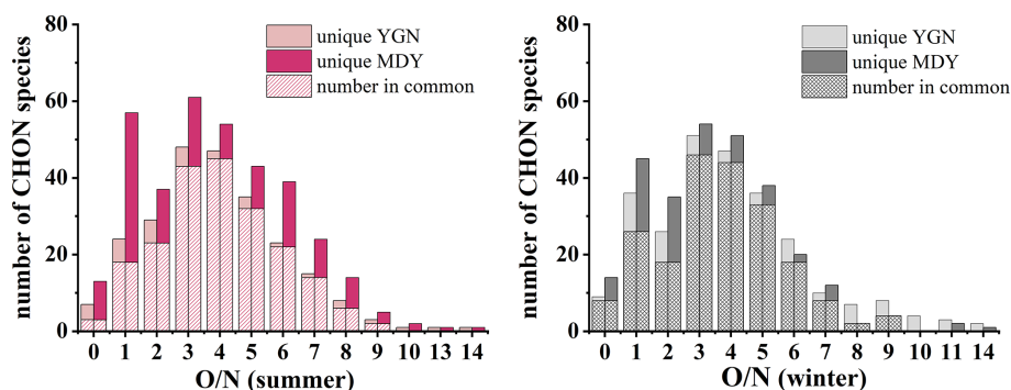
Figure 3. Numbers of common and region-specific compounds in MDY and YGN binned by O/N ratio. Number in common refers to the number of CHON compounds detected in both YGN and MDY, whereas unique YGN and unique MDY denote the numbers of CHON compounds detected exclusively in YGN and MDY, respectively.
