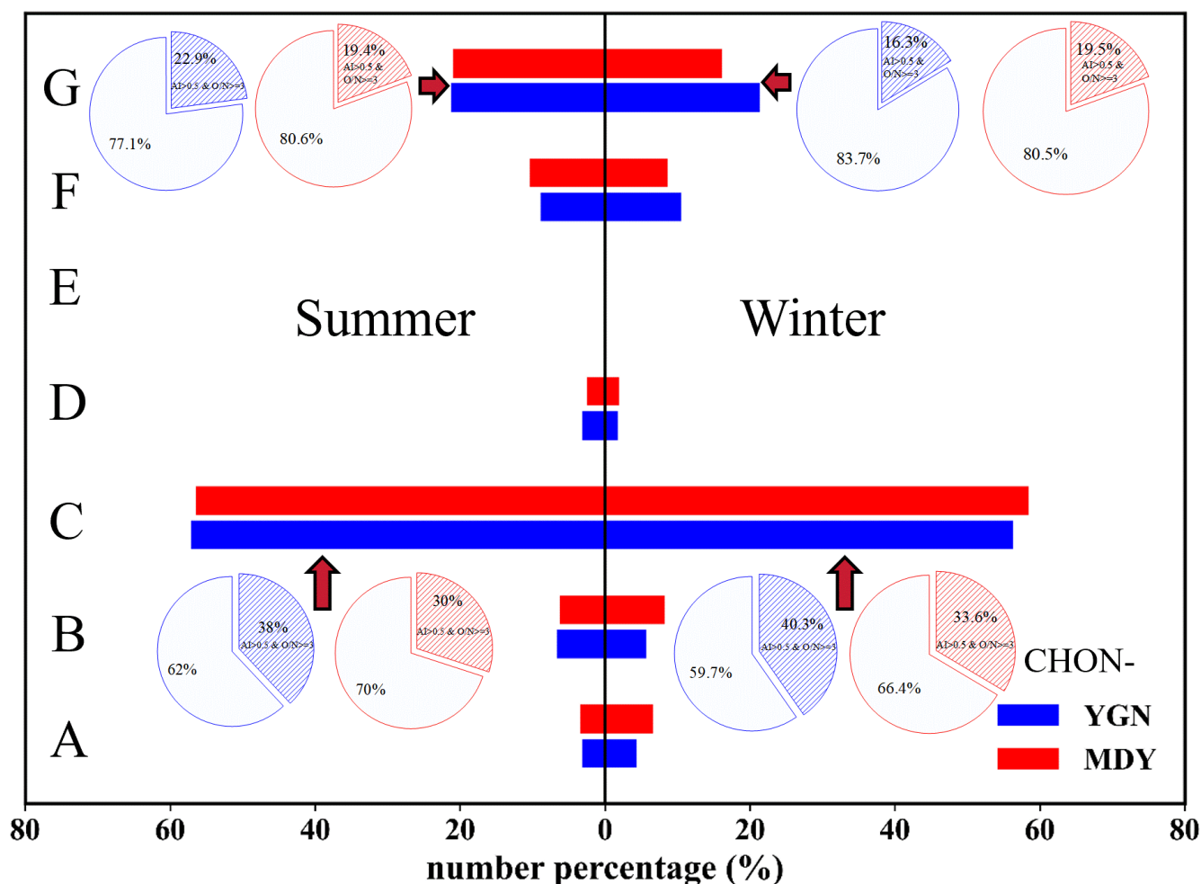
Figure 5. Percentage of CHON- subfraction groups (A–G). Shaded sections in the pie charts represent the number proportion of nitrophenolic compounds within each corresponding subgroup. Blue denotes the Yangon site, while red represents the Mandalay site.
