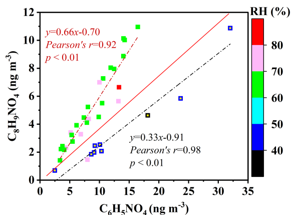
Figure 6. The correlation between \text{C}_6\text{H}_5\text{NO}_4 and \text{C}_8\text{H}_9\text{NO}_4 . Color bar is relative humidity. Yellow stars represent MDY summer samples.
