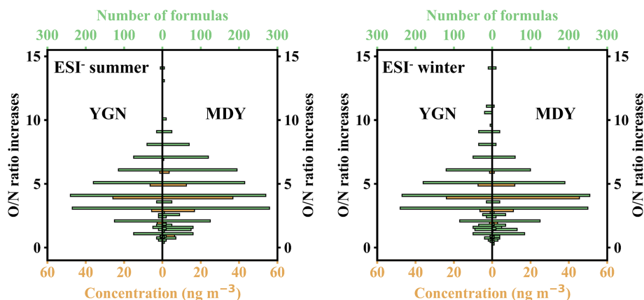
Figure 2. Classification of CHON compounds into subgroups based on O/N ratios in the ESI − mode. Yellow and green colors indicate the ONs mass concentrations ( \text{ng m}^{-3} ) and number of species in each subgroup, respectively.
