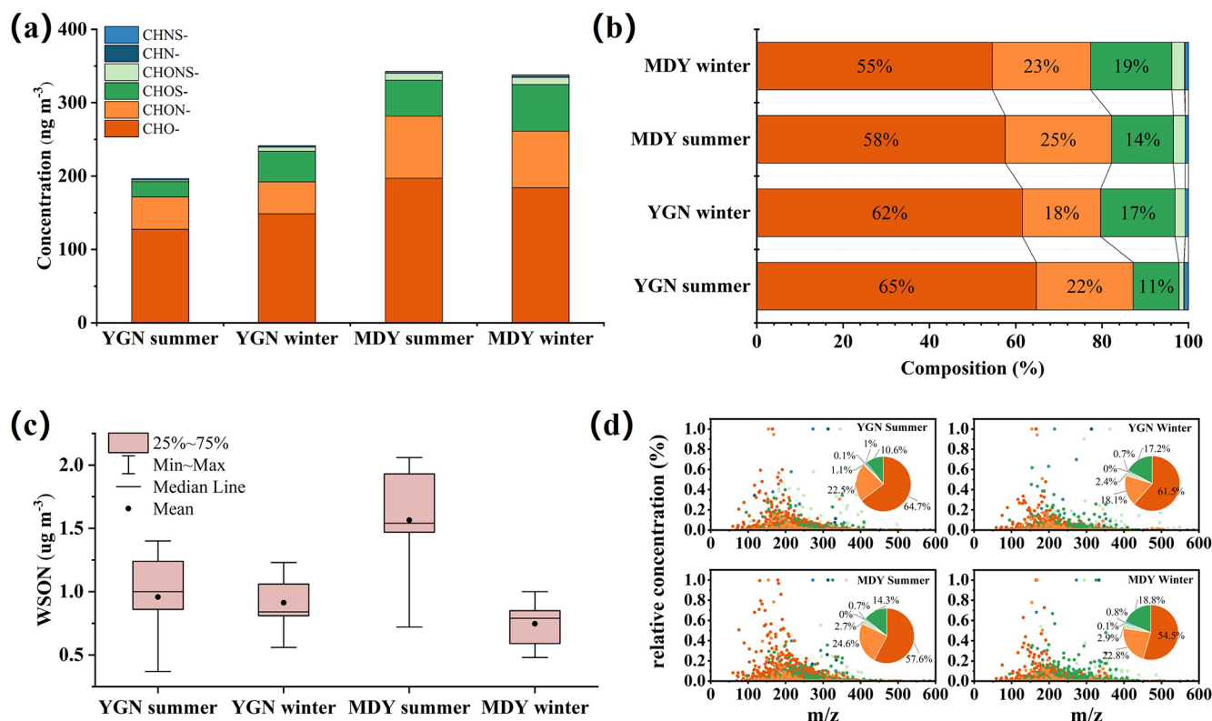
Figure 1. Molecular characteristics of organic matter in Yangon (YGN) and Mandalay (MDY). (a) Semi-quantitative concentrations of CHO, CHON, CHON, CHOS, CHONS, CHN, and CHNS species detected in both cities during summer and winter in the ESI − mode. (b) Percentage contributions of CHO, CHON, CHOS, CHONS, CHN, and CHNS species to the total molecular mass concentrations in both cities during summer and winter in the ESI − mode. (c) Mass concentration of WSON in both cities during summer and winter. (d) Reconstructed mass spectra of organic compounds derived from extracted ion chromatograms in the ESI − mode. The vertical axis represents the semi-quantitative normalized concentration of each compound. The pie charts illustrate the seasonal average concentration contributions of different molecular species.
