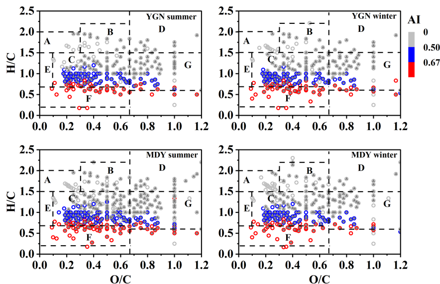
Figure 4. CHON- Van Krevelen (VK) diagram for the identified compounds. According to the H/C and O/C ratios, organic compounds are classified into seven categories (A–G). Color bars represent the aromaticity index (AI), while grey triangles denote compounds with O/N \geq 3 .
