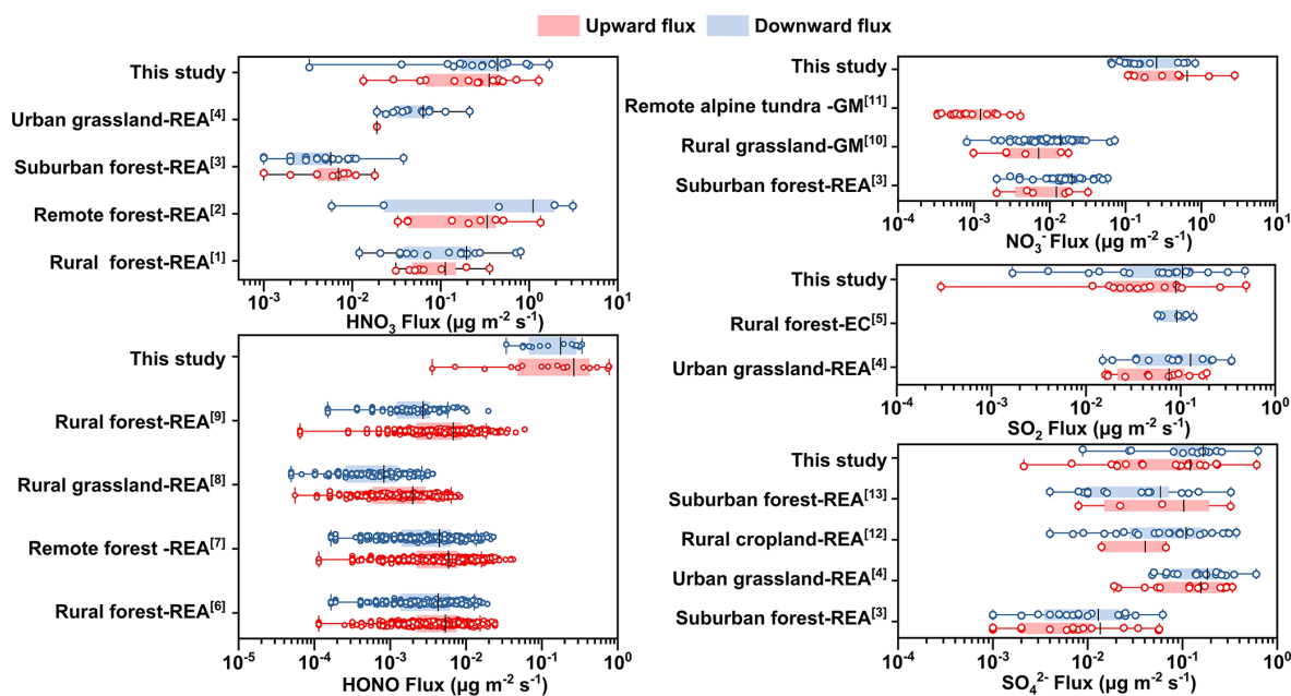
Figure 4. The comparison of the fluxes observed in this study and those reported in the literature. We primarily compiled REA-measured fluxes from the literature, supplementing with EC and GM measurements due to the limited availability of REA flux data for \text{NO}_3^- and \text{SO}_2 . Downward fluxes are represented as positive values in blue to simplify plotting, while upward fluxes are shown in red. (1) Pryor et al. (2002), (2) Hansen et al. (2015), (3) Xu et al. (2021), (4) Myles et al. (2007), (5) Meyers et al. (1998), (6) Zhou et al. (2011), (7) Ren et al. (2011), (8) von der Heyden et al. (2022), (9) Zhang et al. (2012), (10) Huebert et al. (1988), (11) Rattray and Sievering (2001), (12) Meyers et al. (2006), (13) Matsuda et al. (2015).
