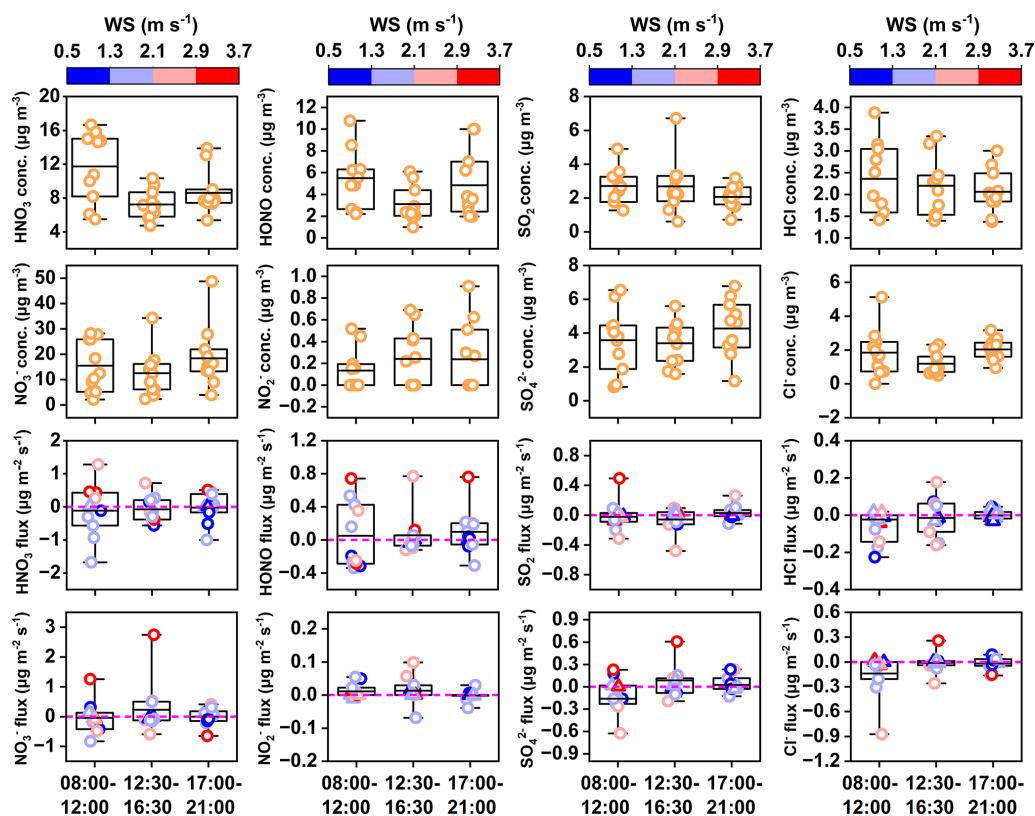
Figure 2. Box-and-whisker plots with overlaid data points for eight inorganic species, grouped by diurnal time intervals. Top two rows: diurnal concentration variations of gaseous ( \text{HNO}_3 , HONO, \text{SO}_2 , HCl) and particulate ( \text{NO}_3^- , \text{NO}_2^- , \text{SO}_4^{2-} , \text{Cl}^- ) species. Bottom two rows: REA-measured fluxes of the same species, with flux points color-coded by horizontal wind speed. Horizontal lines mark means, and boxes denote interquartile ranges.
