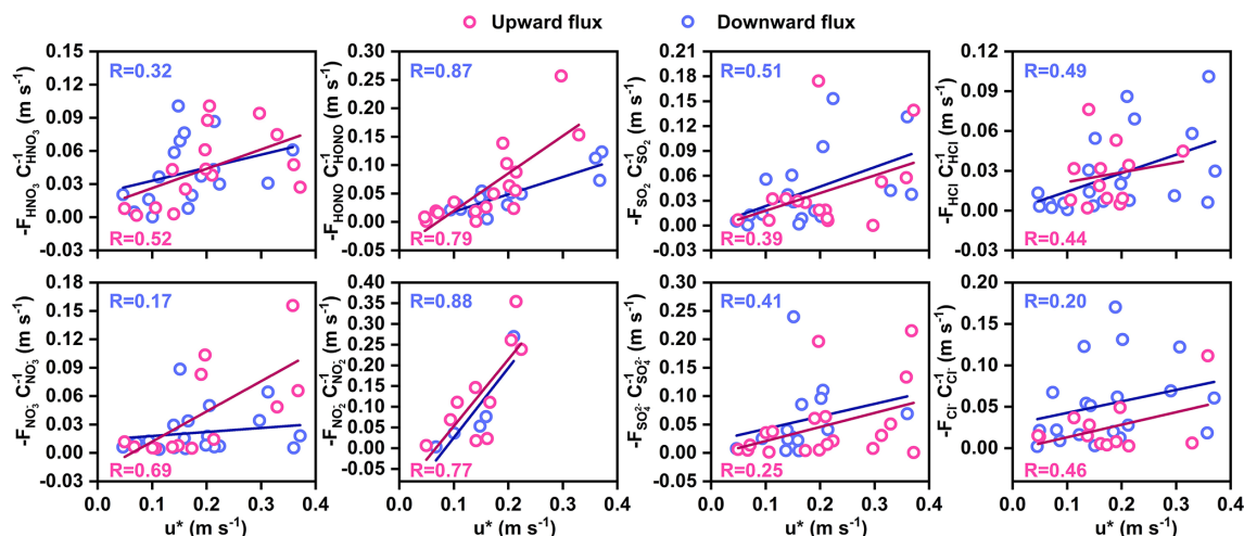
Figure 5. Apparent deposition velocities (calculated as -F/C for downward fluxes and F/C for upward fluxes) of inorganic acidic gases and particles versus friction velocity ( u^* ). Red and blue symbols denote upward and downward fluxes, respectively.
