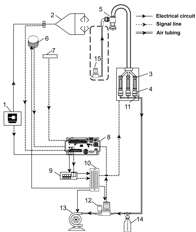
Figure 1. Schematic diagram of the REA flux sampling device for atmospheric inorganic gas and particles. (1) Power supply; (2) 3D sonic anemometer; (3) Denuder tube; (4) Filter-pack cartridge; (5) Cyclone inlet; (6) Vaisala Weather Transmitter; (7) Thermocouple; (8) Data logger; (9) Relay; (10) Terminal block for signal and power distribution; (11) Fast switching valves; (12) Mass flow controller (MFC); (13) Pump; (14) 500 ml buffer bottle; (15) Mass flow meter (MFM) used in test runs only.
