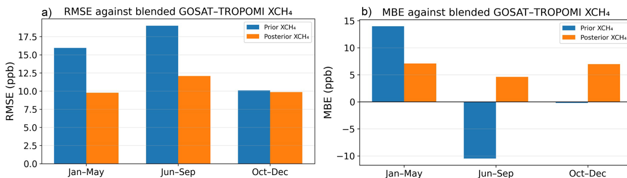
Figure 12. Seasonal RMSE (a) and MBE (b) of prior and posterior modeled XCH 4 relative to GOSAT-TROPOMI blended dataset. Statistics are shown for January–May, June–September, and October–December. The posterior simulation shows reduced errors and seasonal biases compared to the prior.
