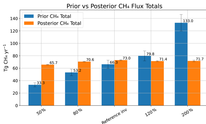
Figure 13. Sensitivity of total posterior methane emissions to prior flux magnitude scaling. The prior inventory was uniformly scaled to 50 %, 80 %, 120 %, and 200 % of its original magnitude. Blue bars show the corresponding prior totals and orange bars the posterior totals.
