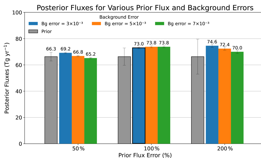
Figure 14. Posterior CH 4 flux estimates as a function of prior-flux uncertainty (50 %, 100 %, 200 %) and three background-error settings (0.3 % in blue, 0.5 % in orange, 0.7 % in green). The reference inversion is outlined in black. The prior flux and its uncertainty are shown as separate grey bars for each group for comparison.
