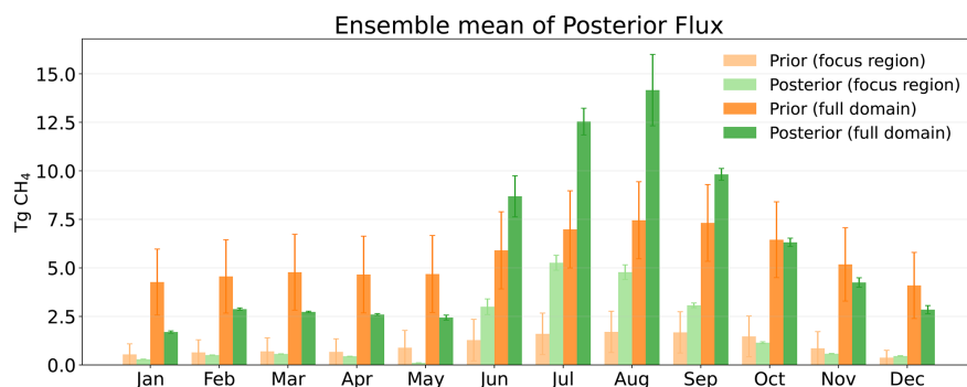
Figure 15. Ensemble mean monthly \text{CH}_4 fluxes ( \text{Tg yr}^{-1} \text{CH}_4 ), showing prior estimates (orange) and posterior means (green) with \pm 1\sigma error bars across nine inversion experiments. Error bars for the prior represent the prescribed prior uncertainty used in the reference inversion.
