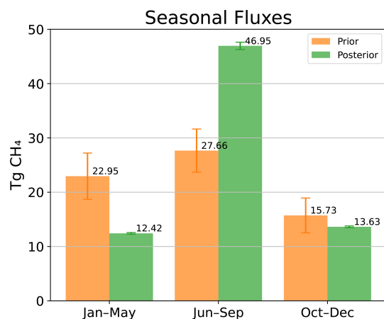
Figure 8. Seasonal methane fluxes (Tg CH 4 ) over South Asia for three periods (January–May, June–September, October–December), comparing prior fluxes (orange bars) with posterior fluxes (green bars). Error bars indicate the corresponding uncertainty ranges.
