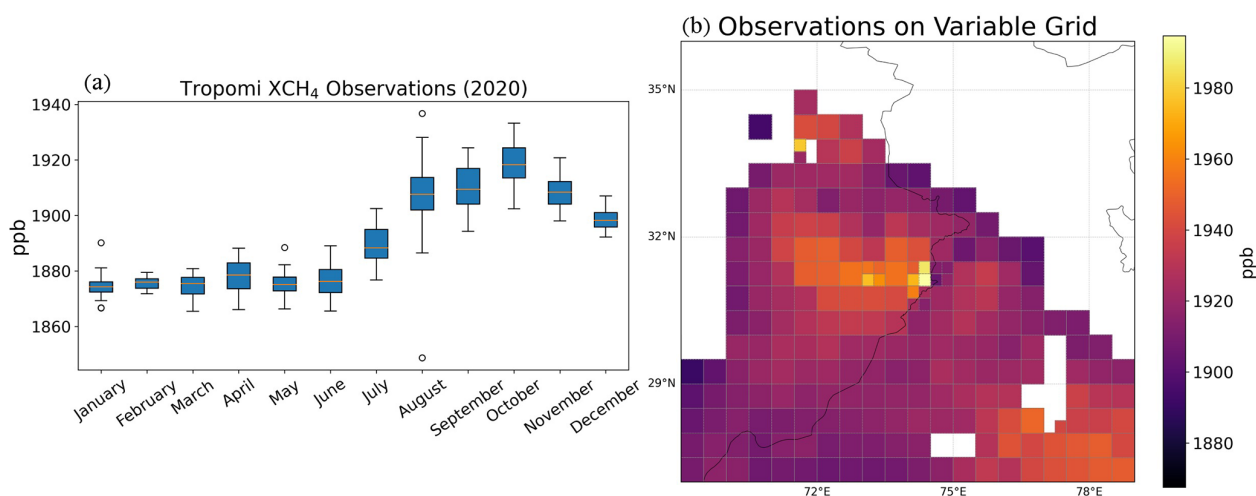
Figure 2. (a) Seasonality of the observed TROPOMI methane column mole fractions ( XCH_4 ) averaged over the whole domain. The blue boxes represent the interquartile range (IQR), the center line the median, the whiskers represent the most extreme data points within 1.5 \times IQR of the monthly mole fractions and the circles are outliers. Also shown is the number of retrievals in each month (orange line). (b) Observations aggregated on a variable resolution latitude/longitude grid ( 0.25^\circ \times 0.25^\circ and 0.50^\circ \times 0.50^\circ ) for a typical day in October. The black circle shows a region where the fine grid is used with larger heterogeneity in mole fractions.
