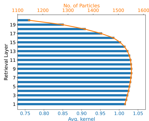
Figure 4. Vertical distribution of particles for a sample retrieval. Blue bars show the averaging kernel values for each retrieval layer, and the orange line indicates the corresponding number of particles released per layer after weighting by the averaging kernel and pressure term.
