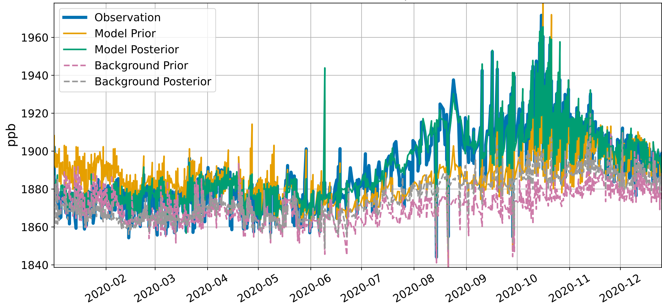
Observed and Modeled CH 4 Mole fractions
