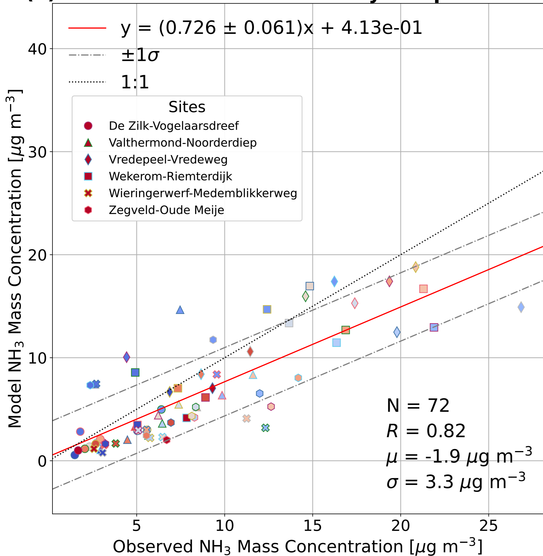
(a) Base Model vs. LML Monthly Temporal Means
