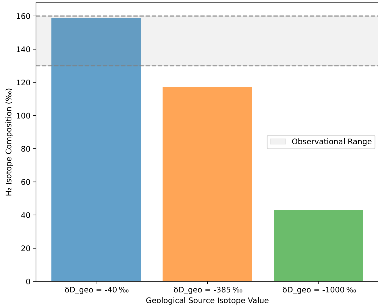
Sensitivity of H 2 Isotopic Composition to Geological \delta D
