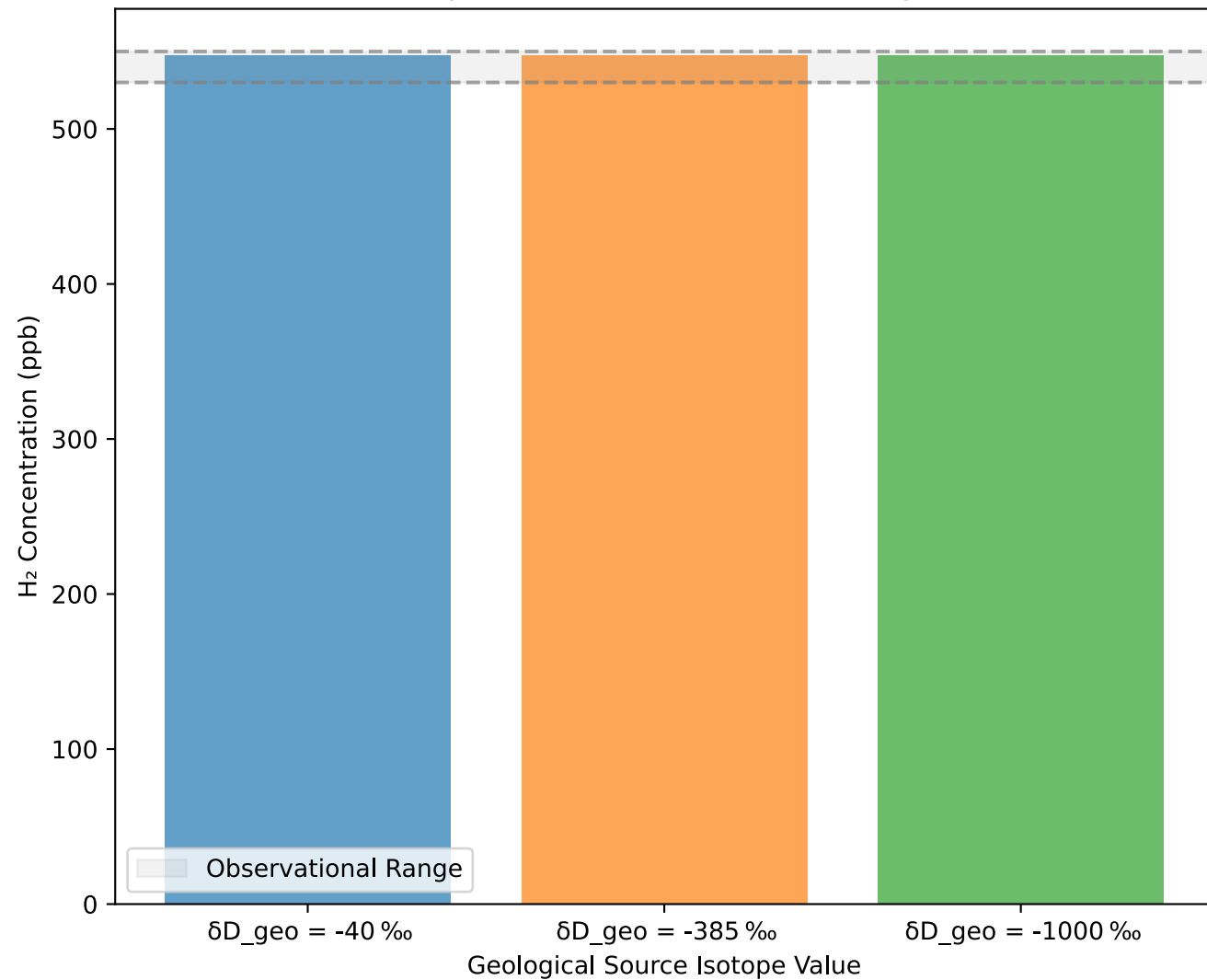
Sensitivity of H 2 Concentration to Geological \delta D
