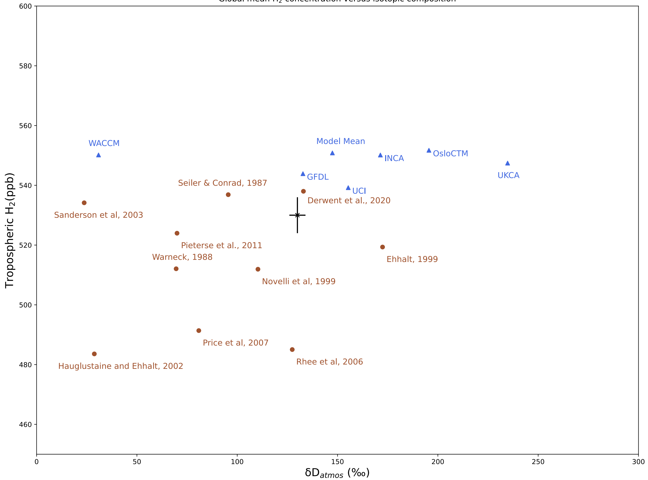
Global mean H 2 concentration versus isotopic composition
