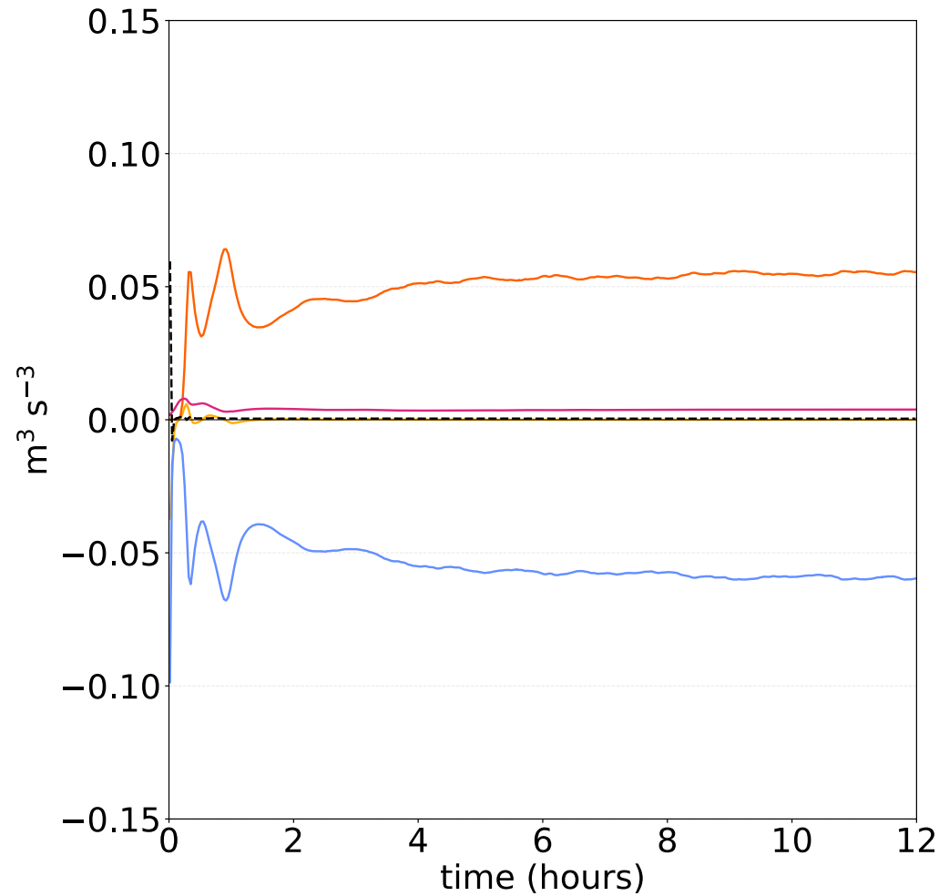
a) closed-cell
