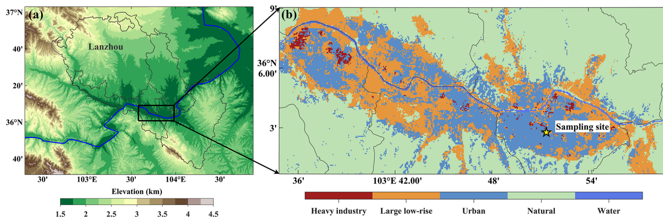
Figure 1. Overview of the location of observations. (a) Regional topography of Lanzhou. The black box denotes the urban area shown in panel (b). (b) Local-scale Local Climate Zone classification of the Lanzhou urban area, with the sampling site marked by a star.
