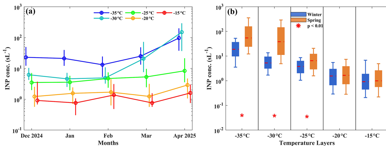
Figure 2. Monthly variations and seasonal differences in INPs. (a) Monthly median INP concentrations. (b) Seasonal box plots of INP concentrations in winter (December–February) and spring (March–April); boxes indicate the interquartile range, whiskers the 10th–90th percentiles, and red asterisks denote significant differences.
