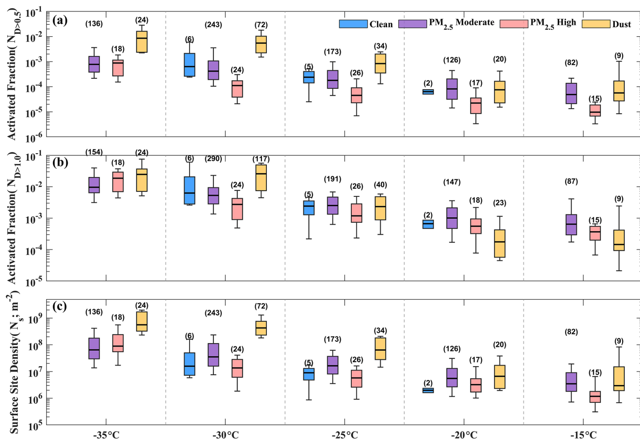
Figure 4. Distributions of ice nucleation activity parameters. Each box shows the 25th–75th percentile range, with the center line indicating the median and the whiskers extending to the 10th and 90th percentiles. Numbers above the boxes indicate the number of samples for each event type at each temperature.
