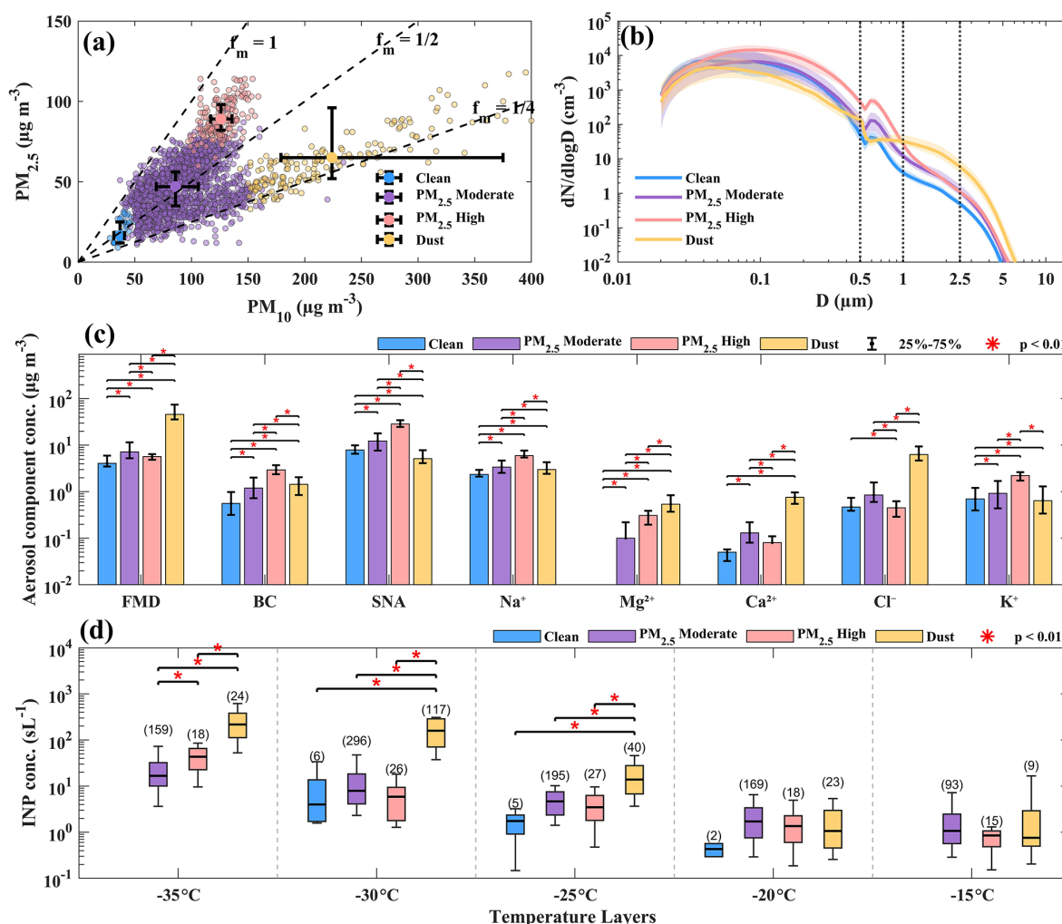
Figure 3. Comparative analysis of physicochemical characteristics and INP concentrations across different aerosol event types. (a) Mass concentrations of PM_{2.5} and PM_{10} . Solid markers indicate the median, error bars represent the 25th and 75th percentiles, and dashed lines show the PM_{2.5}/PM_{10} ratio ( f_m ). (b) Particle number size distribution. The solid line indicates the median, and the gray shading represents the 25th–75th percentile range. (c) Mass concentrations of water-soluble ions, shown as median values for different event types. (d) INP concentrations at different temperatures. Boxes represent the 25th–75th percentiles, red lines inside the boxes indicate the median, and whiskers extend to the 10th and 90th percentiles. Numbers in brackets indicate the number of samples corresponding to combinations of aerosol event types and temperature layers. Red asterisks above the brackets indicate significant differences ( p < 0.01 ) between groups based on median tests.
