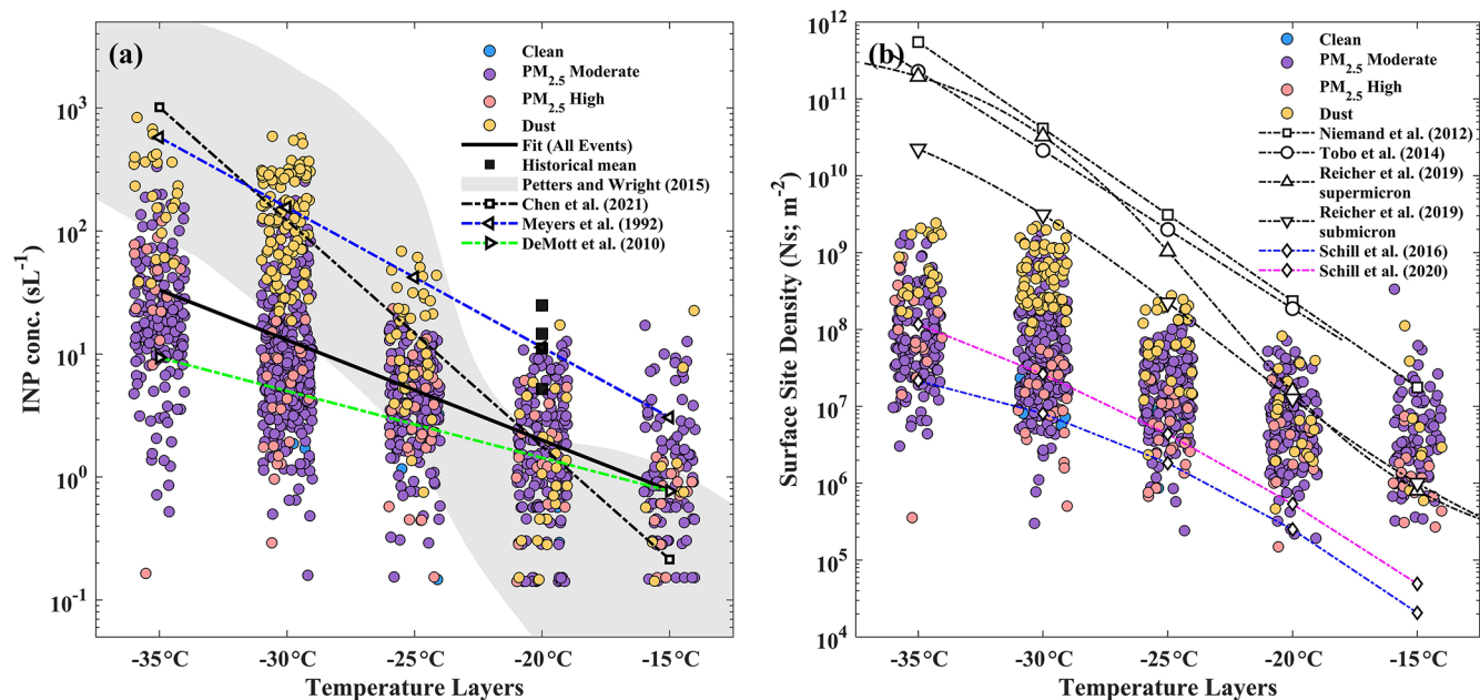
Figure 8. Construction of single-parameter INP parameterizations and comparison with existing parameterization schemes. (a) Temperature dependence of INP concentrations. The black solid line shows the overall fit from all events, and representative literature parameterizations are included for comparison. The gray shaded region denotes the range reported by Peters and Wright (2015). The black square indicates the historical mean INP concentration in Lanzhou (Ge and Zhou, 1986).
