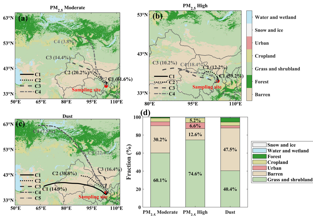
Figure 5. Spatial distributions of 72 h backward air-mass trajectories and associated land-cover characteristics for different aerosol events. Panels (a)–(c) show clustered backward trajectories for (a) PM 2.5 Moderate, (b) PM 2.5 High, and (c) Dust events, overlaid on MODIS land-cover data. The red star indicates the sampling site, and the percentages denote the fraction of trajectories in each cluster. Panel (d) shows the fractional contributions of major land-cover types sampled by trajectories for each event type. Land-cover categories include barren, forest, grass and shrubland, cropland, urban, snow and ice, and water and wetland.
