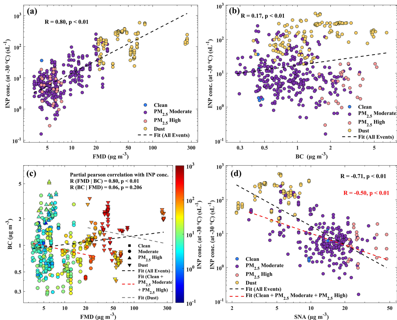
Figure 6. Associations between -30\text{ }^{\circ}\text{C} INP concentrations and aerosol ion components. (a, b, d) Scatter plots of INP concentrations versus FMD, BC and SNA mass concentrations, respectively. R denotes the Pearson correlation coefficient, and p denotes the significance level, calculated in the natural log space. (c) Bivariate plots with FMD and BC on the axes, where the color scale represents INP concentrations. The reported R (FMD | BC) and R (BC | FMD) values denote the partial correlations between FMD and INPs after controlling for BC, and between BC and INPs after controlling for FMD, respectively. All correlations were calculated in natural log space.
