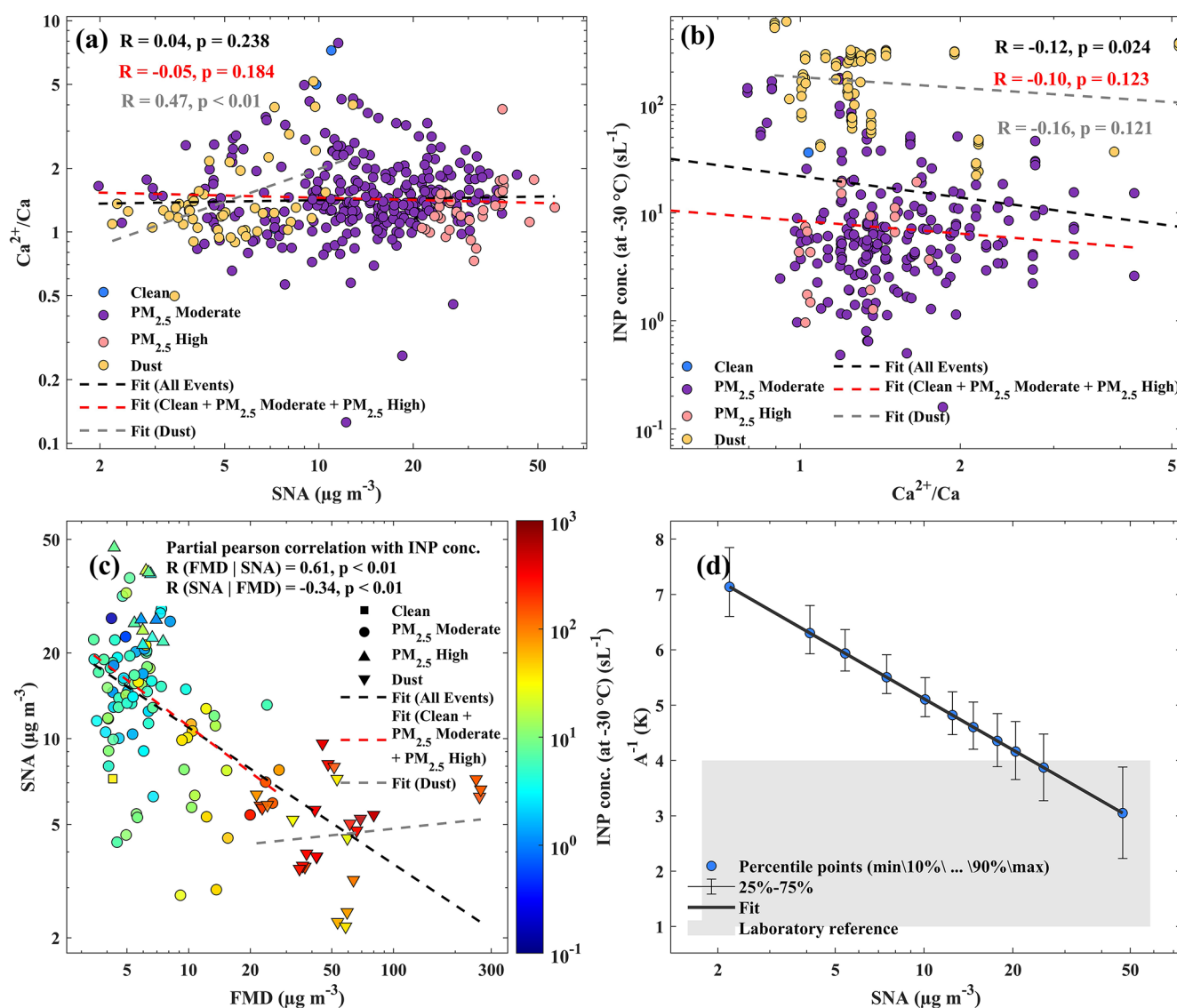
Figure 7. Associations between -30\text{ }^{\circ}\text{C} INP concentrations and SNA. (a) Scatter plots of SNA versus \text{Ca}^{2+}/\text{Ca} . (b) Scatter plots of \text{Ca}^{2+}/\text{Ca} versus INP concentrations. R denotes the Pearson correlation coefficient and p the significance level, calculated in the natural log space. (c) Bivariate plots with FMD and SNA on the axes, where the color scale represents INP concentrations. The reported R(\text{FMD} | \text{SNA}) and R(\text{SNA} | \text{FMD}) values denote the partial correlations between FMD and INPs after controlling for SNA, and between SNA and INPs after controlling for FMD, respectively. All correlations were calculated in natural log space. (d) Dependence of the sensitivity metric A^{-1} on SNA concentrations ( -25 to -35\text{ }^{\circ}\text{C} ). The shaded area indicates the laboratory reference range reported by Villanueva et al. (2025).
