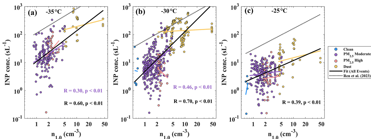
Figure 9. Relationships between INPs and aerosol number concentrations. Panels (a)–(c) show the relationships between INP concentrations and n_{1,0} . The black dashed line indicates the prediction from existing parameterization schemes. The R and p values represent the Pearson correlation coefficient and its significance, and only results with p < 0.01 are shown.
