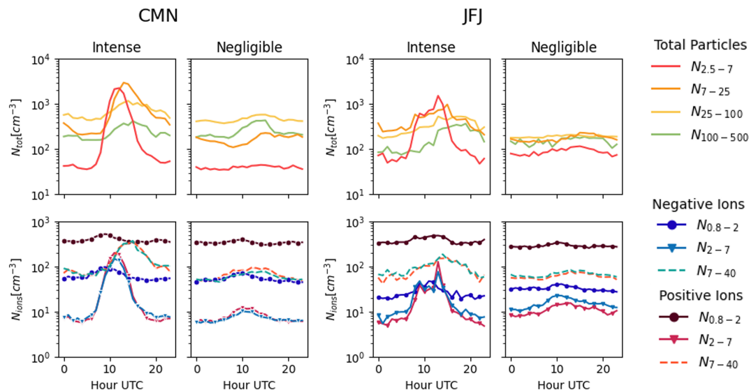
Figure 9. Diurnal variations of total particle number concentrations N_{\text{tot}} , negative ion concentrations and positive ion concentrations N_{\text{ions}} , at two sites CMN (left panel) and JFJ (right panel). Data is shown for Intense and Negligible NPF days. The legend provides particle size ranges with corresponding color codes for total particles, negative ions, and positive ions. Units for all concentrations are in [\text{cm}^{-3}] , and time is shown in UTC hours.
