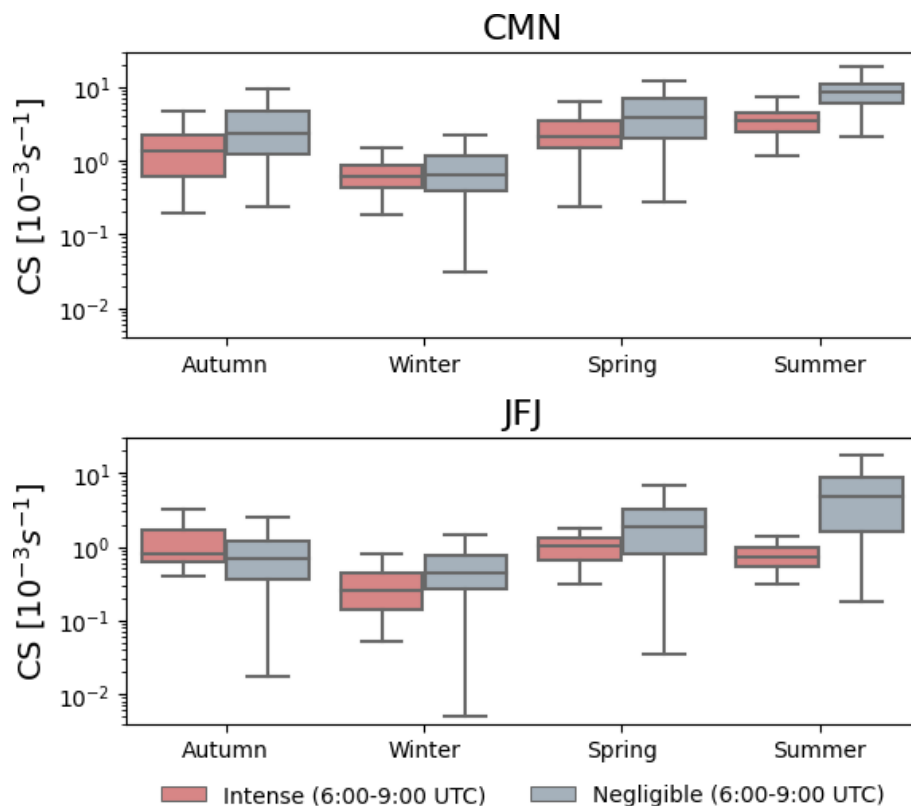
Figure 10. Seasonal variation in Condensation Sink at CMN (top panel) and JFJ (bottom panel) stations. Boxplots represent the logarithmic distribution of CS [ 10^{-3} \text{ s}^{-1} ] during Intense and Negligible event periods (06:00–09:00 UTC) for each season.
