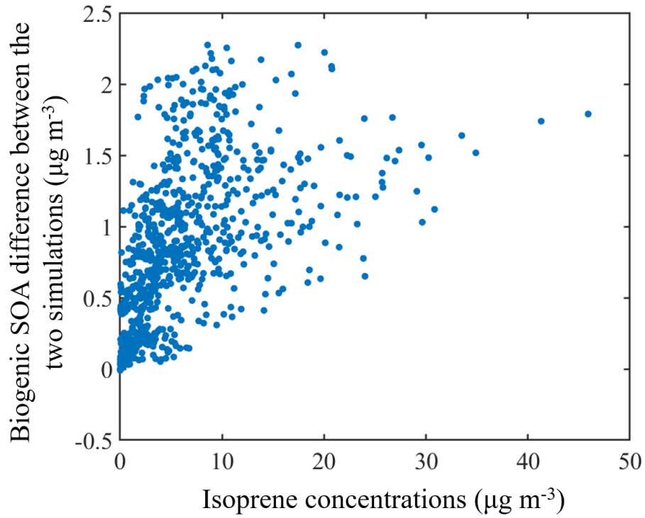
Figure S15. The difference of biogenic SOA concentrations between the two simulations for the simulation cell over Croatia are plotted against the hourly average concentrations of isoprene for the same cell.
