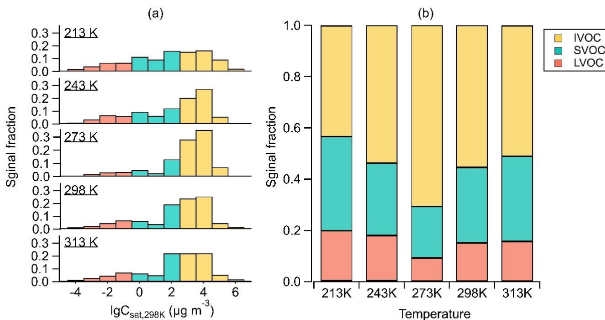
Figure S12. a) Volatility distribution of fresh particles formed at all temperatures corresponding to 298 K saturation concentrations, and b) their fraction the volatility bins: ULVOC, ELVOC, LVOC, SVOC, IVOC, and VOC identified based on the saturation concentrations as described in the Method. Please note that \lg C_{\text{sat},298\text{K}} refer to saturation concentrations at 298 K, which is different from the \log_{10} C_{\text{sat},T} which are related to their formation temperatures.
