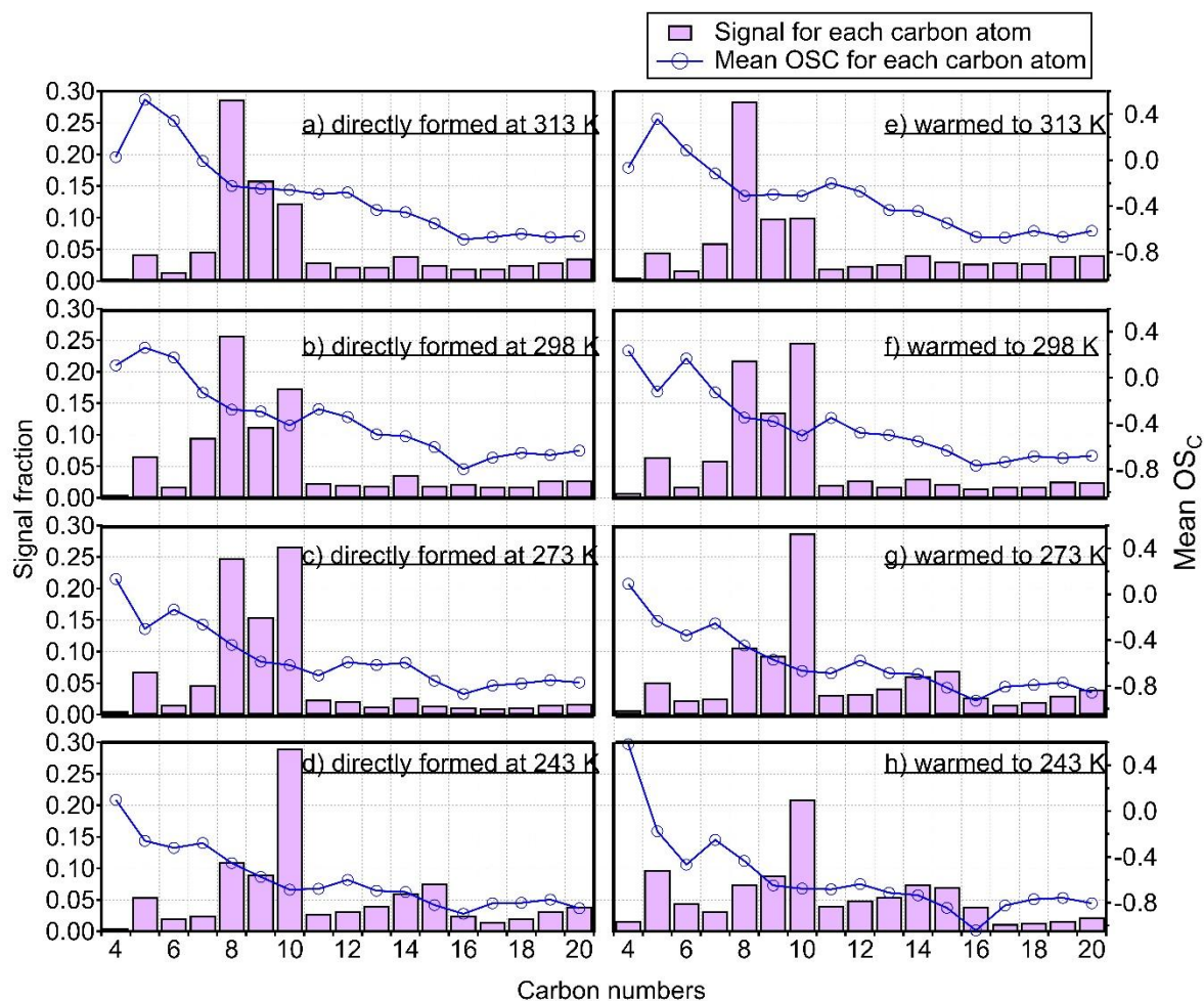
Figure S13. Signal fraction of particle-phase products corresponding to carbon numbers for particles formed directly at 313 K (a), 298 K (b), 273 K (c), 243 K (d), and particles warmed to 313 K (e), 298 K (f), 273 K (g), 243 K (h), as well as the averaged OS_C values of each carbon group (circles and solid lines).
