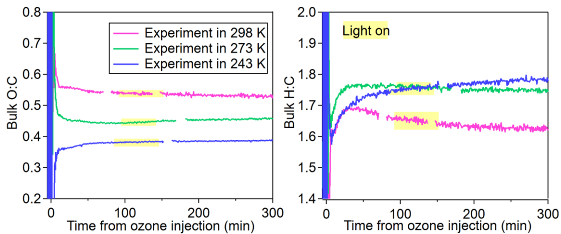
Figure S9. Timeseries of O:C and H:C values of bulk particles measured by HR-AMS during illumination period.
