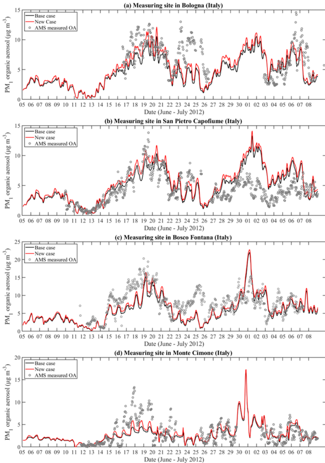
Figure S14. Ground level hourly concentrations of PM 1 organic aerosol as predicted by the Base case and the New case compared against AMS measurements taken at the 4 measuring sites. From top to bottom: Bologna, San Pietro Capofiume, Bosco Fontana, and Monte Cimone.
