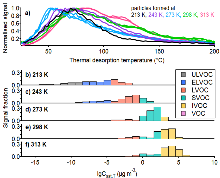
Figure S8. Thermal desorption profiles for SOA formed at different temperatures (colors) panel (a). Two profiles in the same color are from subsequent deposited particles. Volatility distributions for particles formed at 213 K (b), 243 K (c), 273 K (d), 298 K (e), 313 K (f) with C_{\text{sat},T} shifting according to the Clausius-Clapeyron relation; colors indicate different volatility groups. The ULVOC, ELVOC, LVOC, SVOC, IVOC, and VOC are identified based on the saturation concentrations as described in the method section.
