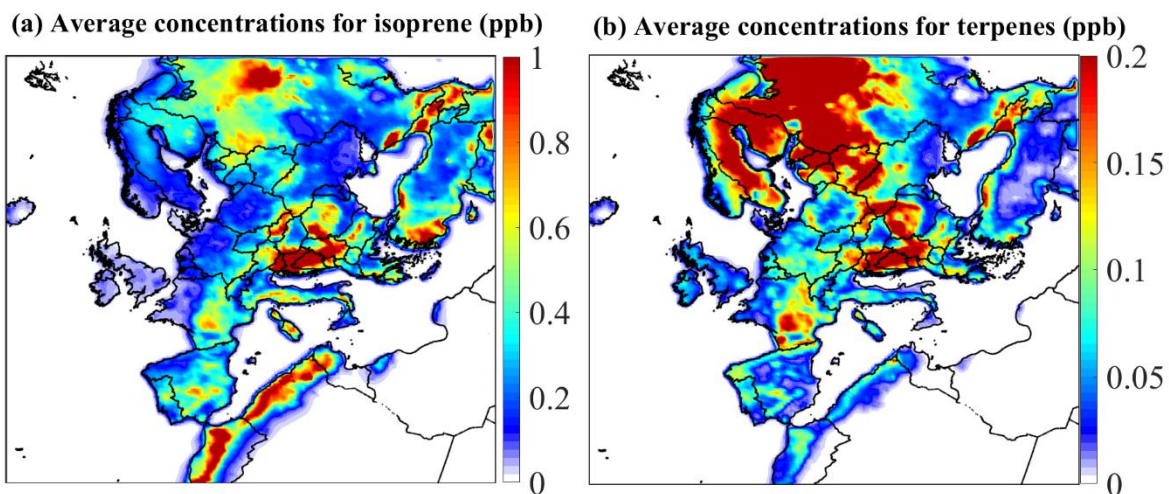
Figure S3. Monthly average concentrations of isoprene (left, in ppb) and terpene (right, in ppb) over Europe predicted by the “base case” simulation for the summer simulation period of PEGASOS 2012.
