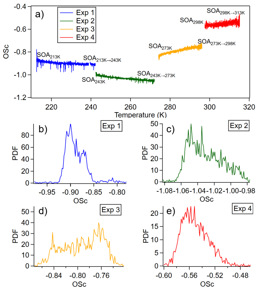
Figure S10. (a) Evolution of carbon oxidation state (OSc) across temperatures during warming periods of different experiments (Exp 1-4). (b-e) probability density function plots of OSc during each experiment (based on HR-ToF-AMS data).
