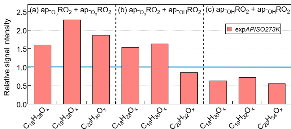
Figure S7. Relative signal intensity of \alpha -pinene dimers ( C_{18-20} ) in newly formed \alpha -pinene SOA at 273K in the presence of isoprene to the particles derived from sole \alpha -pinene oxidation (blue line). Signals are normalised to the total signal amount of a) sum of C_{18}H_{26}O_x , C_{19}H_{28}O_x , C_{20}H_{30}O_x , and b) C_{18}H_{28}O_x , C_{19}H_{30}O_x , C_{20}H_{32}O_x , and c) C_{18}H_{30}O_x , C_{19}H_{32}O_x , C_{20}H_{34}O_x .
