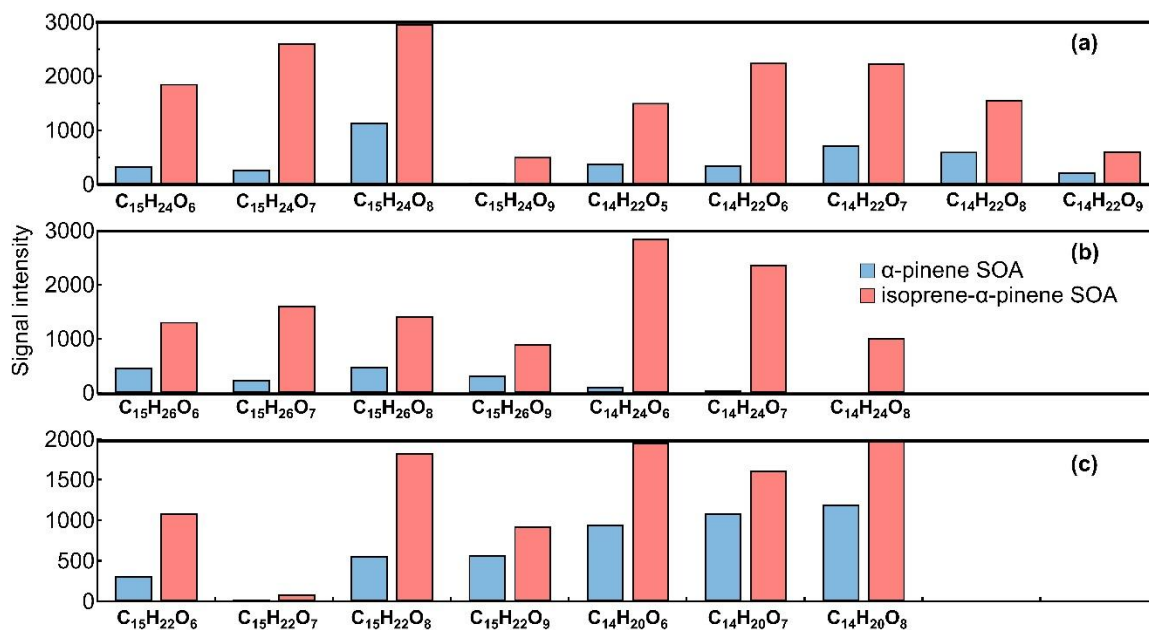
Figure S5. Comparison of C 14 -15 dimers between Exp 0 (sole α-pinene) and Exp 3 (mixture of isoprene and α-pinene) at 273 K. Blue and red bars show the compound groups in the α-pinene SOA and isoprene-α-pinene SOA, respectively. Signals are normalised to the reagent ion (I - ) to 1e6 ions. a) potentially from iso,O 3 RO 2 + ap,OHRO 2 or iso,OHRO 2 + ap,O 3 RO 2 ; b) potentially from iso,OHRO 2 + ap,OHRO 2 ; c) potentially from iso,O 3 RO 2 + ap,O 3 RO 2 .
