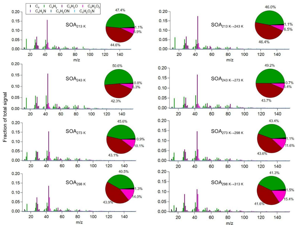
Figure S11 . Chemical composition of the fresh SOA (left) and the SOA after warming (right) measured by HR-ToF-AMS. The pie charts show the bulk chemical information, including organic-related fragments (grouped as C_x , C_xH_y^+ , C_xH_yO^+ , C_xH_yO_z^+ , C_xH_yN^+ , C_xH_yON^+ and C_xH_yO_zN^+ , where x, y, z \geq 1 ). Large portions of hydrocarbon-like (indicated by C_xH_y^+ ), less oxygenated fragments (indicated by C_xH_yO^+ ), and higher oxygenated fragments (indicated by C_xH_yO_z^+ ) are observed.
