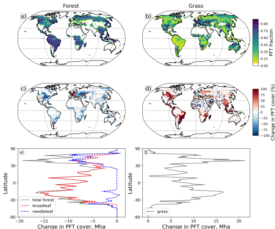
Figure 1. Distribution of the forest (left column) and grass (right column) PFTs. Panels (a) and (b) show the spatial distribution used to represent land cover for 1850. Panels (c) and (d) show the change from pre-industrial to present-day conditions (2014 – 1850) as a % of the 1850 PFT distribution. Panels (e) and (f) show the total change in forest (broadleaf and needleleaf) and grass as a function of latitude.
