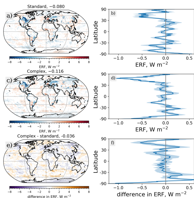
Figure 3. Net simulated TOA land use ERF ( \text{ERF}_{\text{LU}} ) in \text{W m}^{-2} for the standard chemistry mechanism (a), as well as respective zonal mean values (b). Panels (c) and (d) are the equivalent data for the complex chemistry mechanism. Values over panels (a) and (c) are the global mean ERFs. Panel (e) shows the geographical distribution of the difference in \text{ERF}_{\text{LU}} when the chemistry mechanism is changed and panel (f) shows the zonal change in \text{ERF}_{\text{LU}} . Stippling on panels (a), (c) and (e) shows differences that are significant based on Student's t -test with 95 % confidence, while shading on the zonal plots shows the standard error.
