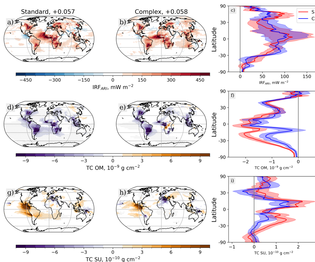
Figure 4. The role of aerosol-radiation interactions in pre-industrial to present-day land use forcing. Panels (a)–(c) show the top of atmosphere IRF from ARI associated with land cover changes for the standard (s, left column) and complex (c, middle column) chemistry mechanism, as well as the zonal mean values of IRF ARI values for both mechanisms (right column). The changes in total column organic matter (OM) mass are displayed in panels (d), (e) and (f), while panels (g), (h) and (i) show the differences in total column sulphate (SU) mass. Stippling in the left and middle columns shows regions of significant differences based on Student’s t -test with 95 % confidence, while shading on the zonal plots shows the standard error.
