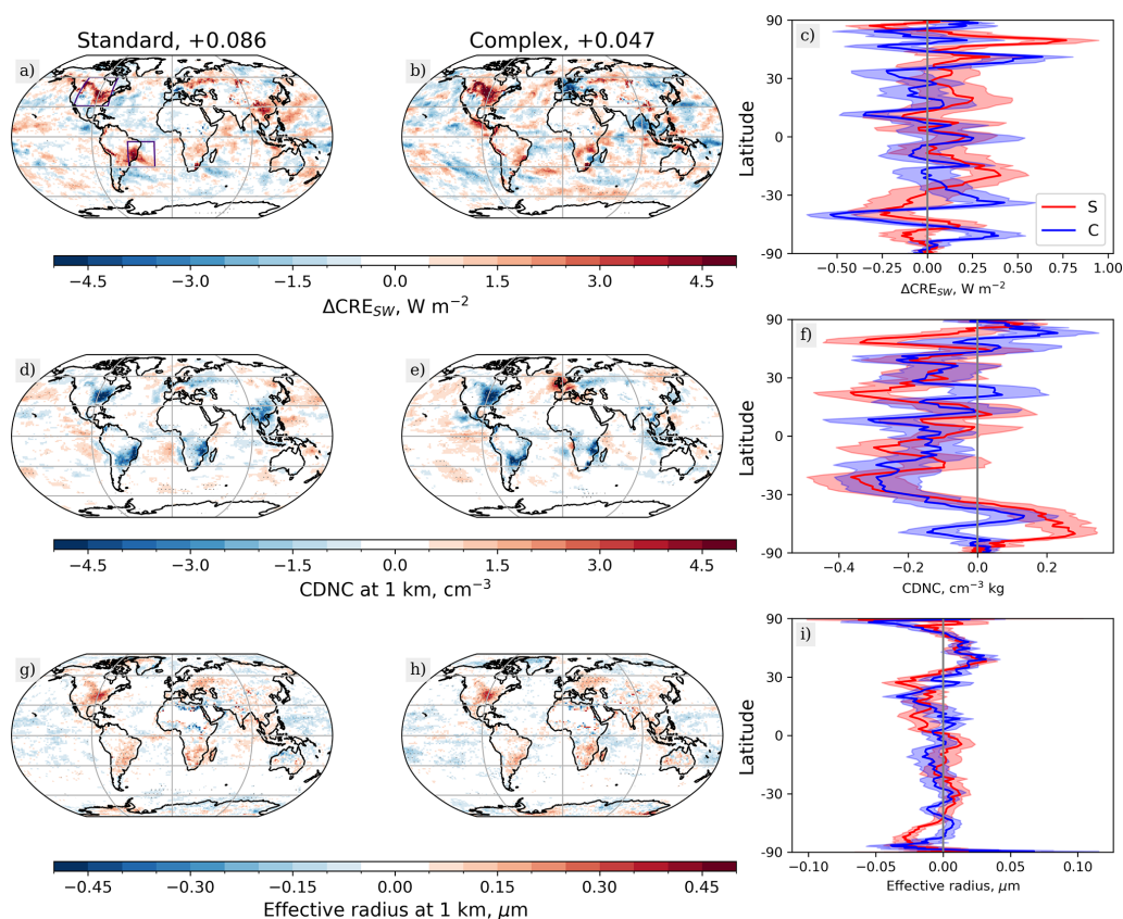
Figure 5. The role of the cloud radiative effect (CRE) in pre-industrial to present-day land use forcing. Panels (a)–(c) show changes in the top of atmosphere fluxes from \Delta\text{CRE}_{\text{SW}} associated with land cover changes for the standard (s, left column) and complex (c, middle column) chemistry mechanism, as well as the zonal mean \Delta\text{CRE}_{\text{SW}} values for both mechanisms (right column). The changes in cloud droplet number concentrations (CDNC) at 1 km altitude are displayed in panels (d), (e) and (f), while panels (g), (h) and (i) show the differences in effective radius at 1 km altitude. Stippling in the left and middle columns shows regions of significant differences based on Student's t -test with 95 % confidence, while shading on the zonal plots shows the standard error. The purple boxes on panel (a) mark regions of more substantial \Delta\text{CRE}_{\text{SW}} impacts that have been studied in additional detail.
