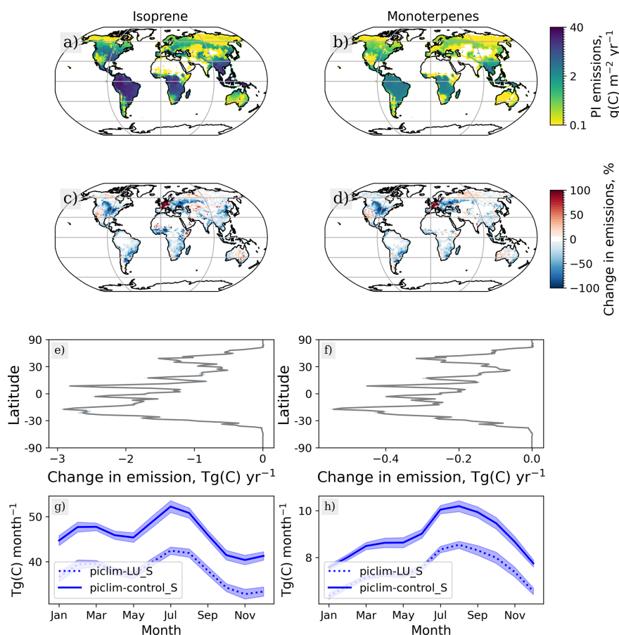
Figure 2. Land cover change impact on BVOC emissions (left column: isoprene, right column: monoterpenes). Panels (a) and (b) show the mean annual emissions of isoprene and monoterpenes for pre-industrial conditions. Panels (c) and (d) show the relative change in the respective emissions when present-day land cover is used. The absolute latitudinal differences are shown on panels (e) and (f), while the the global seasonal cycles from the piClim-control_S and piClim-LU_S experiments are displayed on panels (g) and (h).
