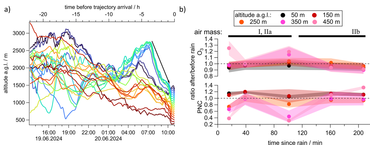
Figure 4. (a) 24 h-backward trajectories colored by arrival height show a strong downdraft within 4 h before the rain event. (b) The ratios of the \text{O}_3 mixing ratios (top) and the particle number concentrations PNC (bottom) measured at five different times after the rain to those measured before the rainfall (at 11:00) were calculated for different altitude increments (color-scale). Error bars represent the combined standard error of flights before and after the rain. Attributed air masses that are identified within a flight are indicated at the top of the graph.
