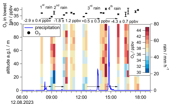
Figure 11. The vertically resolved \text{O}_3 -time series (15 min-time increments with 10 m increments altitude resolution, color-coded, measured with FLab) shows a decrease of 3.0 \pm 1.3 ppbv \text{O}_3 at the lowest bin (top panel) after rain events (blue, 60 s data) and a slow increase as \text{O}_3 -rich air is injected from higher levels.
