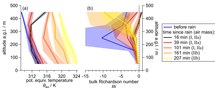
Figure 3. The gradient of the equivalent potential temperature d\theta_{\text{eq}}/dz (a) indicates unstable conditions throughout the day below 300 m, while the air mass above 300 m is stabilized after the rain at 11:00. The bulk Richardson number Ri (b) is consistent with a successive destabilization after the rain and indicates a stratification between 200 and 300 m before the rain. The solid traces show the median and the shaded area is the interquartile range of the binned data. Dashed lines indicate Ri = 0 and Ri = 0.25 .
