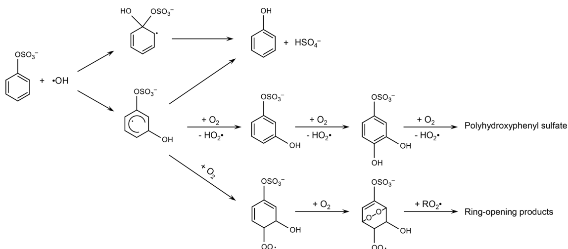
Figure 2. Scheme for the mechanism of phenyl sulfate reacting with \cdot\text{OH} .
