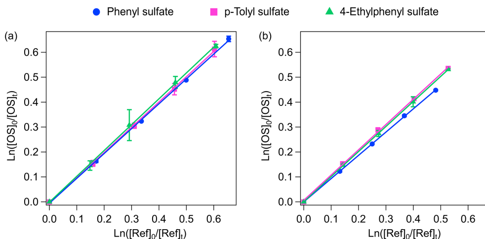
Figure 1. Loss of aromatic OSs and BA during the process of the liquid-phase \bullet\text{OH} oxidation at (a) pH 3 and (b) pH 8.
