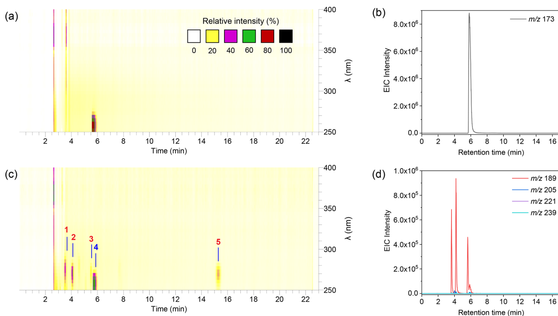
Figure 3. UPLC-PAD-MS chromatograms of samples collected (a) before and (c) after the liquid-phase \bullet\text{OH} oxidation of phenyl sulfate at pH 3. The y axis and color map represent the wavelength and corresponding UV-vis absorbance, respectively. Extracted ion chromatograms (EIC) of (b) phenyl sulfate and (d) the compositions of chromophores.
