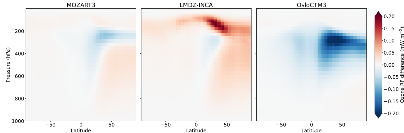
b) SSP3 Ems (SSP1BG - SSP3BG): Ozone RF
