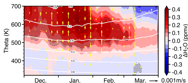
Figure 9. Differences in \text{H}_2\text{O} (shading) and vertical component of BD circulation (yellow arrows) over the Arctic between the WQBO and EQBO phases from SLIMCAT simulations for the period 1979–2022. The white contours are the climatological concentration of the \text{H}_2\text{O} . Black dotted regions indicate the differences in \text{H}_2\text{O} are statistically significant at the 95 % confidence level according to the Student's t -test.
