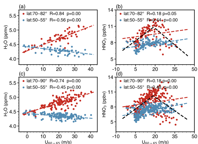
Figure 10. Relationship between (a, c) \text{H}_2\text{O} and (b, d) \text{HNO}_3 and the zonal mean wind between 60 and 65° N on the 500 K isentropic level. Data from (a, b) MLS observations (2004–2022) and (c, d) SLIMCAT simulation (1979–2022) for the period (a, c) December to February and (b, d) September to February. Red represents high-latitude regions (MLS: 70–82° N, SLIMCAT: 70–90° N), and blue represents mid-latitude regions (50–55° N). Dashed lines represent linear fits, with R denoting the correlation coefficient. The black dashed line provides a segmented fit before and after 20 \text{ m s}^{-1} at high latitudes. Values of p < 0.05 are considered statistically significant.
