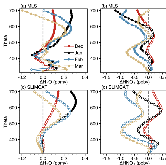
Figure 8. Differences in \text{H}_2\text{O} and \text{HNO}_3 averaged over 60–82° N between the WQBO and EQBO phases from (a, b) MLS observations and (c, d) SLIMCAT simulations for the period 2004–2021. Solid filled symbols indicate the differences are statistically significant at the 95 % confidence level according to the Student's t -test.
