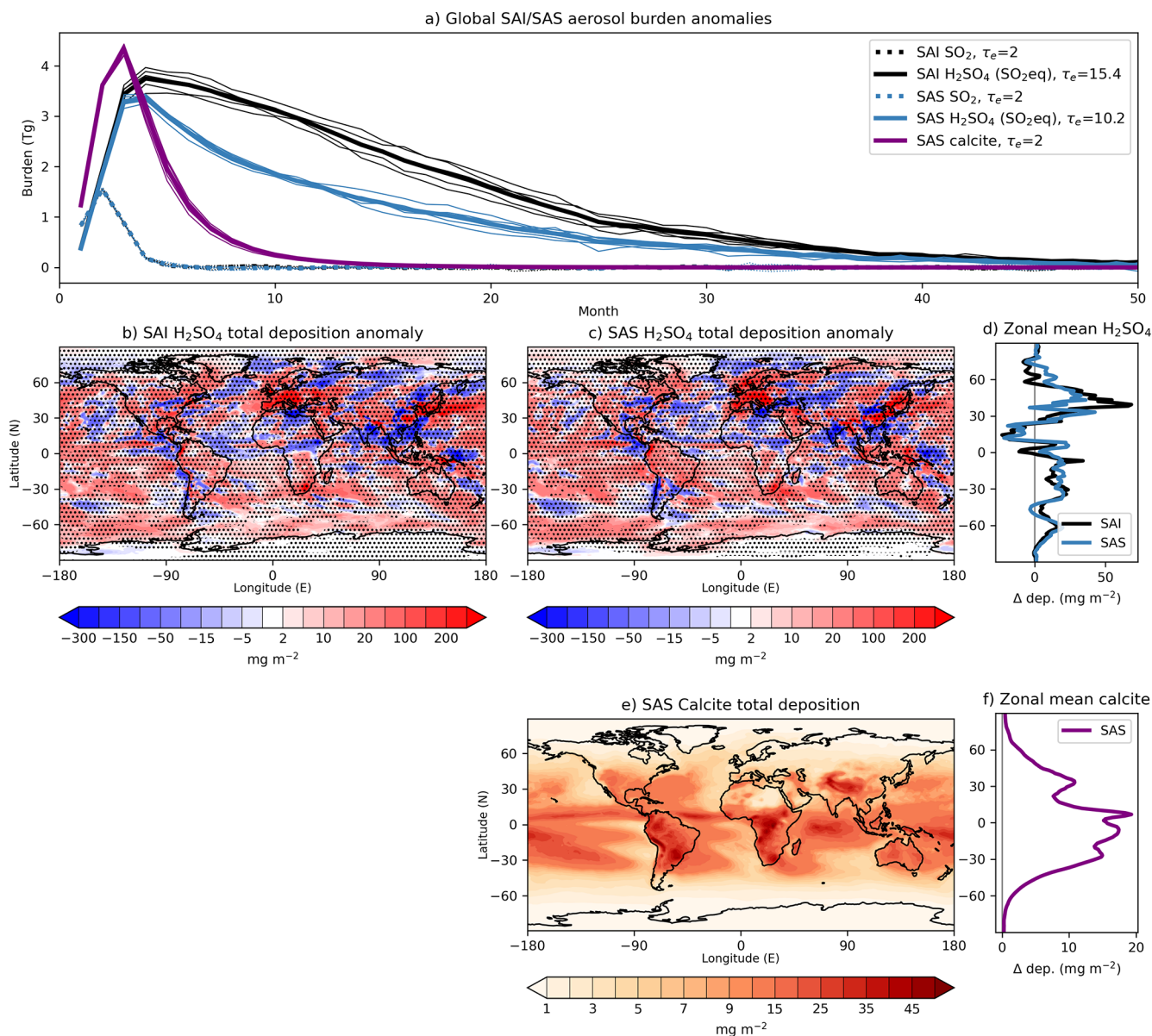
Figure 4. (a) Global \text{SO}_2 , \text{H}_2\text{SO}_4 , and calcite atmospheric burden anomalies in SAI and SAS. (b, c) Accumulated \text{H}_2\text{SO}_4 deposition anomaly in the SAI and SAS simulations relative to the control and (d) zonal means. (e) Accumulated calcite deposition anomaly in SAS and (f) zonal mean. Hatching indicates where differences are insignificant at the 5% level using a paired t -test.
