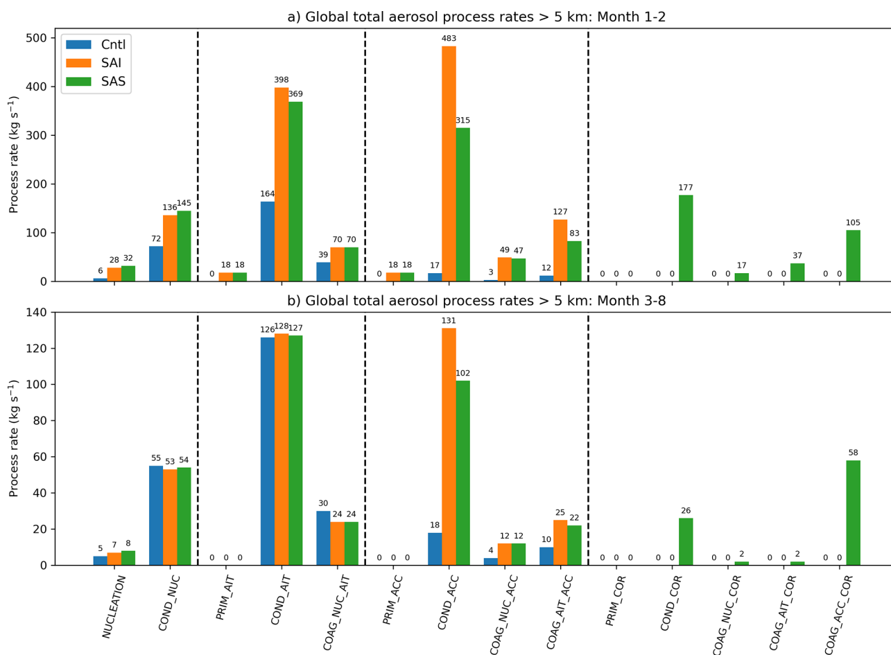
Figure 5. Total aerosol process rates for (a) during SAI/SAS deployment (months 1–2), and (b) the 6 months after deployment (months 3–8) in the Control, SAI, and SAS simulations. Quantities are integrated above 5 km altitude. We neglect intra-mode coagulation which will also contribute to aerosol growth.
