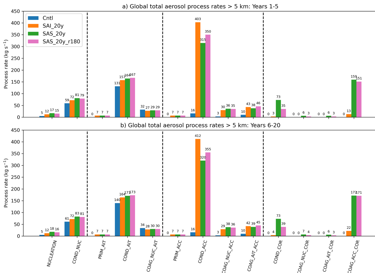
Figure 9. Total aerosol process rates in part 2 simulations for (a) during the spin-up period (Years 1–5), and (b) the equilibrium period (years 6–20) in the Control, SAI_20y, SAS_20y and SAS_20y_r180 simulations. Quantities are integrated above 5 km altitude.
