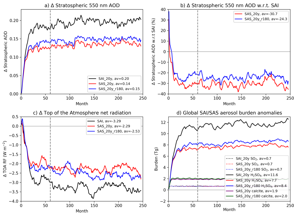
Figure 6. Global-mean anomalies in the Part 2, 20y simulations: (a) sAOD anomaly with respect to Control; (b) sAOD anomaly in the SAS simulations with respect to SAI; (c) Top Of the Atmosphere (TOA) net radiation anomaly; and (d) SO 2 , H 2 SO 4 (SO 2 eq) and calcite burden anomalies. The ToA_RF anomalies in (c) are smoothed by a 12-month running mean.
