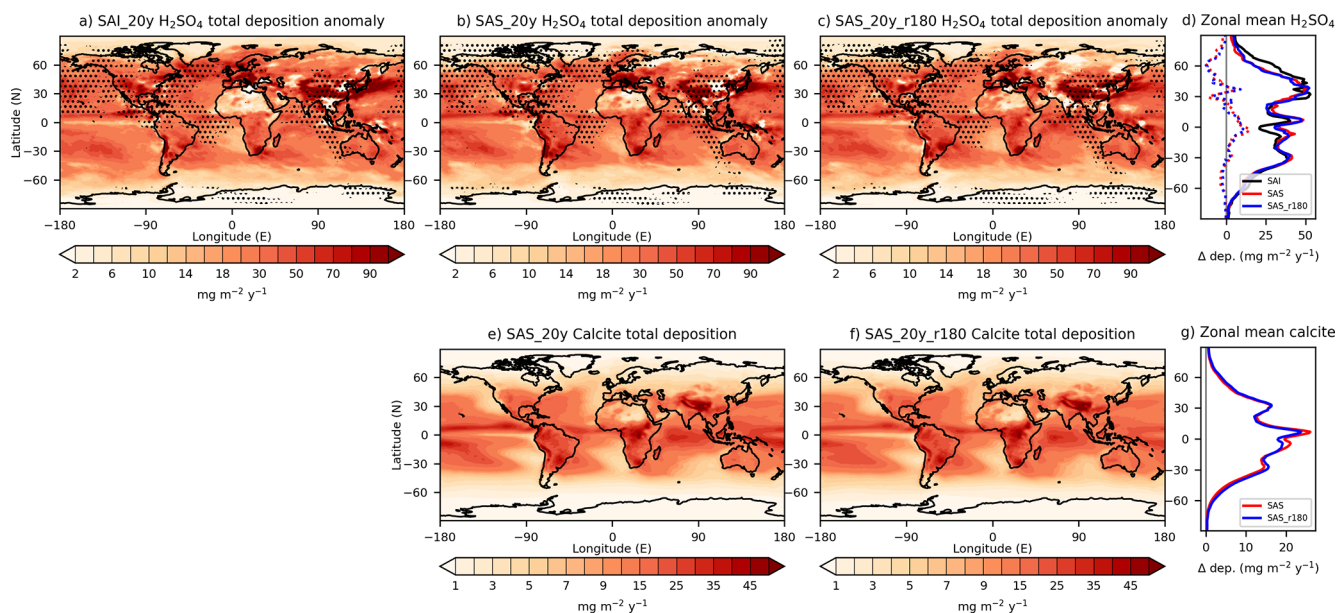
Figure 8. (a, b, c, e, f) Regional \text{H}_2\text{SO}_4 and calcite deposition rate anomalies in the Part 2 simulations for the last 15 simulated years and (d, g) zonal means. The dashed lines in Fig. 9d indicate SAS anomalies with respect to SAI. Hatching indicates where differences are insignificant at the 5% level using a pooled t -test.
