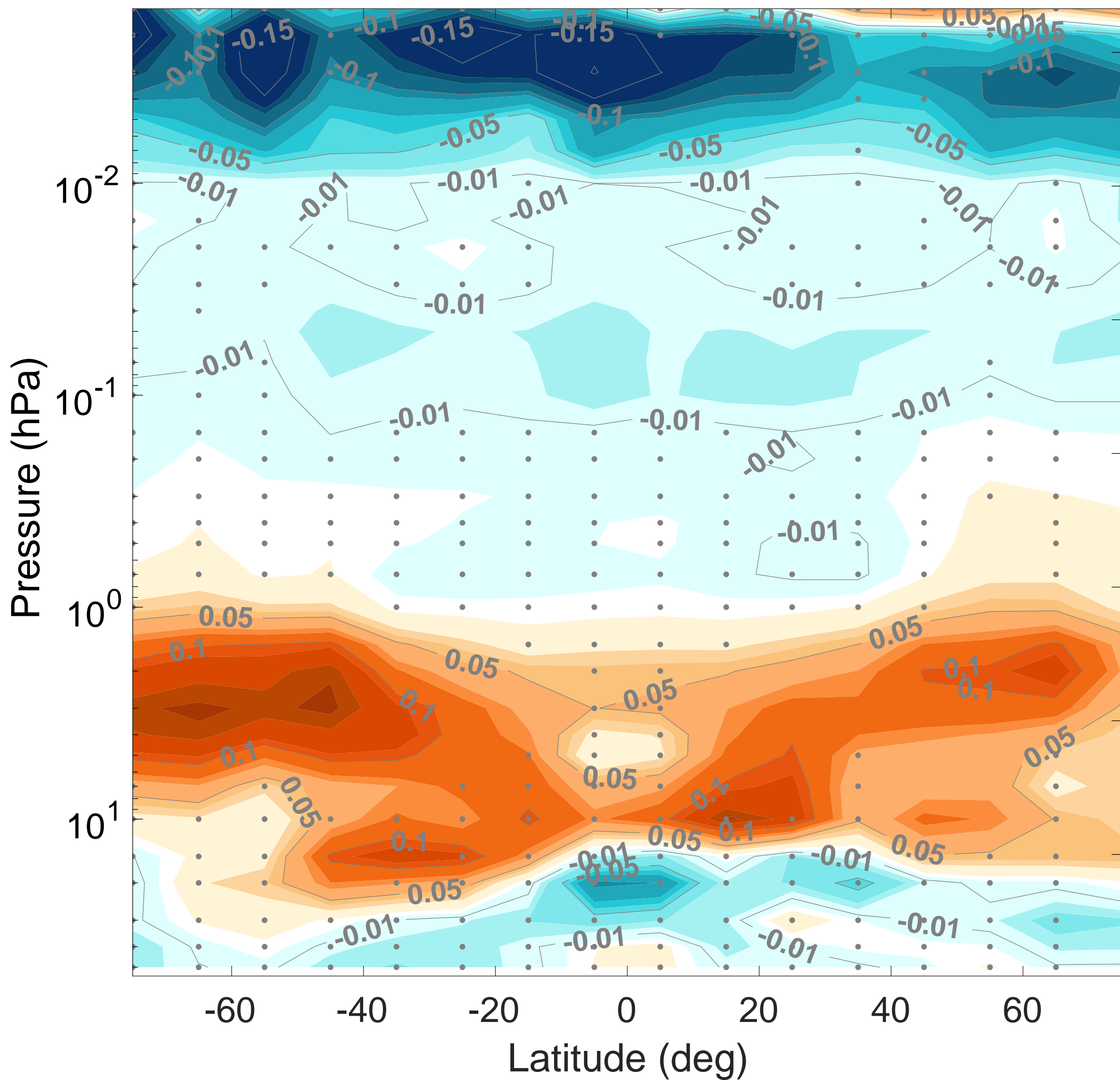
2004-2023, nighttime
