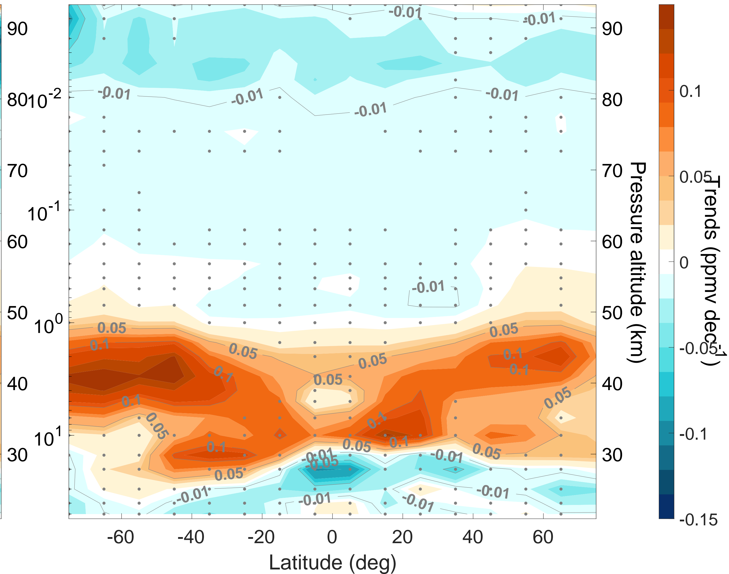
2004-2023, daytime
