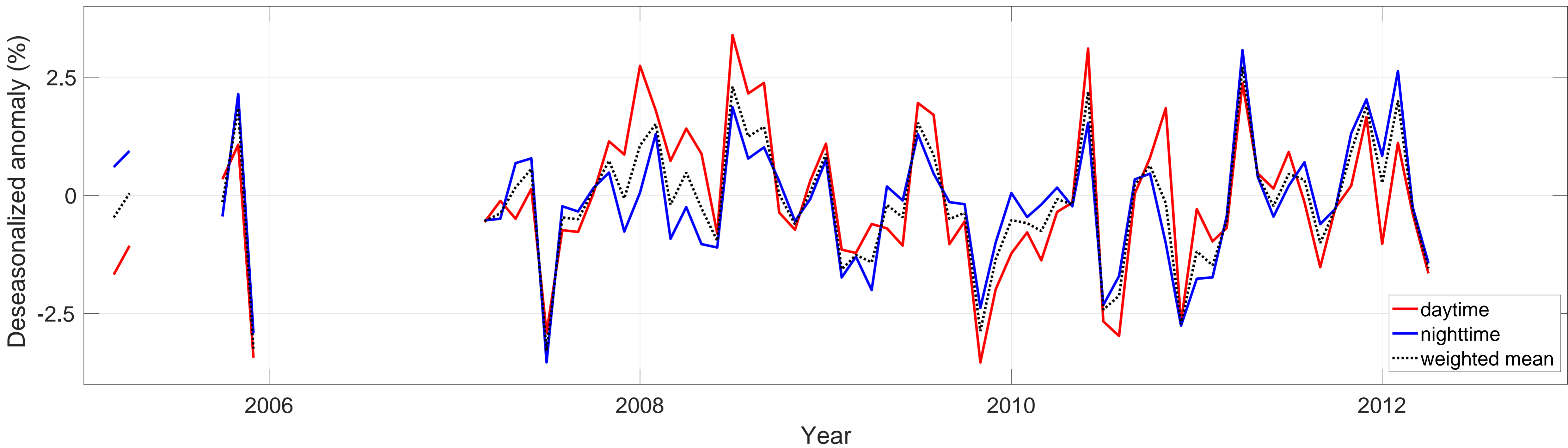
Deseasonalized anomalies, %
