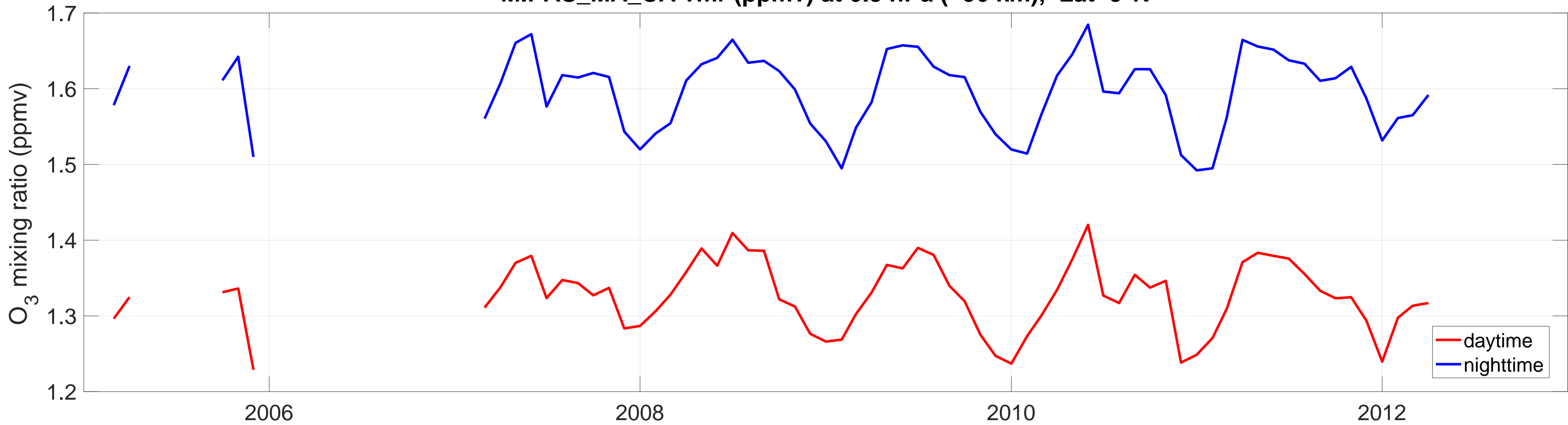
MIPAS_MA_UA vmr (ppmv) at 0.3 hPa (~56 km), Lat=5°N
