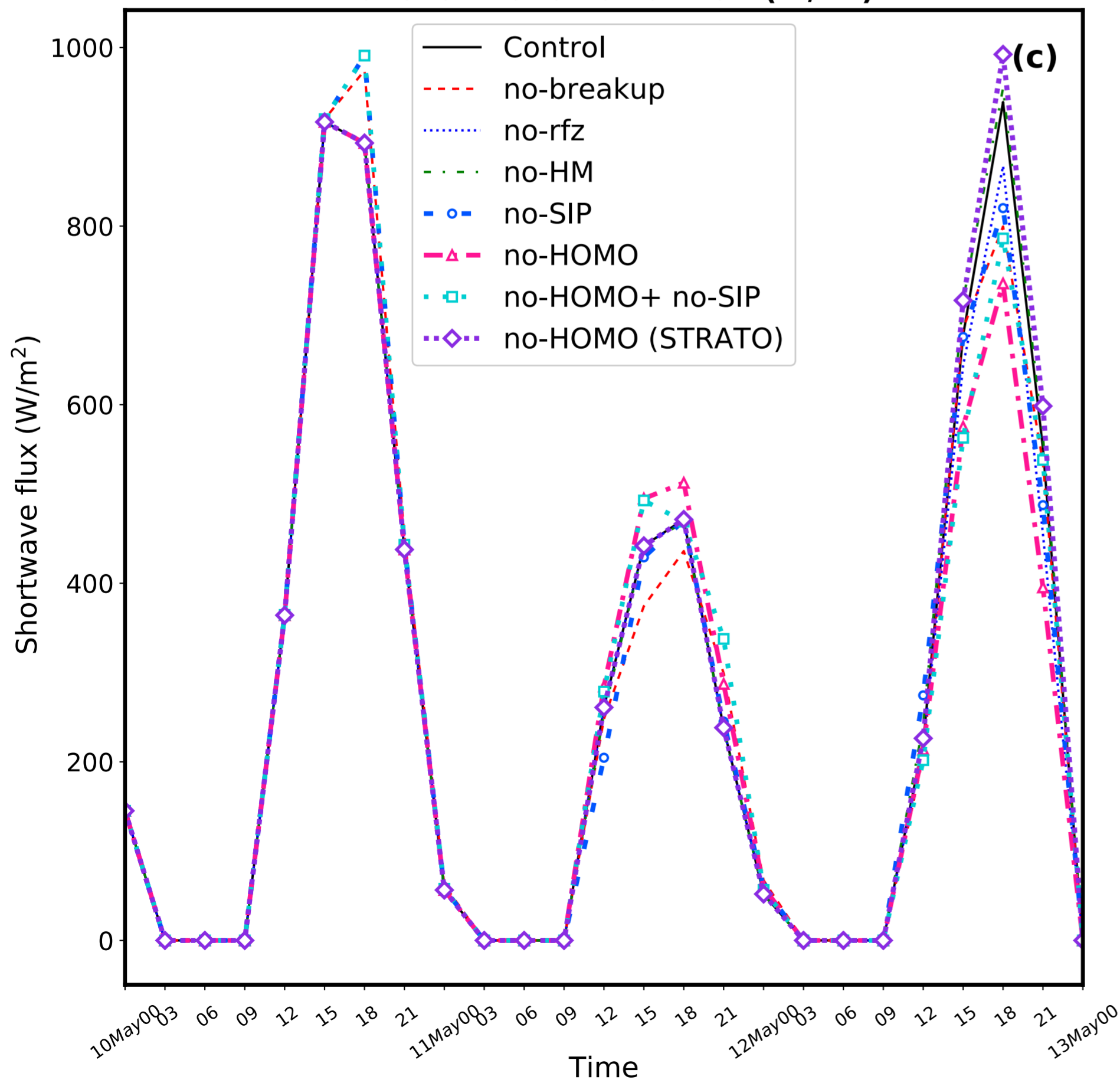
Net shortwave flux at TOA ( W/m^2 )
