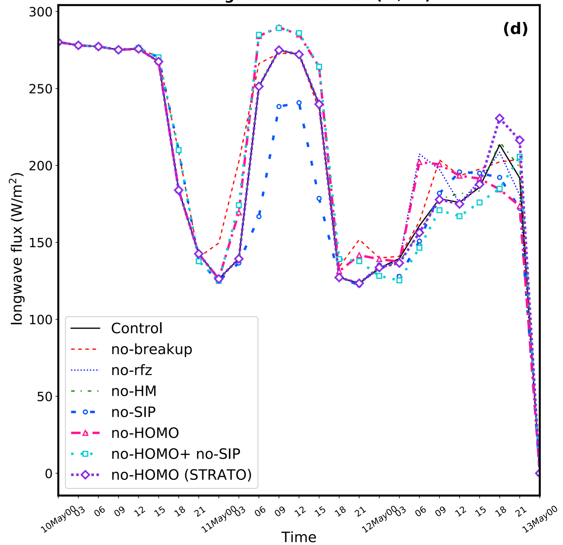
Net longwave flux at TOA ( W/m^2 )
