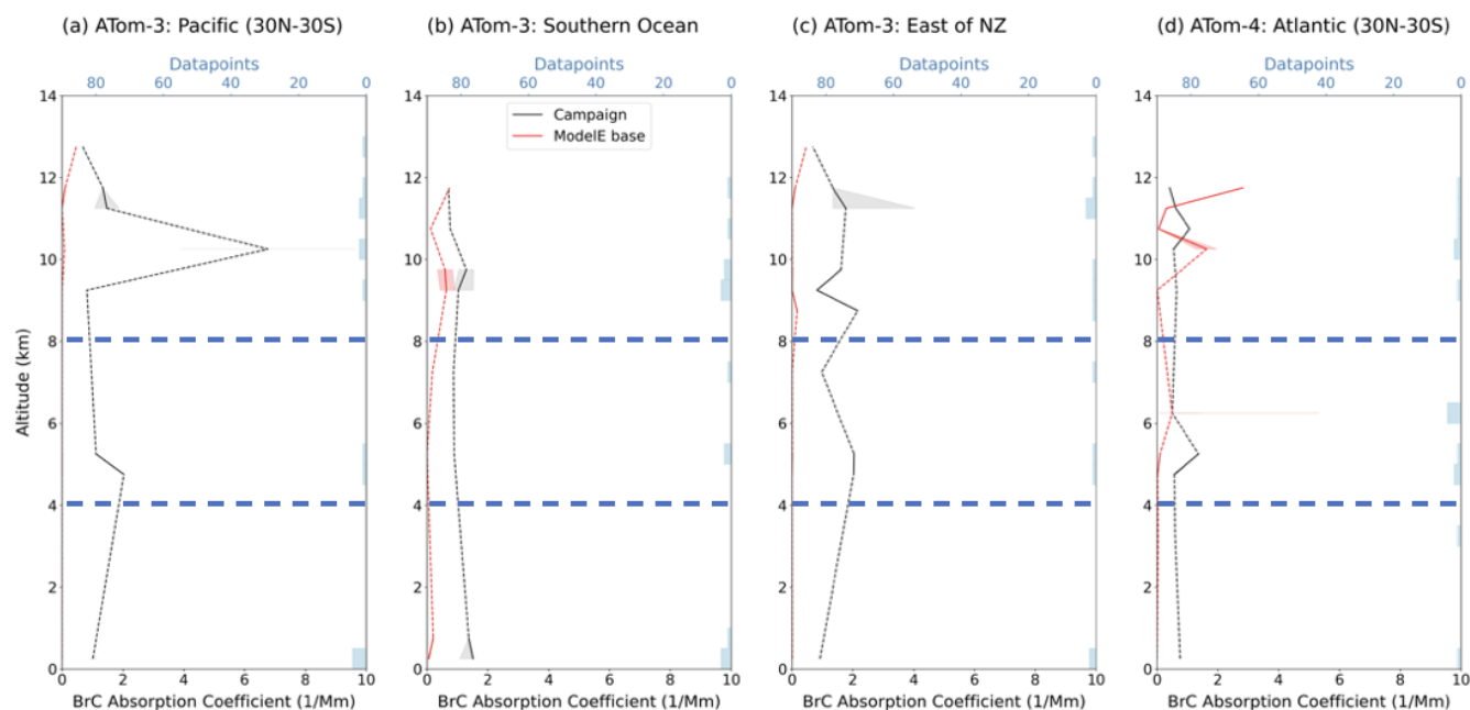
Figure 7. Vertical profiles of median BrC absorption (BrC-Abs) at 365 nm, measured by flight campaigns (black) and simulated by (red), in remote regions, reported in units of \text{Mm}^{-1} . Consistent with Fig. 6, a CO and BC scaling factor (Eqs. 1–2) have been applied to model data, campaign and specific region of analysis is indicated on the top left of each plot, the midpoint of each altitude bin is plotted, dashed lines interpolate over altitudes with no data, shaded areas show the IQR of BrC-Abs in each altitude bin, blue bars show the number of datapoints grouped in each bin, and horizontal blue dashed-lines separate the lower-, mid-, and upper-troposphere. Data is not filtered for BB number fraction.
