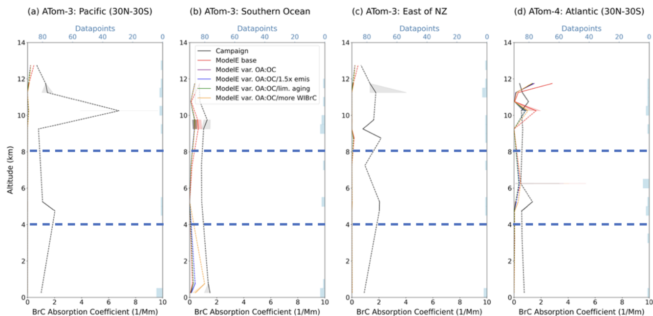
Figure 11. Vertical profiles of median BrC absorption (BrC-Abs) at 365 nm, measured by flight campaigns (black) and simulated by ModelE's base case of BrC representation (red), variable OA-to-OC ratio case (purple), 1.5 times BB OA emissions case (blue), limited aging case (green), and larger fraction of WIBRC case (orange). Analysis is over remote regions, and data is in units of \text{Mm}^{-1} . Consistent with Fig. 7, a CO and BC scaling factor (Eqs. 1–2) have been applied to model data, campaign and specific region of analysis is indicated on the top left of each plot, the midpoint of altitude bins is plotted, dashed lines interpolate over altitudes with no data, shaded areas show the IQR of BrC-Abs in each altitude bin, blue bars show the number of datapoints averaged in each bin, and horizontal blue dashed-lines separate the lower-, mid-, and upper-troposphere. Data is not filtered for BB number fraction.
