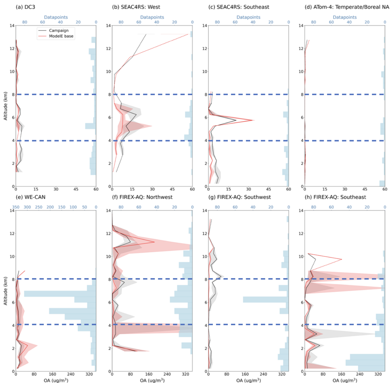
Figure A4. Vertical profiles of median, total organic aerosol (OA) concentration measured by flight campaigns (black) and simulated by ModelE's base case of BrC representation (red), over land/near sources, reported in units of \mu\text{g m}^{-3} . Model data has been multiplied by a CO and BC scaling factor (Eqs. 1–2). Consistent with Fig. A2, campaign and specific region of analysis is indicated on the top left of each plot, the midpoint of altitude bins is plotted, dashed lines interpolate over altitudes with no data, shaded areas show the IQR of data in each altitude bin, blue bars show the number of datapoints grouped in each bin, horizontal blue dashed-lines separate the lower-, mid-, and upper-troposphere, and data is filtered for BB number fraction (when relevant).
