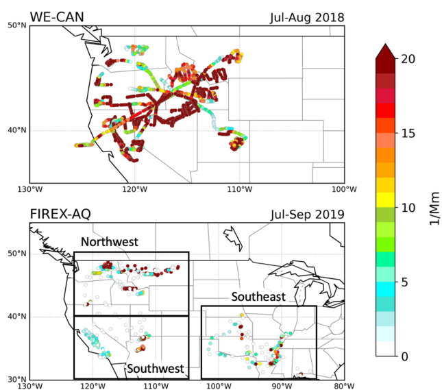
Figure 2. Map of BrC absorption coefficient measurements, at 365 nm, collected during the WE-CAN and FIREX-AQ flight campaigns. WE-CAN ambient absorption is calculated from online WS absorption measurements, while FIREX-AQ ambient absorption is calculated from water soluble (WS) and, if available, methanol-soluble filter measurements above the reported limit of detection. Regions identified for analysis are shown in black boxes and labelled.
