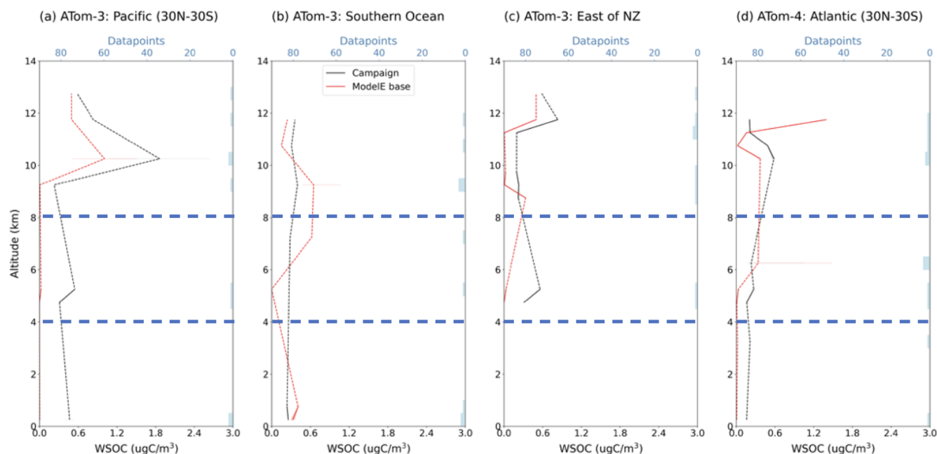
Figure A7. Vertical profiles of median water-soluble organic carbon (WSOC) concentration measured by flight campaigns (black) and simulated by ModelE’s base case of BrC representation (red), over remote regions, reported in units of \mu\text{gC m}^{-3} . Consistent with Fig. A4, a CO and BC scaling factor (Eqs. 1–2) have been applied to model data, campaign and specific region of analysis is indicated on the top left of each plot, the midpoint of altitude bins is plotted, dashed lines interpolate over altitudes with no data, shaded areas show the IQR of data in each altitude bin, blue bars show the number of datapoints grouped in each bin, and horizontal blue dashed-lines separate the lower-, mid-, and upper-troposphere. Data is not filtered for BB number fraction.
