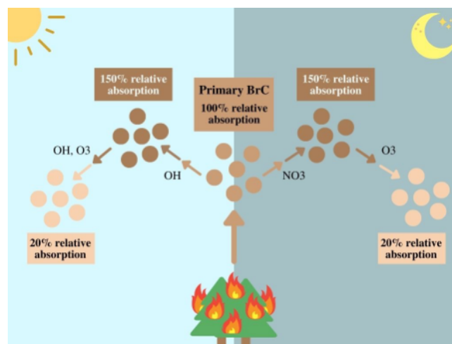
Figure A1. Chemical aging scheme of primary BrC in GISS ModelE. The large arrow represents emission of BrC mass from BB, while smaller arrows represent mass transfer between BrC types. Reproduced from DeLessio et al. (2024), Fig. 3.
