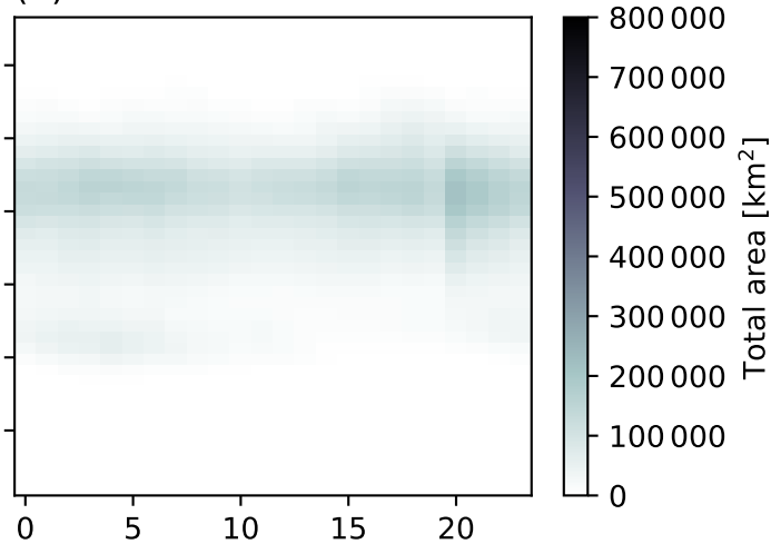
(e) non-ice-producing updrafts
