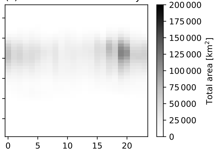
(c) ice clouds detected only
