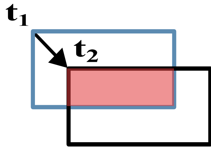
(a) Overlap > 0.5 ?
