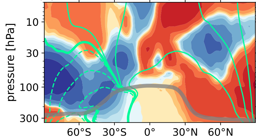
(e) net tendency \times 10
