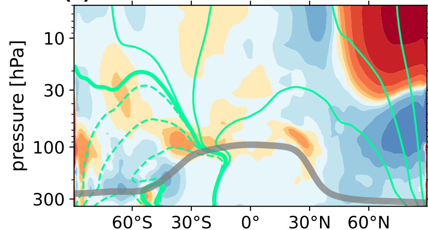
(e) net tendency \times 10
