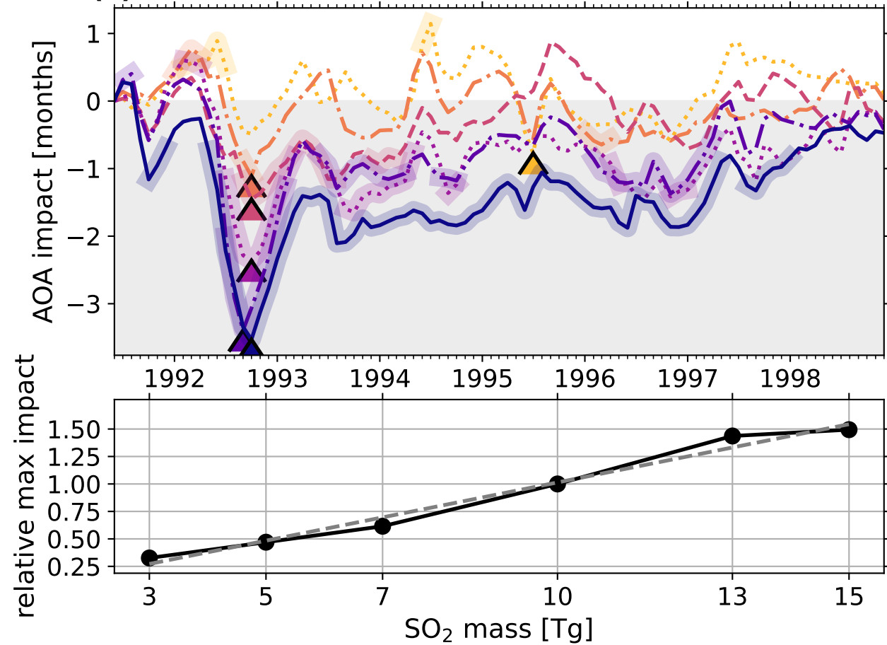
(c) 20S–40S, 30 hPa
