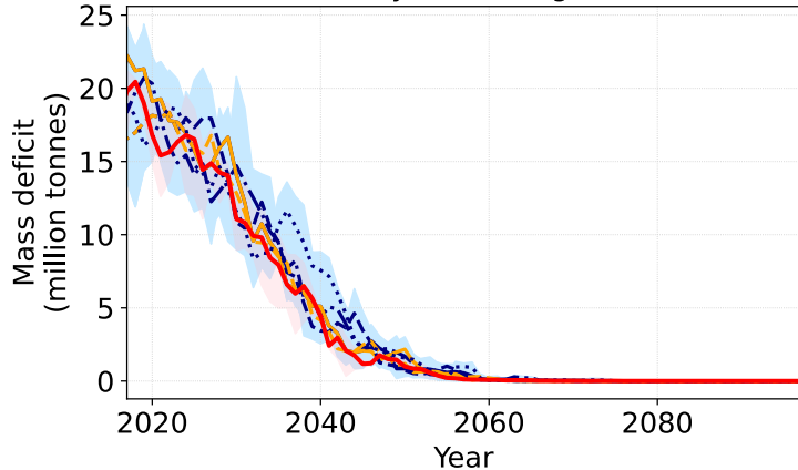
October-mean ozone mass deficit (< 220 DU) over Antarctica (3-year moving mean)
