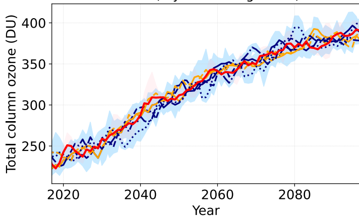
October-mean total column ozone over Antarctica (3-year moving mean)
