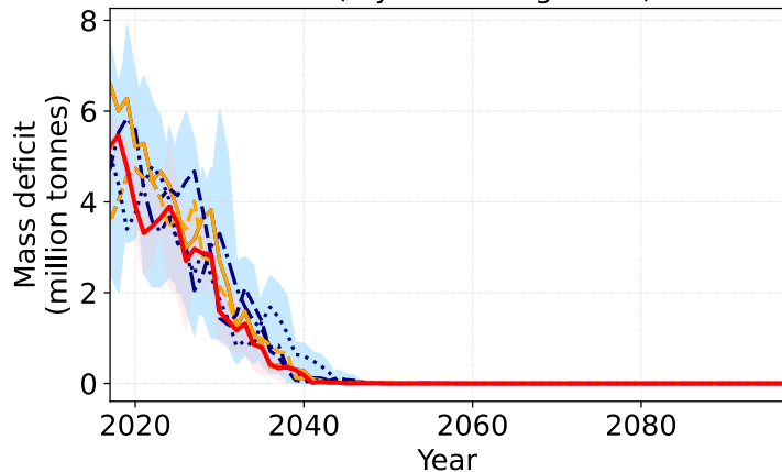
October-mean ozone mass deficit (< 175 DU) over Antarctica (3-year moving mean)
