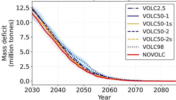
October-mean ozone mass deficit (< 220 DU) over Antarctica (30-year moving mean)
