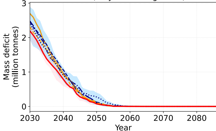
October-mean ozone mass deficit (< 175 DU) over Antarctica (30-year moving mean)
