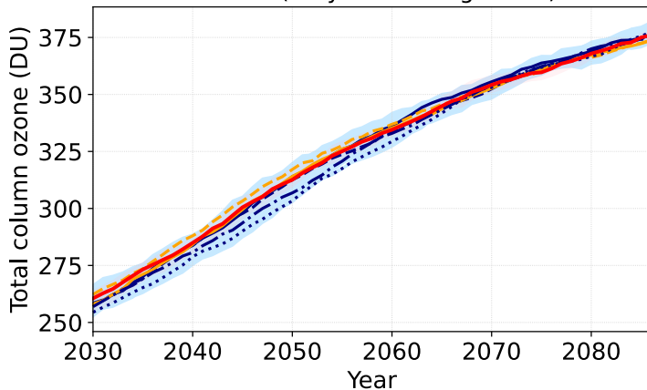
October-mean total column ozone over Antarctica (30-year moving mean)
